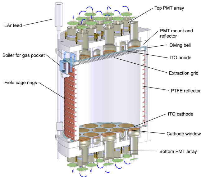
FIG. 1. The DarkSide-50 TPC. Reproduced from [4] under [6].
