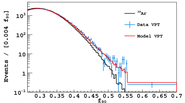
FIG. 8. f_{90} for events with 100 < S1 < 180 PE comparing single-scatter ER data ( ^{39}\text{Ar} ), VPT data passing all major cuts, notably S1pMaxFrac, and simulated VPT events using the f_{90} model including Cherenkov light. The normalization of the simulation is absolute, using the activities in Table I and the 532.4 live-days exposure.
