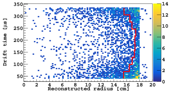
FIG. 5. Radial cut (red) shown on events in the initial blinding box shown in Fig. 4. All event quality cuts (Sec. VA 1), all basic cuts (Sec. VA 2) through MinS2uncorr, and vertical fiducialization via t_{\text{drift}} have been applied.
