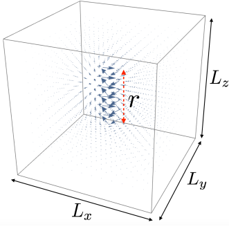
FIG. 4. The background field \mathcal{A}^{Q\bar{Q}} from monopole-antimonopole pair (the blue arrows) in a periodic L_x \times L_y \times L_z lattice box. The distance between monopole and anti-monopole is r , and they are separated along the z -direction.
