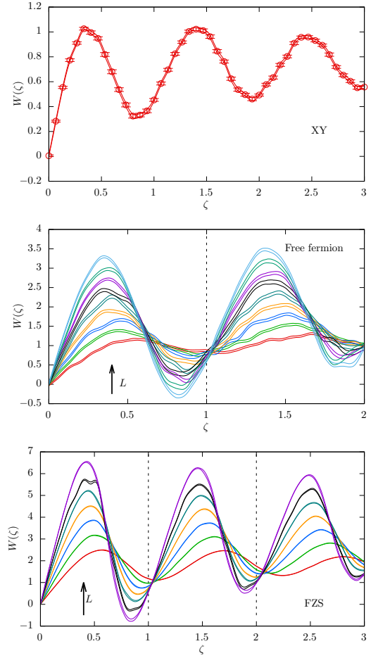
FIG. 5. Top panel shows W(\zeta) for the critical XY model at r/L = 1/4 on L = 20 lattice. The measurements of W(\zeta) are the red circles, while the red band is the 1\text{-}\sigma error band from the cubic spline interpolation. The middle panel shows W(\zeta) for free Wilson-Dirac fermion and the bottom one for the critical FZS model. The different color bands correspond to different L at fixed r/L = 1/4 . Along the direction of the arrow, the values of L for free fermion are L = 12, 16, 20, 24, 28, 32, 36, 40, 44 respectively. For the FZS model, it is L = 12, 16, 20, 24, 28, 32, 36 respectively.
