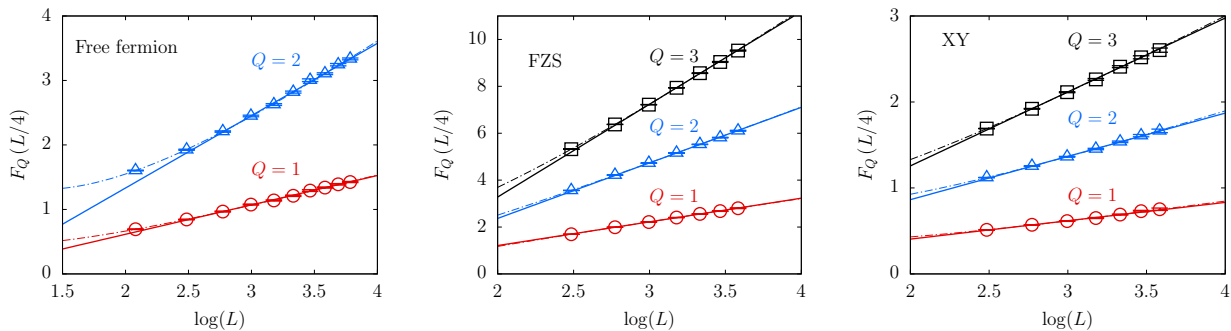
FIG. 2. The free energy of monopole-antimonopole background field insertion is shown as a function of \log(L) for fixed \rho = r/L = 1/4 . The left panel is for free Wilson-Dirac fermion, the middle panel for the critical frozen superconductor model and the right panel for the critical XY model. The curves are fits to the data.
