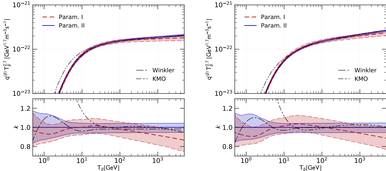
FIG. 8. CR p\text{He} (left panel) and \text{He}p (right panel) antiproton source term with the uncertainty on cross sections for the best fit of Param. I-B and II-B, i.e. with NA49 pC and LHCb p\text{He} data. Uncertainties are given at the 2\sigma confidence interval.
