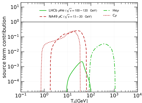
FIG. 3. Similar to Fig. 1, but for the nuclear channel. Fraction of the antiproton source term originating from the kinematic parameter space of the cross section which is experimentally determined by NA49 p\text{C} and LHCb p\text{He} data. Specifically, we assume a range of \sqrt{s} = 15\text{-}20 GeV for NA49 and 100\text{-}120 GeV for LHCb. Each contribution is normalized to the total source term of the specific channel.
