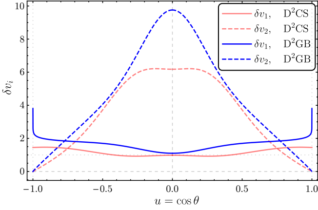
FIG. 1. (Color online) The metric deformation functions \delta v_1 (solid) and \delta v_2 (dashed) as functions of u , for both dCS-deformed (red) and EdGB-deformed (blue) NHEK. Note that in D 2 GB, \delta v_1 blows up at the two poles u = \pm 1 .
