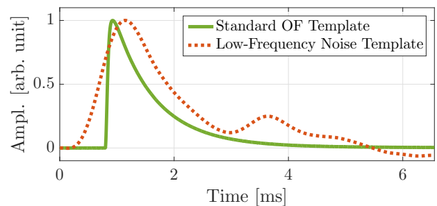
Figure 14. Template traces for the standard OF (green solid) and low-frequency noise (orange dotted) fits. The templates were generated by averaging many events’ pulse shapes, which removes uncorrelated noise. Details of the low-frequency noise template generation are discussed in the text and the standard OF template definition is discussed in Sec. II C. The maxima of the amplitudes (Ampl.) are scaled to unity in the figure.
