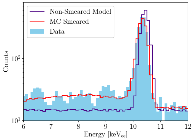
Figure 23. ^{71}\text{Ge} K -shell peak in the Run 2 data, with no fiducial-volume cut, compared to the results of the electric-field study. The study simulates peak events on top of a flat Compton background before applying a smearing function. The smeared low-energy tail observed in the data is replicated in the simulation.
