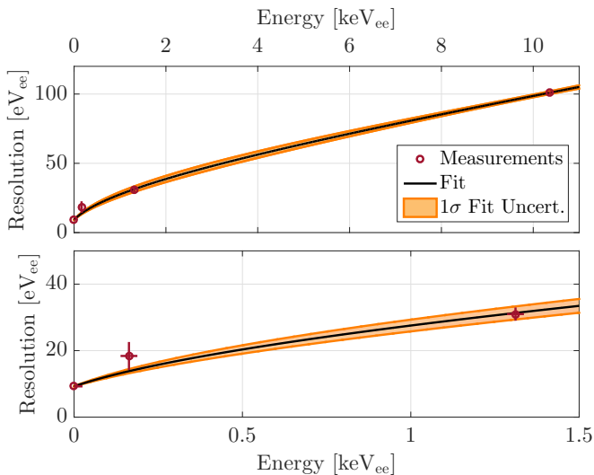
Figure 18. Width of four points in the Run 2 energy spectrum (red points), the best-fit curve (black), and 68% uncertainty band (orange). The bottom panel is an enlargement of the top panel below 1.5 keV ee .
