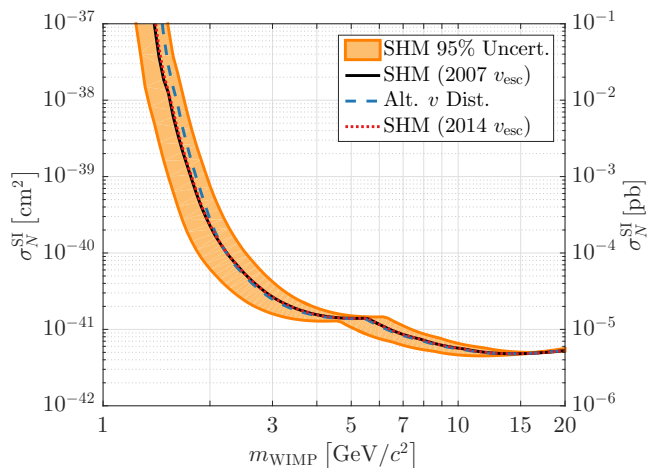
Figure 31. The 95% (orange) uncertainty band on the “best-fit” Run 2 spin-independent limit (black solid) due to the uncertainties in most probable WIMP velocity ( v_0 ) and the galactic escape velocity ( v_{\text{esc}} ) used in the SHM. The 2014 RAVE survey v_{\text{esc}} distribution is sampled and thus the best-fit curve substituting the 2014 median value into the SHM is given for consistency (red dotted). The black and red-dotted curves are the same as in Fig. 29, where an enlargement at low WIMP mass is given. The best-fit limit computed using the alternative velocity distribution of Eq. 26 is also presented (blue dashed).
