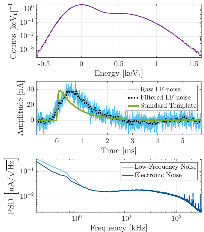
Figure 12. Top : Run 2 noise distribution. The electronic-noise distribution is centered at \sim 0 keV t while the low-frequency-noise distribution dominates from 0.5–1.5 keV t . For reference, 1 keV t \approx 66 eV ee . Middle : raw (thin light blue solid) and filtered (thick black dotted) trace from a typical low-frequency noise event compared to the standard-event template (thick green solid), derived from high-energy 71 Ge K -shell events. The difference in pulse shape is most evident between 0 and 2 ms. Bottom : power spectral densities (PSD) for 500 low-frequency (light blue) and electronic (dark blue) noise traces. The low-frequency noise population has more power below \sim 1 kHz.
