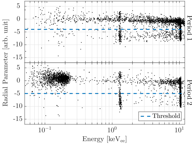
Figure 25. 2T-fit based radial parameter as a function of energy for Run 2 Period 1 (top) and Period 2 (bottom). The vertical clusters are the ^{71}\text{Ge} activation lines and the horizontal band at high radius contains reduced-amplification events. The radial cut thresholds are indicated by the blue dashed line, effectively removing events at high radius, including the low-energy cluster seen in Period 2.
