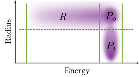
Figure 26. Diagram showing the morphology of the expected event distribution in the radial-parameter vs. reconstructed-energy plane from a mono-energetic homogeneously distributed source. The distribution is split (vertical solid lines) into non-peak events R , with reduced NTL-amplification and peak event P . The latter group is further separated into inner peak events P_i , that pass the cut threshold (horizontal dotted line), and outer peak events P_o , that do not. In practice, the ^{71}\text{Ge} activation peaks were considered, which can be separated from background because of the known half-life of the isotope.
