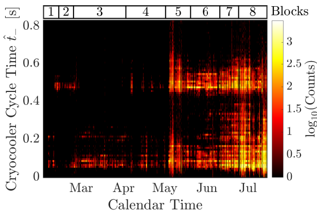
Figure 13. Number of low-energy triggered events for Run 2 Period 1 in the two-dimensional plane of cryocooler time, \hat{t}_c , and calendar time in 2014. The color scale is logarithmic with empty bins mapped to black. The rate of low-frequency noise injection evolved throughout the run because of the deterioration of the cryocooler, ranging from 0 to >1000 counts per bin. The boundaries of the eight time blocks defined after applying a smoothing filter to the histogram are given in the bar labeled “Blocks” above the plot.
