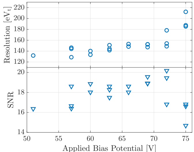
Figure 9. Baseline resolution (top) and the corresponding signal-to-noise ratio SNR (bottom) as a function of the applied bias potential. Each point represents a single 3 hr long data set taken prior to Run 2. The resolution and SNR increase and decrease, respectively, past \sim 70 V in applied bias. The average uncertainty for each point is 3.6\text{eV}_t for the resolution and 0.39 for the SNR. The additional variation seen at a given bias is likely a result of time dependence of the noise. For reference, 1\text{keV}_t \approx 66\text{eV}_{ee} .
