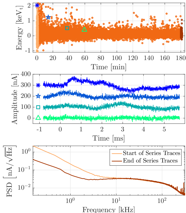
Figure 10. Top : total phonon energy, or noise, as a function of time since biasing in Run 1. The noise decays quasi-exponentially with time; four example events are given by non-circular markers. The first and last 500 traces are highlighted in light and dark orange, respectively. The noise distribution is offset from 0 \text{keV}_t as the energy-estimating algorithm tends to fit to upward noise fluctuations. For reference, 1 \text{ keV}_t \approx 66 \text{ eV}_{ee} . Middle : raw traces of the events marked in the top panel. Traces are shifted by 100 nA with respect to each other for clarity. Bottom : power spectral densities (PSD) for the noise at the start (light orange) and end (dark orange) of the series. The earlier traces have more power below \sim 10 kHz.
