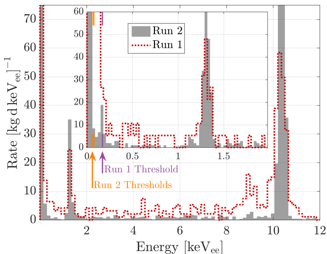
Figure 5. Measured efficiency-corrected spectra for Run 1 (red dotted curve) and Run 2 (gray shaded area). The ^{71}\text{Ge} activation peaks at 10.37 and 1.30 keV ee are prominent in both spectra and the peak at 0.16 keV ee is additionally visible in the Run 2 spectrum. The ^{65}\text{Zn} K -shell electron-capture peak is also visible at 8.89 keV ee in the Run 1 spectrum. Inset : an enlargement of the spectra below 2 keV ee with bins five times smaller and the runs' analysis thresholds given by the extended and labeled tick marks.
