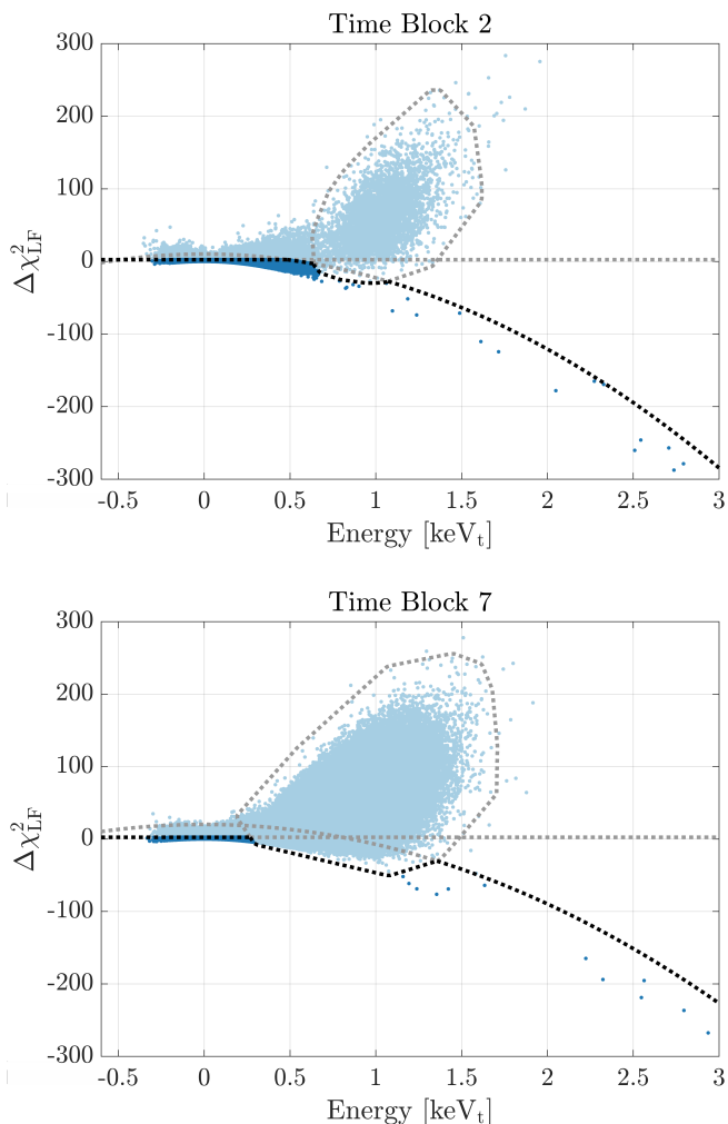
Figure 15. \Delta\chi_{\text{LF}}^2 as a function of total phonon energy for time blocks 2 (top) and 7 (bottom) showing the three portions of the low-frequency-noise rejection cut (dotted) with the defining portion at any given energy darkened. Low-frequency noise events cluster near \sim 1 keV t while good events fall on a downward opening parabola. The major difference between the two subplots is the difference in low-frequency-noise: time block 2 shows low noise, while time block 7 is more noisy. Events above any portion of the cut are rejected (light blue) while those below are retained (dark blue). Time block 2 is relatively less noisy, while time block 7 is relatively more noisy. The contour portion in block 2 cuts more loosely ( 2.5\sigma ) than in block 7 ( 5\sigma ) because of the changing low-frequency noise environment throughout the run. A pre-selection cut removing events with unusually high NSOF \chi^2 values has been applied in these figures and, for reference, 1 \text{ keV}_t \approx 66 \text{ eV}_{\text{ee}} .
