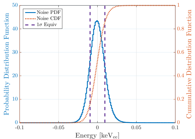
Figure 17. Reconstructed energy probability distribution function (PDF) of noise-only events in Run 2 (blue solid, left vertical axis) with the corresponding cumulative distribution function (CDF; orange dotted, right vertical axis). The 1\sigma -equivalent is taken as half the distance between the 15.87 th and 84.13 th percentiles (dark purple dashed) and is 9.26 \pm 0.11 \text{ eV}_{ee} .
