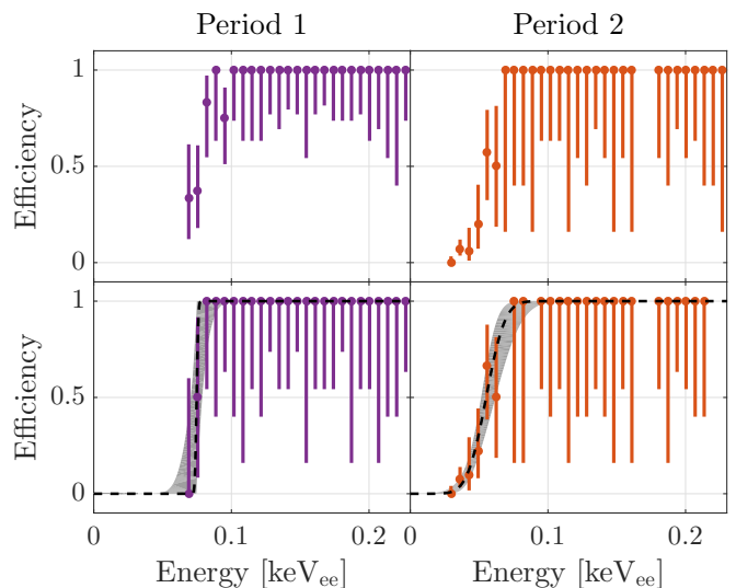
Figure 19. Binned trigger efficiency without (top) and with (bottom) a cut on cryocooler timing for Run 2 Periods 1 (left) and 2 (right). Using the cryocooler information noticeably improved the Period 1 measurement while marginally improving that for Period 2. The best-fit error function (black dashed curve) and its 68% uncertainty (grey shaded) are given in the bottom row for each period.
