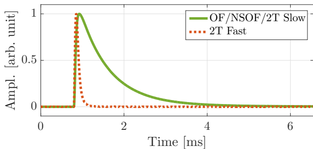
Figure 6. Templates used for the standard optimal filter (OF), non-stationary optimal filter (NSOF), and 2T-fit algorithms for CDMSlite analysis. The green solid curve is the single trace used for the OF, NSOF, and 2T-fit slow templates, which is derived from averaging high-energy traces. In the 2T fit, the slow template’s amplitude carries the main energy information. The 2T-fit fast template (orange dotted), is derived by considering the differences between the slow template and the traces used in the slow template’s derivation. In the 2T fit, the fast template’s amplitude captures the position information from the signal trace. The maxima of the amplitudes (Ampl.) are scaled to unity in the figure.
