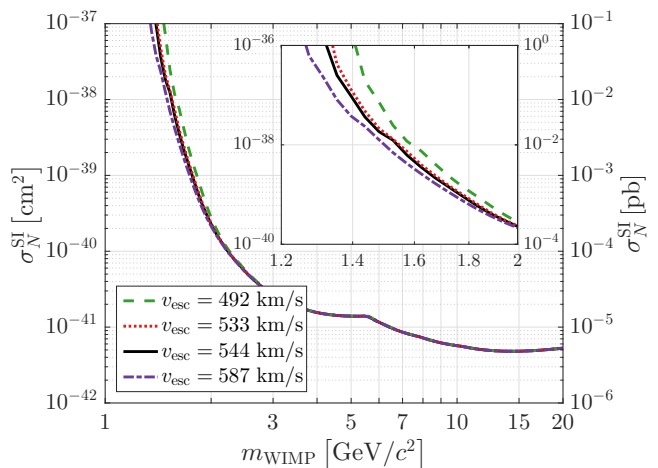
Figure 29. Effect on the Run 2 “best-fit” limit from varying the Galactic escape velocity v_{\text{esc}} in the Maxwellian halo model while keeping all other parameters constant. Curves shown are the median values of the 2007 and 2014 RAVE survey results at 544 \text{ km s}^{-1} (black solid) and 533 \text{ km s}^{-1} (red dotted) respectively as well as the 90% confidence bounds of the 2014 result at 492 \text{ km s}^{-1} (green dashed) and 587 \text{ km s}^{-1} (purple dot-dashed). The inset shows an enlargement below WIMP masses of 2 \text{ GeV}/c^2 . Varying v_{\text{esc}} changes the lowest WIMP mass that can produce recoils above threshold while the impact on the limit at higher masses is negligible.
