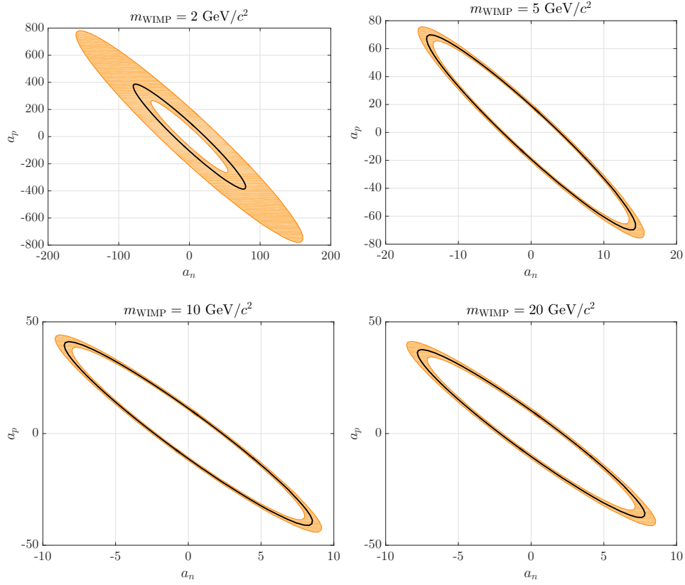
Figure 33. Median (90% C.L.) upper limit and associated 95% uncertainty (thick black solid curve surrounded and orange bands) on the WIMP-nucleon coupling coefficients a_p and a_n from CDMSlite Run 2 for WIMP masses of 2 (top left), 5 (top right), 10 (bottom left), and 20 (bottom right) \text{GeV}/c^2 . Areas outside the ellipses are excluded for each WIMP mass.
