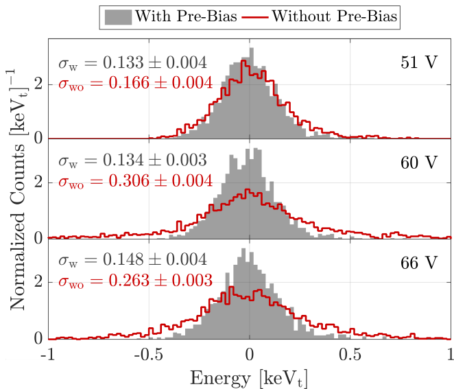
Figure 11. Baseline noise distribution for series that were pre-biased (gray area) and series that were not pre-biased (red curve) taken at potential differences of 51/60/66 V (top/middle/bottom). The Gaussian-equivalent widths (see Sec. IV A) of the distributions with \sigma_w and without \sigma_{wo} pre-biasing are also given, in keV t . The thinner distribution widths for pre-biased series compared to non-pre-biased series demonstrates the effect of pre-biasing. For reference, 1 keV t \approx 66 eV ee .
