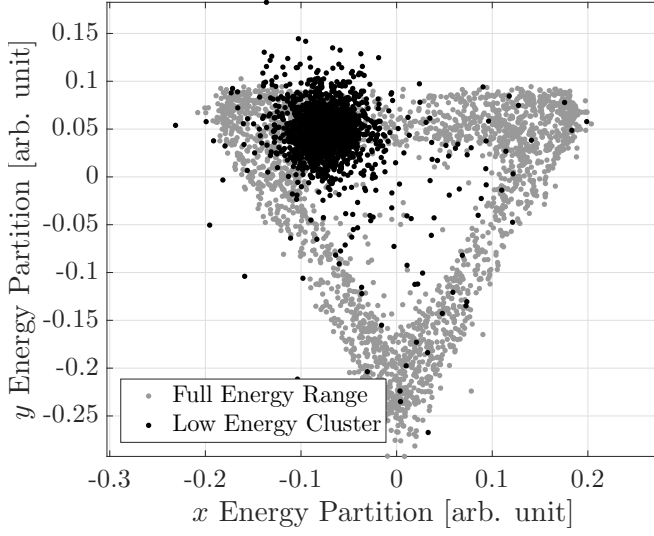
Figure 24. Position of Run 2 events using the energy partition coordinates. Events in the full energy range are gray while those between 100 and 200 eV ee are highlighted in black. The population at low energy is clearly clustered in position.
