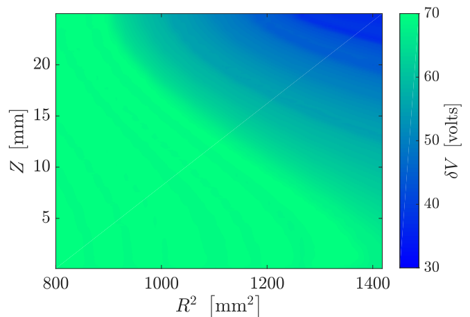
Figure 22. Difference in electric potential between the final locations of electrons and holes (color map), after propagating through the crystal, as a function of their initial position in the detector. A single vertical slice of the detector, perpendicular to the circular top and bottom faces (see Fig. 2) and along an arbitrary radius ( R coordinate, with 0 at the center of the detector) is shown. To uniformly cover the crystal, the squared radius is sampled and thus R^2 is plotted. The top of the crystal (along the Z coordinate) is at 70 V and the bottom is at 0 V. The copper housing (not shown at high R^2 ) surrounding the detector is also at 0 V and a small gap exists between it and the sidewall. This causes the total potential difference experienced by drifting charges to be <70 V in regions where field lines terminate on the sidewall. Radii with R^2 < 800 mm 2 experience the full 70 V potential difference and are not shown.
