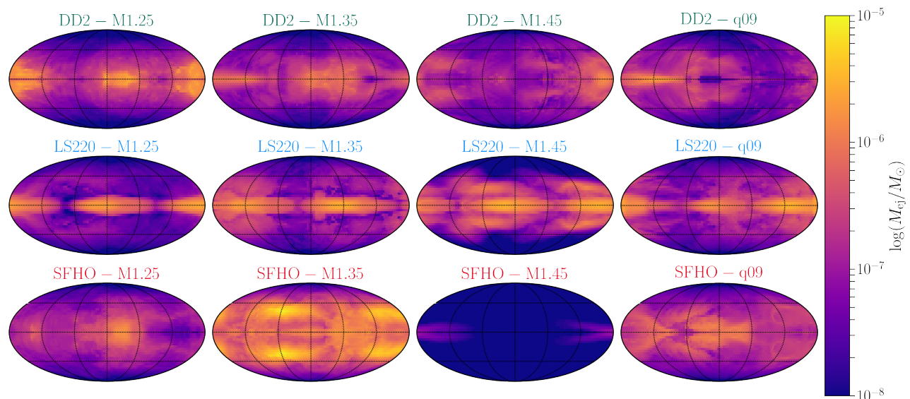
FIG. 10. Angular distribution of the ejected mass at the final time for the various binaries, with the different rows referring to the different EOSs considered.
