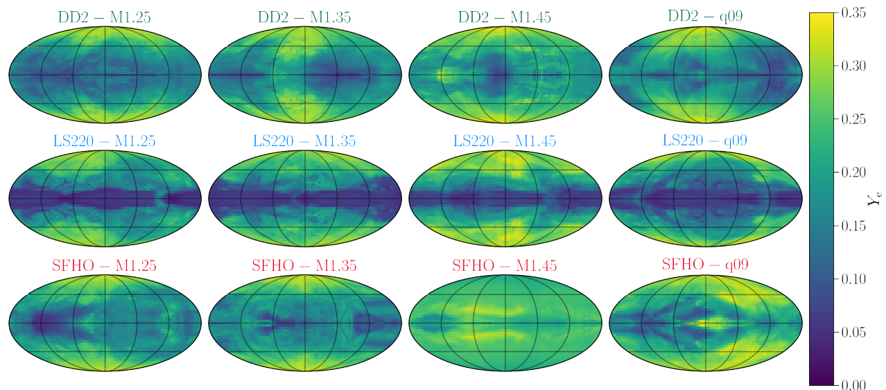
FIG. 11. The same as in Fig. 10 but for the electron fraction.
