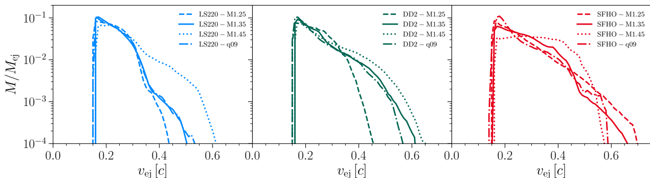
FIG. 6. The same as in Fig. 3 but for the ejecta velocity v_{\text{ej}} . The range of v_{\text{ej}} is divided into bins of width 0.05 and the histograms are normalized over the total ejected mass.
