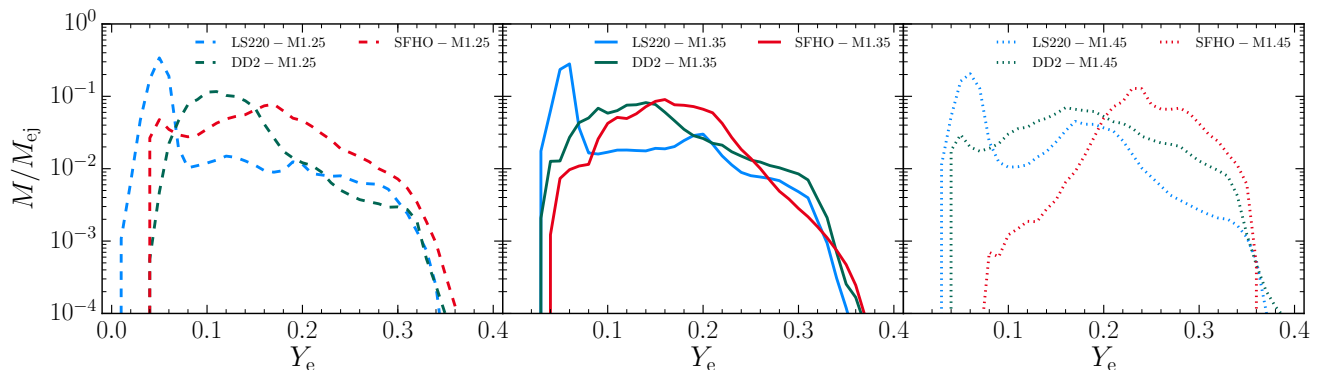
FIG. 4. Distributions of the ejected mass fraction as function of the electron fraction Y_e , as measured by a detector at radius 300 km. This is the same as Fig. 3, except that the curves are here grouped by mass configuration rather than EOS so as to highlight the dependence on the latter. For clarity, unequal-mass binaries are not shown.
