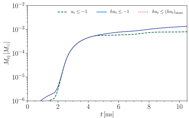
FIG. 15. Mass ejection according to different unboundness criteria for the LS220-M1.35 model. In green is the geodesic criterion, blue is the original Bernoulli one, and red is the modified Bernoulli thresholded on the atmosphere value. All values have been measured through a detector at 300 km.
