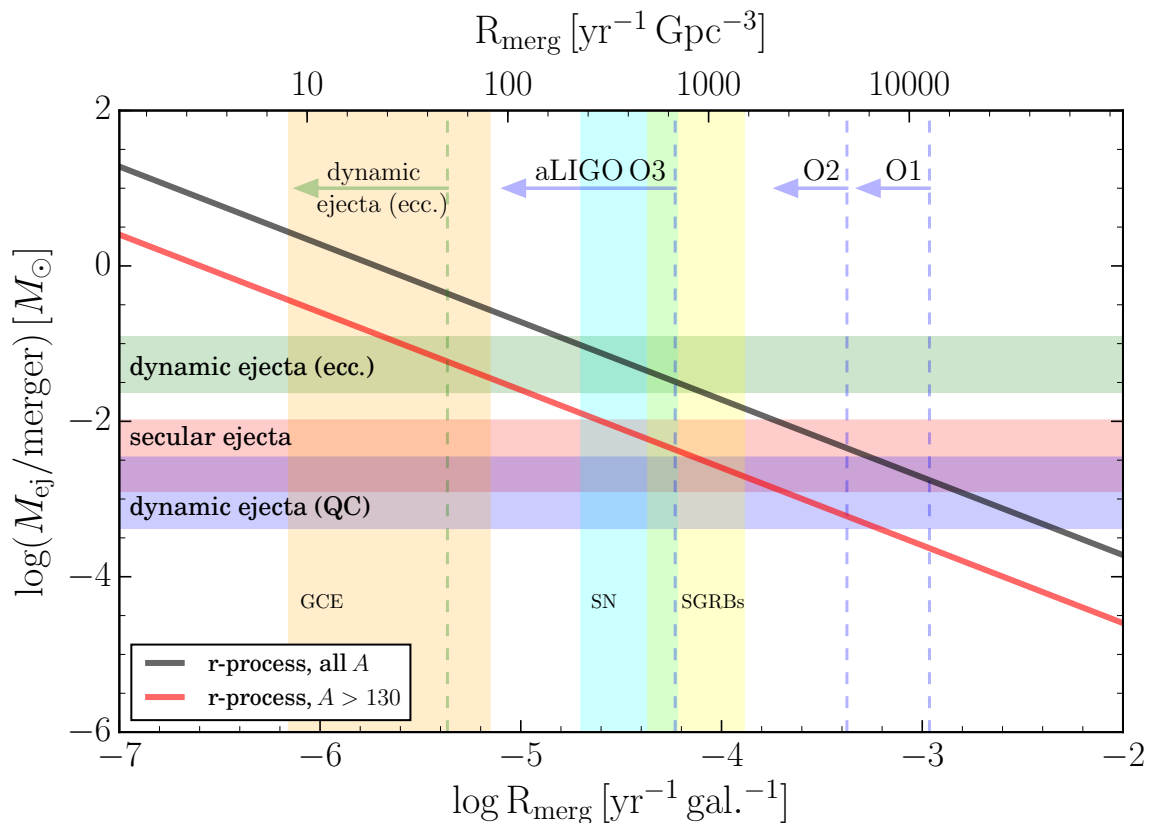
FIG. 14. Ejected material per merger for a given BNS merger rate required to reproduce the observed mass of all (black) and A > 130 (red) r-process elements in the Milky Way. The dark blue-shaded regions correspond to the range of values of ejected mass reported in Table II. The red-shaded region corresponds to ejected masses from other sources of ejecta. The dashed vertical gray lines report the observed, O1, and predicted, O2 and O3, upper bounds on BNS mergers from LIGO. The dot-dashed black line is predicted merger rate from GW170817. The orange, light blue, and yellow shaded regions correspond to observational constraints from galactic chemical evolution (GCE), supernova (SN), and short gamma-ray bursts (SGRBs) population synthesis models as defined in the text.
