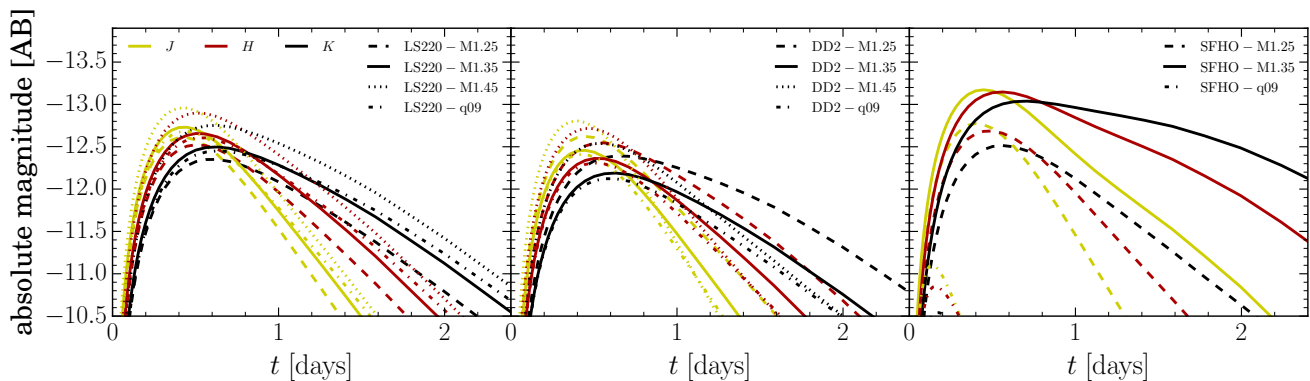
FIG. 13. Synthetic light curves in the infrared 2MASS J , H and K -bands for all of the binaries considered.
