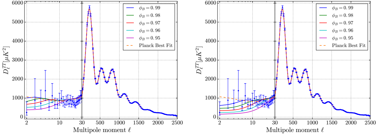
FIG. 7: TT angular power spectrum provided by Planck best fit and spectra computed for the non-oscillating vacuum with different values of the scalar field at the bounce. Left panel: m = 1.20 \cdot 10^{-6} . Right panel: m = 1.18 \cdot 10^{-6} . The corresponding cosmological parameters determined by Planck best fit for TT +lowP data are given in Ref. [2]. Both panels incorporate lensing corrections.
