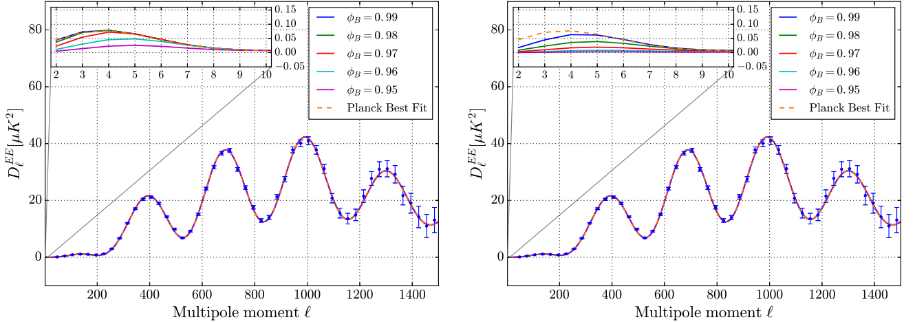
FIG. 8: EE angular power spectrum provided by Planck best fit and spectra computed for the non-oscillating vacuum with different values of the scalar field at the bounce. Left panel: m = 1.20 \cdot 10^{-6} . Right panel: m = 1.18 \cdot 10^{-6} . The corresponding cosmological parameters determined by Planck best fit for TT +lowP data are given in Ref. [2]. Both panels incorporate lensing corrections.
