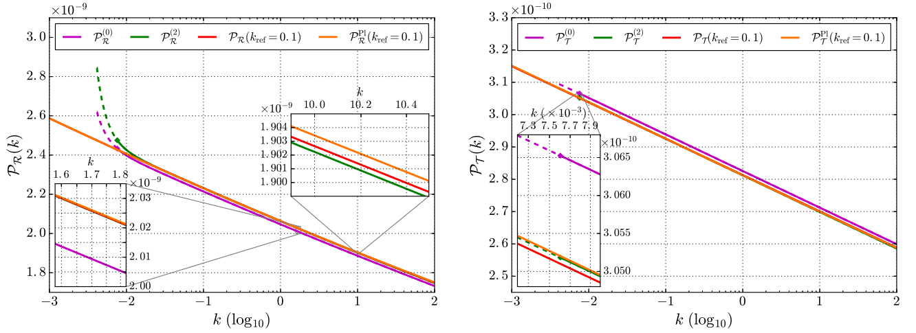
FIG. 4: Comparison between power spectra calculated with different strategies in the slow-roll regime. Here, \phi_B = 0.97 and m = 1.20 \cdot 10^{-6} . A dashed line indicates modes that exit the Hubble horizon in an inflationary phase but not in slow-roll regime. Left panel: slow-roll power spectra for the scalar perturbations. Right panel: slow-roll power spectra for the tensor perturbations.
