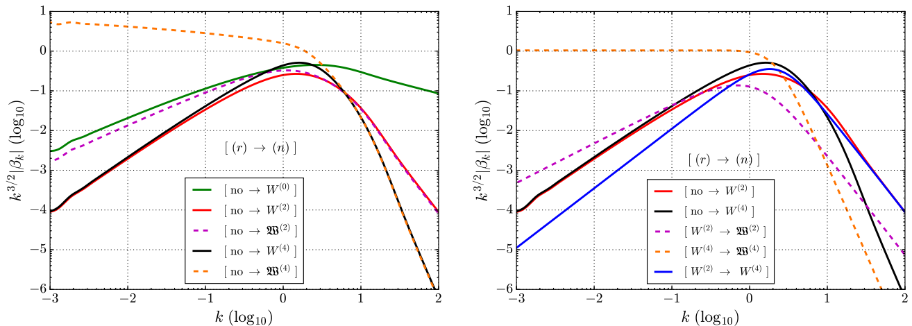
FIG. 3: Comparison between different vacuum prescriptions for the initial data of the tensor perturbations, for \phi_B = 0.97 and m = 1.20 \cdot 10^{-6} : absolute value of the antilinear coefficients of the Bogoulibov transformation relating the vacuum state of reference, (r) , with another vacuum, (n) . Left panel: comparison taking the non-oscillating (no) vacuum as the reference state.
