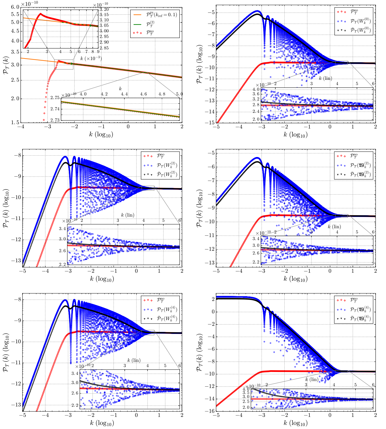
FIG. 5: Comparison between primordial power spectra obtained with different sets of solutions for the perturbations. Here, \phi_B = 0.97 and m = 1.20 \cdot 10^{-6} .
