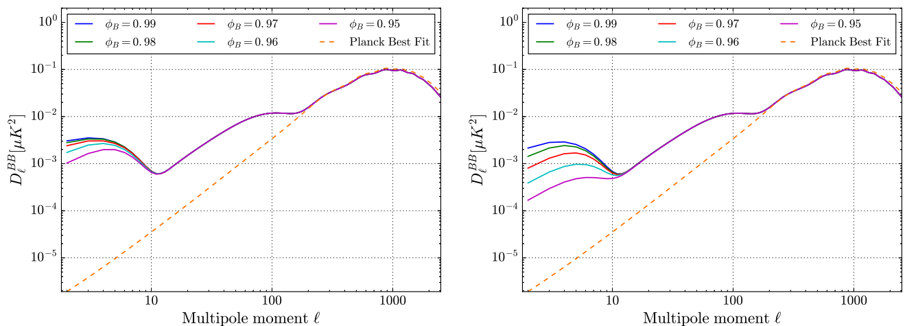
FIG. 10: BB angular power spectrum provided by Planck best fit and spectra computed for the non-oscillating vacuum with different values of the scalar field at the bounce. Left panel: m = 1.20 \cdot 10^{-6} . Right panel: m = 1.18 \cdot 10^{-6} . The corresponding cosmological parameters determined by Planck best fit for TT+lowP data are given in Ref. [2]. Both panels incorporate lensing corrections.
