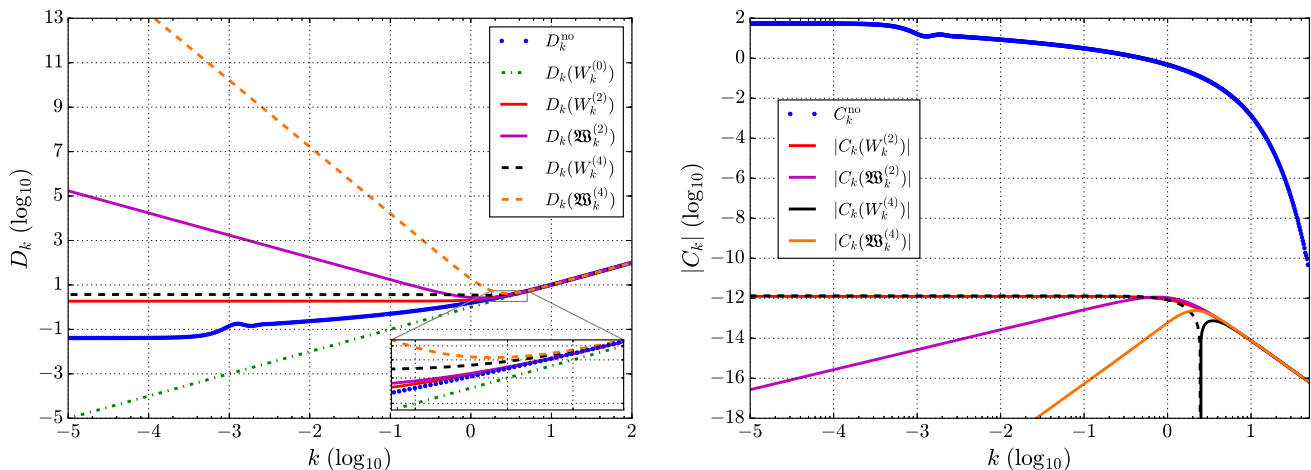
FIG. 2: Comparison between different vacuum prescriptions: functions that determine the initial conditions of the tensor field, for \phi_B = 0.97 and m = 1.20 \cdot 10^{-6} . Left panel: function D_k . Note that D_k(\mathfrak{W}_k^{(0)}) = k = D_k(W_k^{(0)}) . Right panel: function C_k . Here, dashed lines indicate negative values of C_k . We note that, for the 0th-order adiabatic initial conditions, C_k(\mathfrak{W}_k^{(0)}) = 0 = C_k(W_k^{(0)}) .
