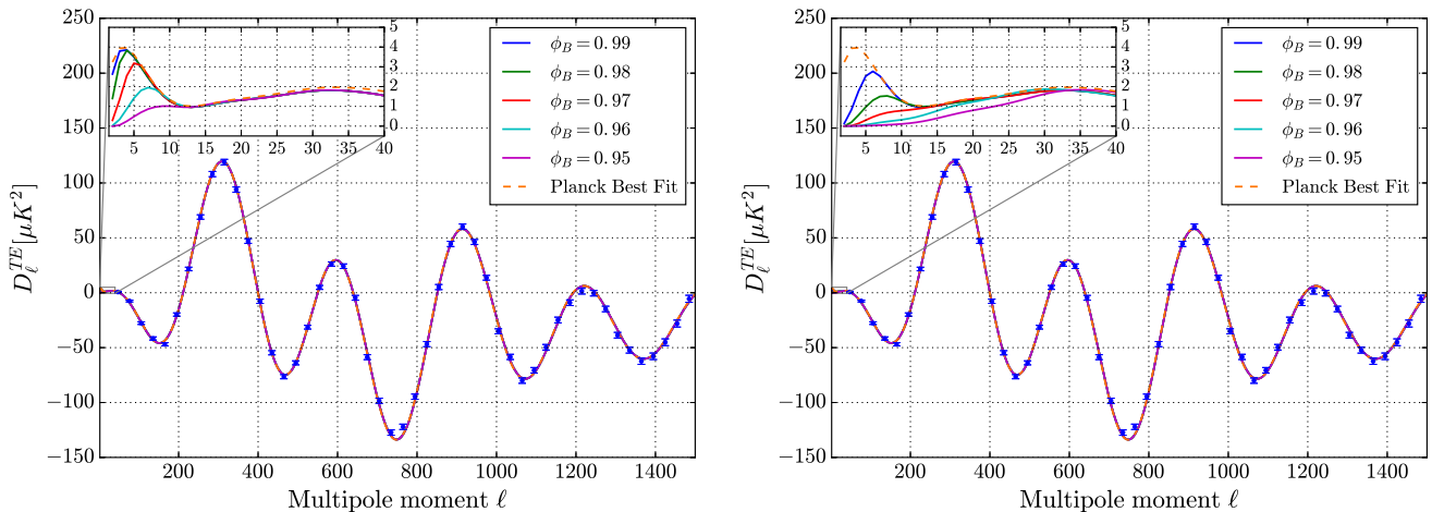
FIG. 9: TE angular power spectrum provided by Planck best fit and spectra computed for the non-oscillating vacuum with different values of the scalar field at the bounce. Left panel: m = 1.20 \cdot 10^{-6} . Right panel: m = 1.18 \cdot 10^{-6} . The corresponding cosmological parameters determined by Planck best fit for TT+lowP data are given in Ref. [2]. Both panels incorporate lensing corrections.
