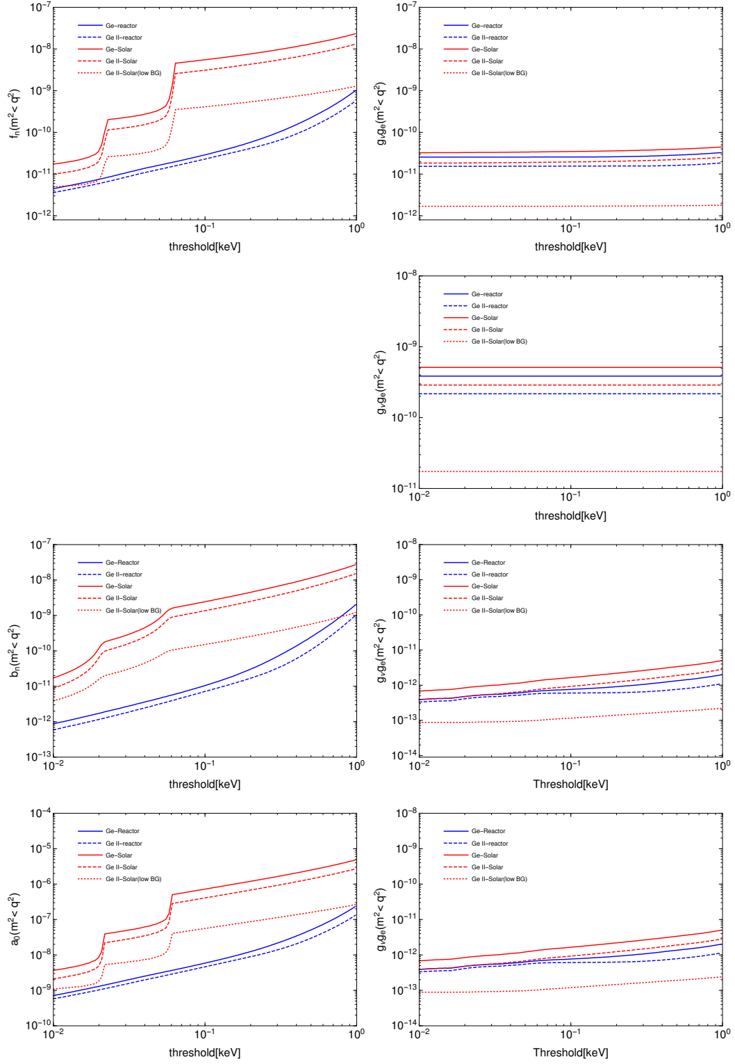
FIG. 5. Discovery limits vs. threshold for neutrino scattering off germanium nuclei (left) and electrons (right), for the different BSM models (from top to bottom): scalar, pseudo-scalar, vector and axial-vector
