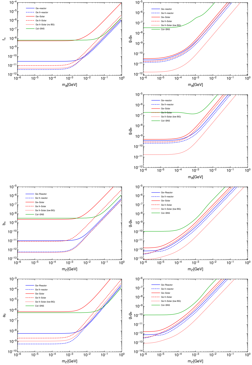
FIG. 3. Discovery limits for neutrino scattering off germanium nuclei (left) and electrons (right), for the different BSM models (from top to bottom): scalar, pseudo-scalar, vector and axial-vector
