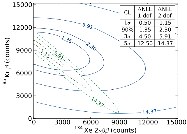
Figure 4. Contour lines of the profile-likelihood ratio, \Delta\text{NLL} , scanned for the ^{85}\text{Kr } \beta and ^{134}\text{Xe } 2\nu\beta\beta components using two NLL functions. The blue solid lines were obtained using the same function as the ^{134}\text{Xe } 2\nu\beta\beta search, which accounts for all the systematic errors. The green dashed lines were evaluated without consideration of the normalization errors. The table shows \Delta\text{NLL} values of various CL for 1 and 2 dof.
