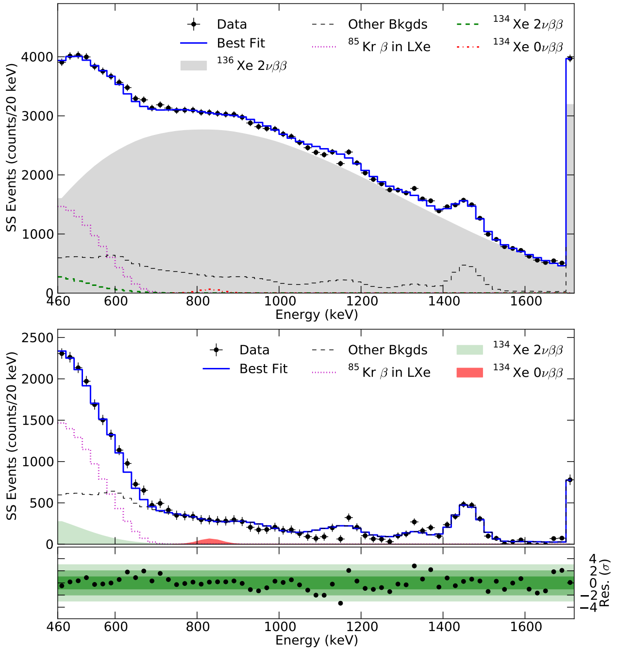
Figure 3. The top plot shows the SS energy projection for the results of the ^{134}\text{Xe} - 2\nu\beta\beta analysis, using the fitted central values. While the 0\nu\beta\beta search is performed in a separate fit with higher energy threshold, it is overlaid here for comparison since the backgrounds at these energies are the same. The last bin is the summed contents of all bins between 1700 keV and 9800 keV. The middle plot shows the same results where the ^{136}\text{Xe} - 2\nu\beta\beta component is subtracted from data and best fit values. The bottom plot presents the residuals between data and best fit normalized to the Poisson error.
