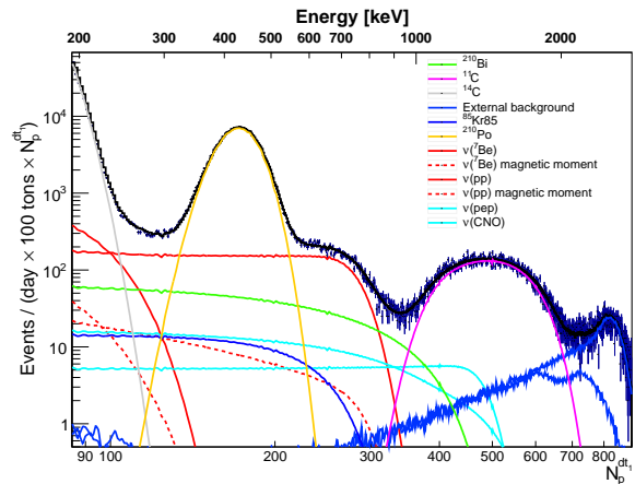
FIG. 1. Spectral fit with the neutrino effective moment fixed at \mu_{\nu}^{eff} = 2.8 \times 10^{-11} \mu_B (note the scale is double logarithmic to underline the contributions at lower energies). The fitting curves for \mu_{\nu}^{eff} = 2.8 \times 10^{-11} \mu_B and \mu_{\nu}^{eff} = 0 are visually indistinguishable.
