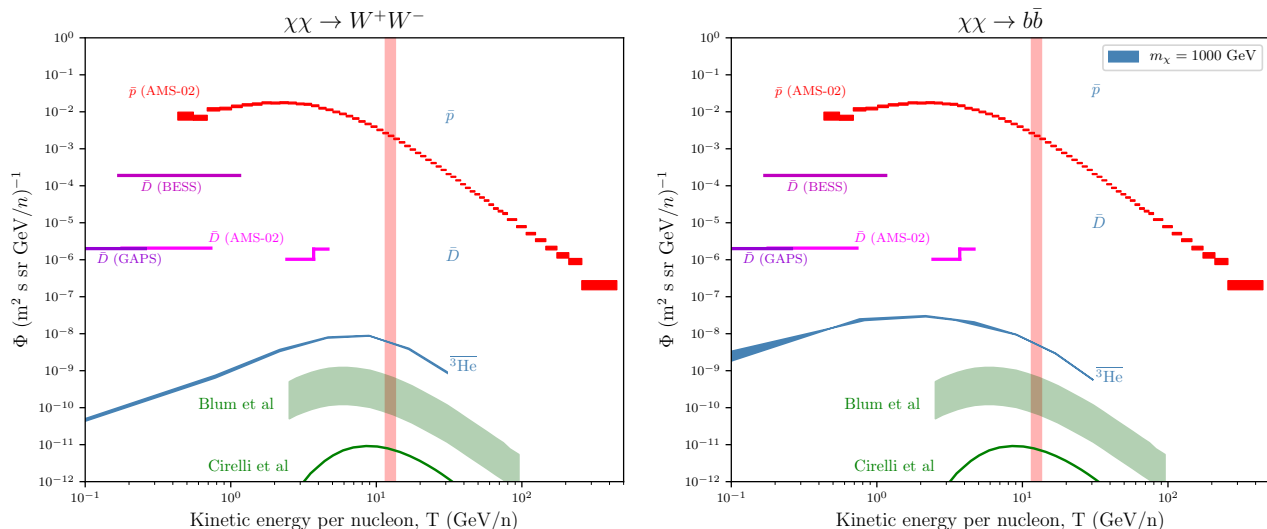
FIG. 1. The predicted antinucleon fluxes for a 1 TeV dark matter particle pair-annihilating into W^+W^- (left panel) and b\bar{b} (right panel), normalized to yield one {}^3\text{He} at 12 GeV/n in five years. The spectra were computed using a Fisk potential of \phi_F = 1.5 GV, MethodAnn for {}^3\text{He} -ISM interactions, and the MIN propagation parameters. The thickness of the lines reflects the uncertainties in the coalescence momentum for {}^3\text{He} formation in the case of antiprotons, and the combined uncertainty in the coalescence momentum relevant for {}^3\text{He} and \bar{D} formation for the \bar{D} flux. The green regions are the {}^3\text{He} background estimates from Blum et al’s recent paper [14] and from Cirelli et al [4]. The red rectangles indicate the AMS-02 antiproton flux data, while the pink and purple lines indicate the current (BESS [15]) and future (AMS-02 and GAPS [16, 17]) sensitivities to antideuterons. While the original GAPS satellite mission proposal projected a {}^3\text{He} sensitivity of 10^{-9} ( \text{m}^2\text{s sr GeV}/n ) ^{-1} for 0.1 \text{ GeV}/n \lesssim T \lesssim 0.25 \text{ GeV}/n [18], the detector design has been changed and there is no planned satellite mission. There is no current {}^3\text{He} sensitivity estimate, though it is expected to be similar to the \bar{D} sensitivity [12].
