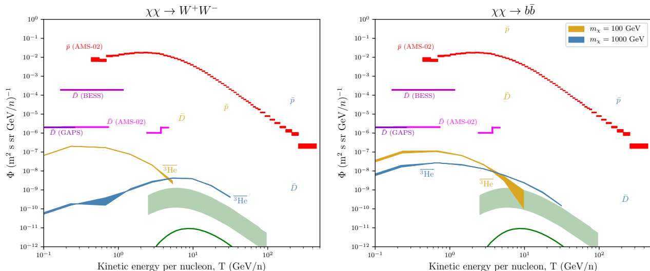
FIG. 2. As in Fig. 1, but for the predicted antiproton and antideuteron fluxes for 100 GeV (yellow lines) and 1 TeV (blue lines) dark matter particles pair-annihilating into W^+W^- (left panel) and \bar{b}b (right panel), normalized to yield one {}^3\text{He} per year overall. Spectra are computed using \phi_F = 500 MV, MethodAnn and MAX propagation.
