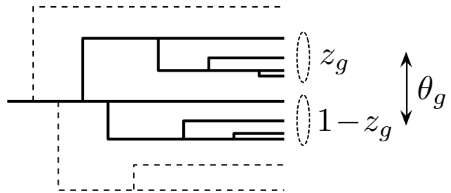
FIG. 8. Schematic of the soft drop algorithm, which recursively removes branches from the C/A clustering tree if the momentum fraction z fails to satisfy z > z_{\text{cut}}\theta^\beta . The g subscript indicates the final groomed kinematics.
