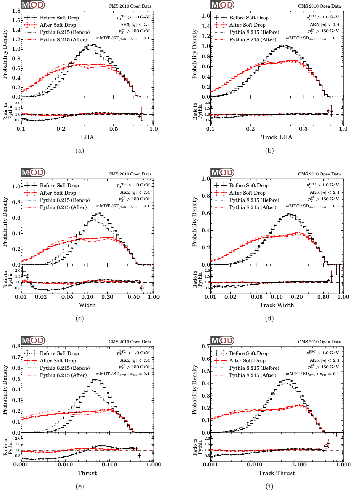
FIG. 19. Same observables as in Fig. 19, but now showing the original distributions (black) compared to those obtained after soft drop declustering (red).
