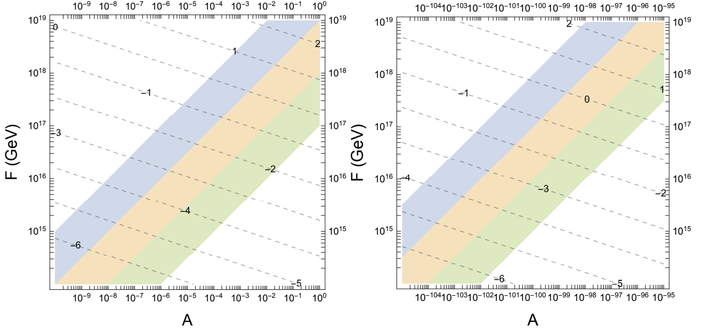
Figure 1: Axion relic abundance and mass as a function of axion decay constant F and Wilson coefficient A . The dashed contours denote the axion relic abundance and are labelled by \log_{10}(\Omega_{ax}h^2) ; the -1 contour is the observed relic abundance. The blue, orange, and green bands are mass regions 10^{-23}\text{eV} \leq m_a \leq 10^{-22}\text{eV} , 10^{-22}\text{eV} \leq m_a \leq 10^{-21}\text{eV} , and 10^{-21}\text{eV} \leq m_a \leq 10^{-20}\text{eV} , respectively, so that the m_a = 10^{-22}\text{eV} line is the boundary between the blue and orange bands. Left : the n = 3 case, which accommodates the relic abundance and mass by using the electroweak hierarchy. Right : the n = 0 case, which accommodates these solely with instanton suppression.
