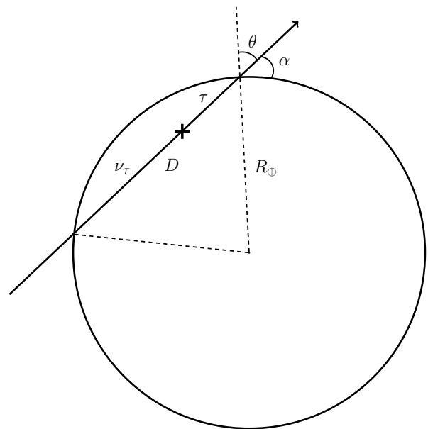
FIG. 16. Chord length through the Earth D for nadir angle \theta and radius of the Earth R_\oplus .
