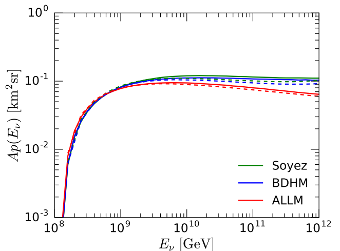
FIG. 20. The effective aperture for the Pierre Auger Observatory for A = 3,000 \text{ km}^2 using the analytic approximation to the tau survival probability in rock and an approximate efficiency for detection, for Soyez, BDHM and ALLM models for both energy loss and neutrino cross section (solid line), and with the NLO perturbative neutrino cross section substituted (dashed lines).
