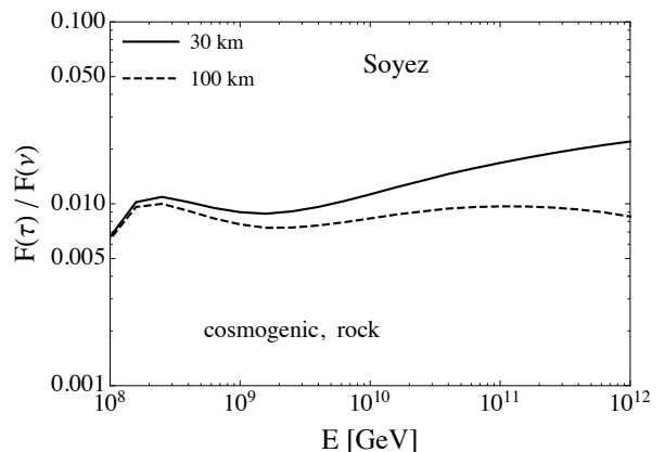
FIG. 14. The transmission function calculated analytically for incident cosmogenic neutrino flux and with tau energy loss in the Soyez approach, for a depth of 30 and 100 km rock.
