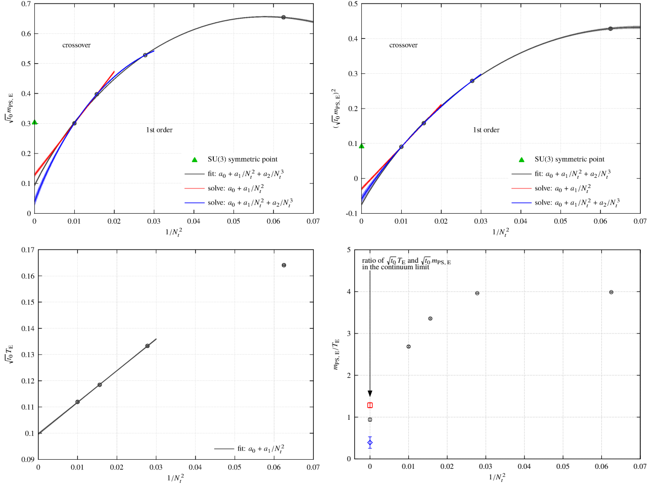
FIG. 6. Continuum extrapolation of the critical point \sqrt{t_0} m_{\text{PS},E} (upper-left), (\sqrt{t_0} m_{\text{PS},E})^2 (upper-right), \sqrt{t_0} T_E (lower-left) and m_{\text{PS},E}/T_E (lower-right). Note that the continuum value of m_{\text{PS},E}/T_E in the lower-right panel is obtained by using the ratio of \sqrt{t_0} m_{\text{PS},E} and \sqrt{t_0} T_E in the continuum limit obtained in the upper-left and the lower-left panel respectively.
