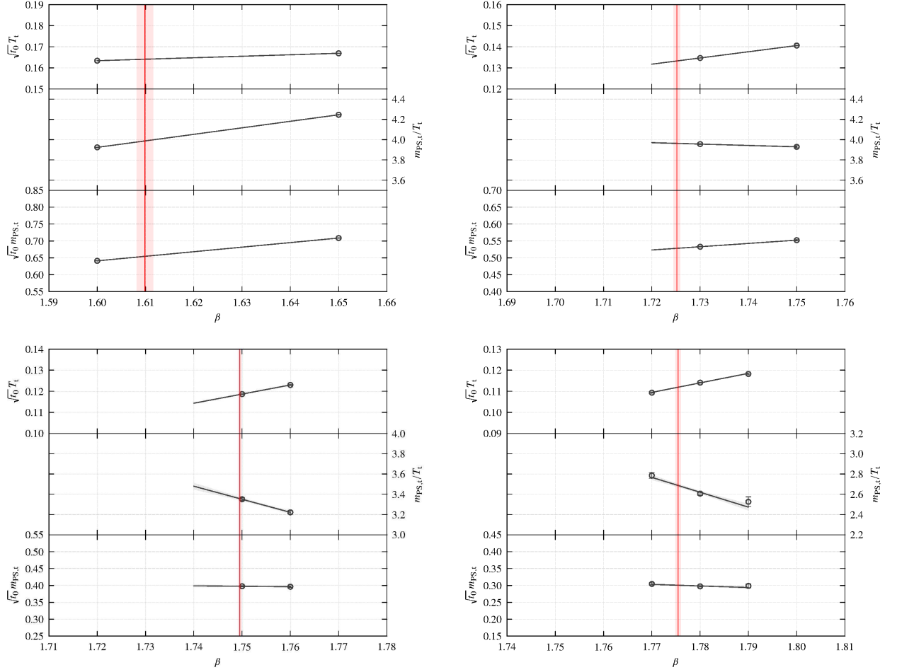
FIG. 5. \sqrt{t_0}T , m_{PS}/T and \sqrt{t_0}m_{PS} along the transition line projected on \beta for N_t = 4 (upper left), 6(upper right), 8(lower left) and 10(lower right). The vertical red line shows the location of the critical value of \beta determined by the kurtosis intersection analysis.
