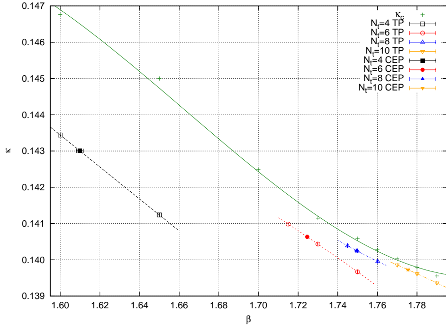
FIG. 2. Phase diagram for bare parameter space (\beta, \kappa) at N_t = 4, 6, 8 and 10 . The open symbols represent a transition/crossover point while the filled symbols are the critical end points determined by the kurtosis intersection with new formula. On the transition line, the left (right) hand side of an critical end point is the first order phase transition (crossover) side. Polynomial interpolation is used to determine the phase transition line. \kappa_c is the pseudo-scalar massless point with N_f = 3 at the zero temperature.
