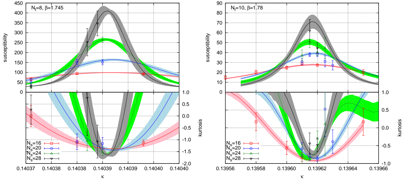
FIG. 1. The susceptibility (upper half) and kurtosis (lower half) of chiral condensate as a function \kappa with several spatial sizes, N_s = 16 - 28 . The left panel is for (N_t, \beta) = (8, 1.745) and the right is for (N_t, \beta) = (10, 1.78) . The raw data points (as symbols) as well as the multi-ensemble reweighting ( 1\text{-}\sigma band) are plotted.
