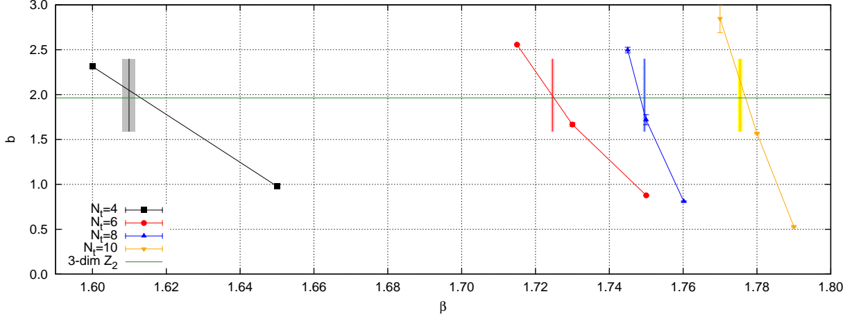
FIG. 4. Exponents of the susceptibility peak height along the transition line projected on \beta value for N_t = 4, 6, 8 and 10 . The line connecting the data points is to guide readers' eyes. The point where the line for each N_t intersects the (green) horizontal line is an estimate of the critical point assuming the Z_2 universality class. On the other hand, the shaded areas represent the critical \beta determined by the kurtosis intersection analysis.
