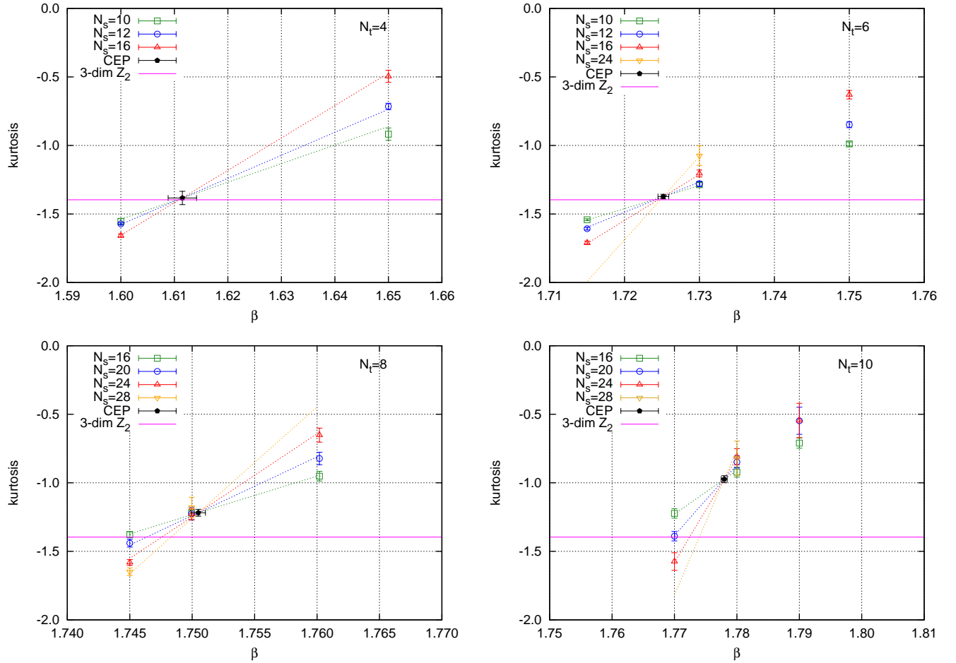
FIG. 3. Kurtosis intersection for chiral condensate at N_t = 4, 6, 8 and 10 . The simple fitting form: K = K_E + AN_s^{1/\nu}(\beta - \beta_E) is also drawn in the figure. For N_t = 4 and 6 , the values of kurtosis at the crossing point (black pentagon) is consistent with the three-dimensional Z_2 universality class, while for N_t = 8 and 10 , obviously it is not consistent. The conclusion of this paper is based on the fitting form with a correction term. See text for details.
