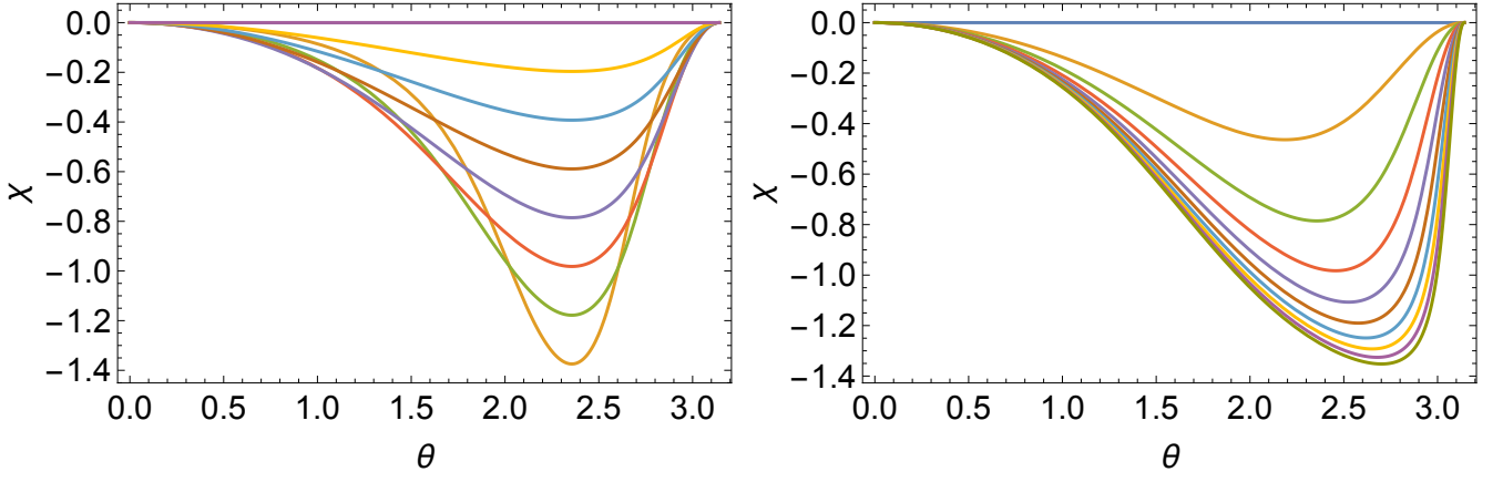
FIG. 1. Rotation of the polarization angle \chi as function of the direction of the velocity \theta with respect to the photon propagation in the rest frame. Left Panel: \gamma = 2 , different position angles \phi = 0, \pi/16 \dots \pi/2 . Right Panel: \phi = \pi/4 , different Lorentz factor, \gamma = 1, 2, \dots 10 . (Only a fraction of the curve is revealed to the observer through the generally narrow radio beam.)
