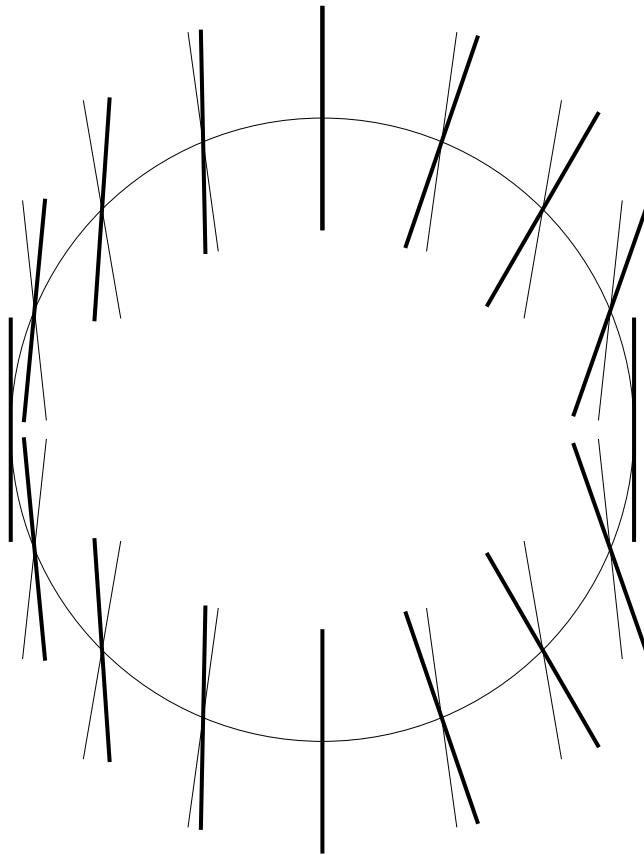
FIG. 2. Polarization pattern produced by a moving strong lens as viewed by an observer. The source is polarized along the vertical direction. Thin lines indicate polarization direction for stationary lens; thick lines indicate polarization direction for a lens moving horizontally, in a direction transverse to the initial photon propagation. The circle represents the Einstein ring. The effects of motion are exaggerated for clarity. Lens is moving from left to right, as seen by the observer.
