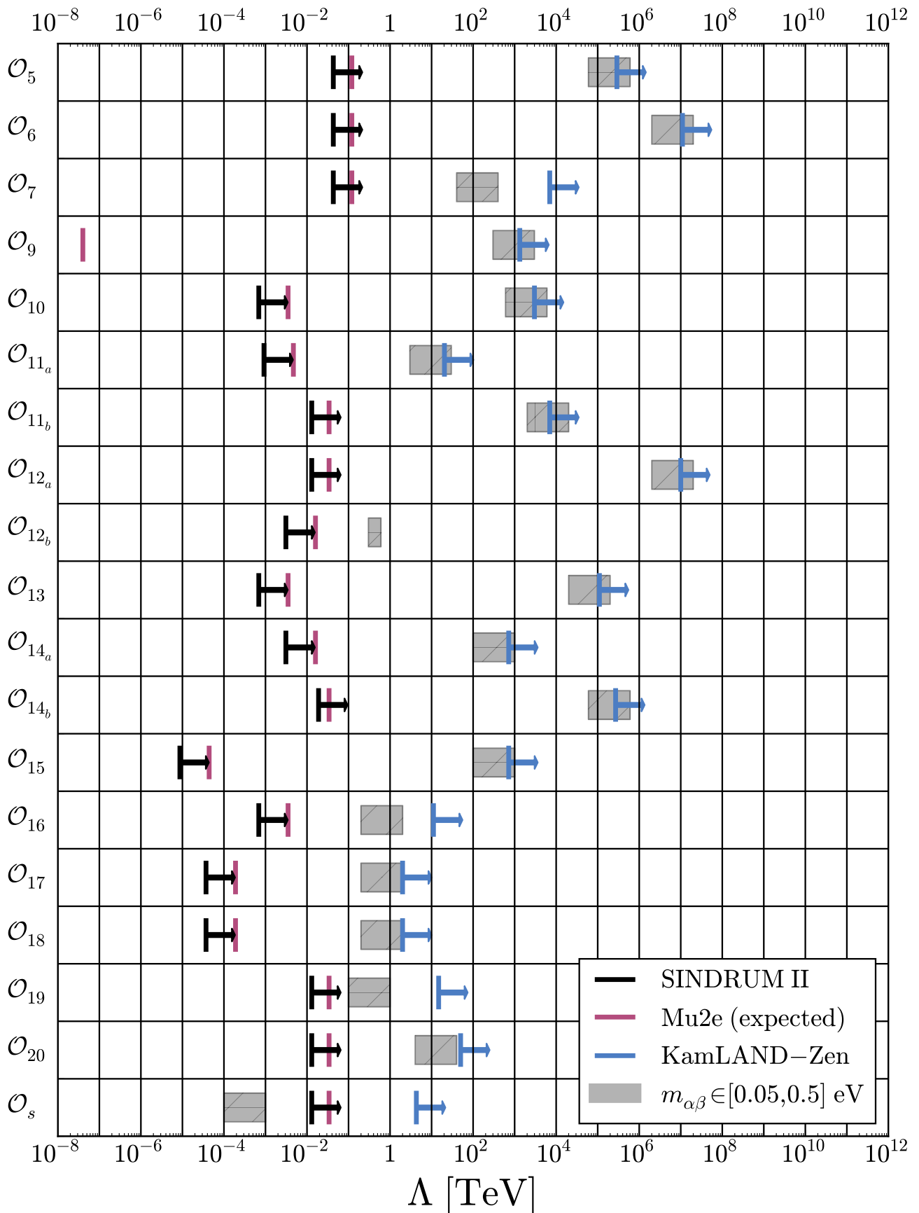
FIG. 7: Bounds on the effective scale associated with the dimension-nine operators listed in Table III from the KamLAND-Zen experiment for 0\nu\beta\beta (blue) and SINDRUM-II experiment for \mu^- \rightarrow e^+ (black). Also shown are the estimated sensitivity of the Mu2e experiment (pink) and the range of \Lambda for which m_{\alpha\beta} \sim 0.05 - 0.5 eV (grey). We assume g_{\alpha\beta\dots} = 1 for all coefficients here. See text for details.
