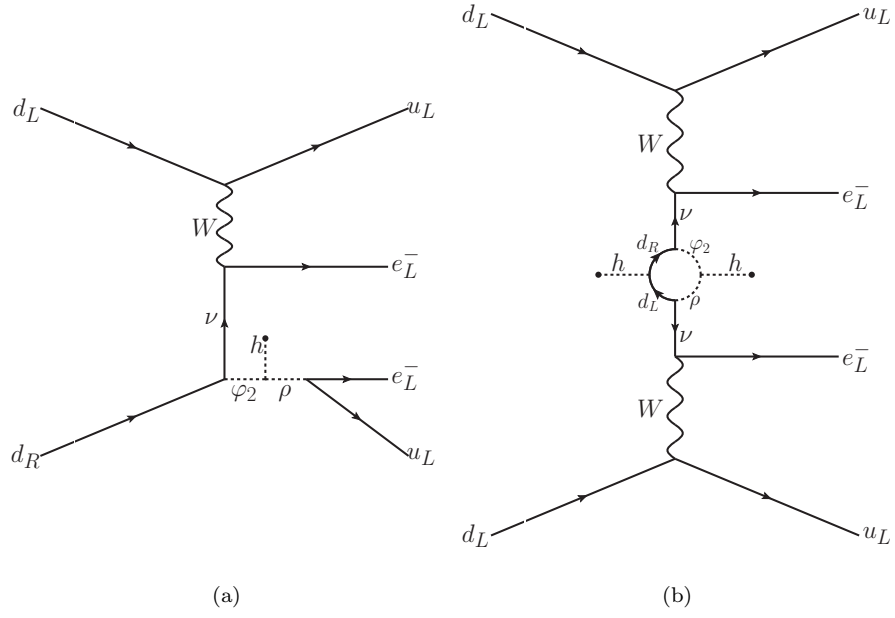
FIG. 8: The tree-level (a) and one-loop-level (b) contributions of 0\nu\beta\beta from the model presented in Eq. (A.2).
