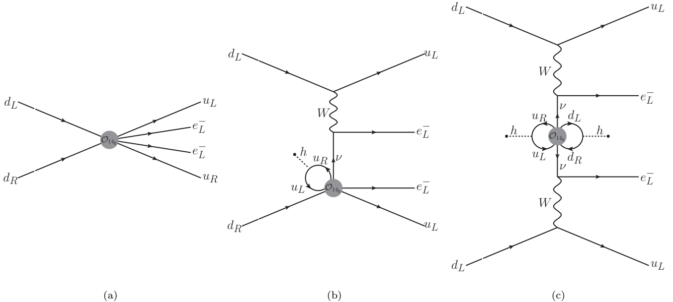
FIG. 1: Feynman diagrams contributing to 0\nu\beta\beta from the operator \mathcal{O}_{14b} = (L\bar{Q})(LQ)\bar{u}^c d^c . The dominant contributions scaling as \Gamma \sim \Lambda^{-10} (a), \Lambda^{-6} (b), and \Lambda^{-2} (c) are depicted.
