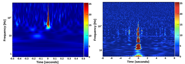
FIG. 6. OmegaScan: Type C glitch in LHO strain channel (left) and lightning glitch in LLO magnetometer (right). Plots generated through LIGOdV-web [45].
