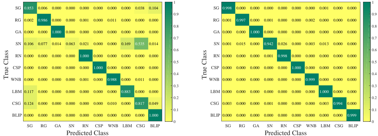
FIG. 4. Confusion Matrix for Simulated Data: Results from traditional SVM (left) and DBNN (right) classifiers. Closer a diagonal element to unity, better is the classification for the corresponding type. Accuracy of our method is thus evident.
