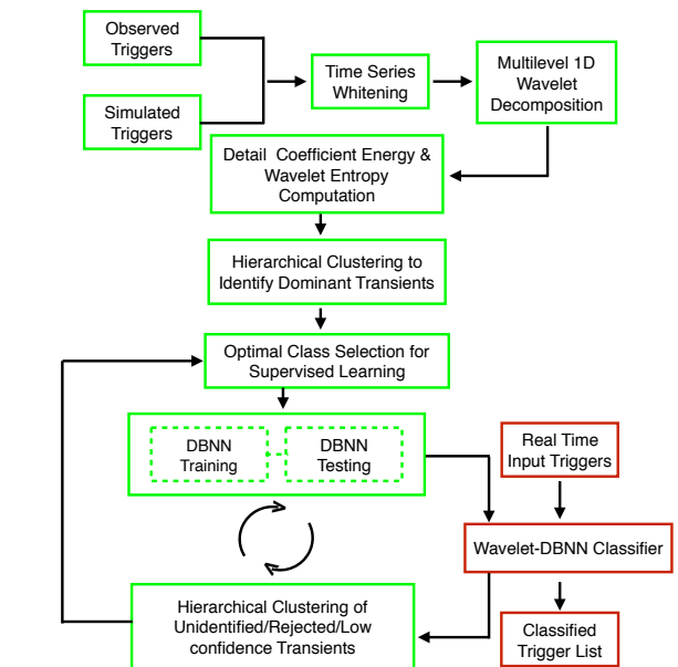
FIG. 3. Block diagram of the proposed hybrid classifier.
