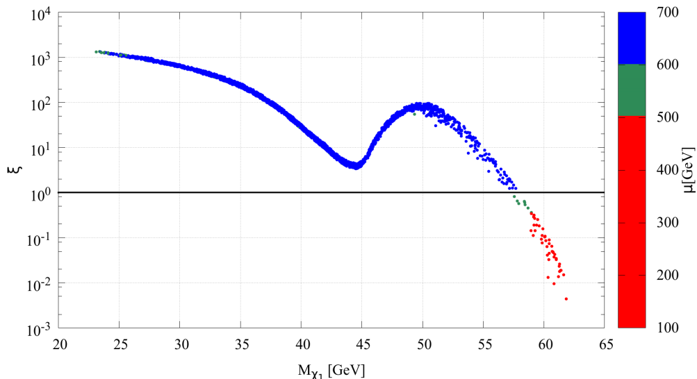
Figure 19: Scatter plot in the \xi - M_{\tilde{\chi}_1^0} plane for parameter space points which can be probed by LZ through the SD WIMP-neutron interactions, by Xenon-nT through the SI WIMP-nucleon based interactions and by ILC through the Higgs to invisible branching fraction. The color palette corresponds to the value of the higgsino mass parameter ( \mu ).
