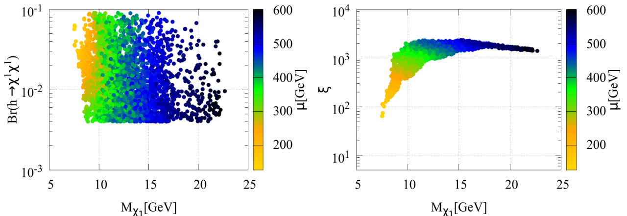
Figure 15: (a) Scatter plot in the Br(h \rightarrow \tilde{\chi}_1^0 \tilde{\chi}_1^0) - M_{\tilde{\chi}_1^0} plane and (b) in the \xi - M_{\tilde{\chi}_1^0} plane for parameter space points which can be probed by PICO-250 through the SD WIMP-proton interactions, by Xenon-nT through the SI WIMP-nucleon based interactions and also by ILC through the Higgs to invisible branching. The color palette corresponds to the value of the higgsino mass parameter ( \mu ).
