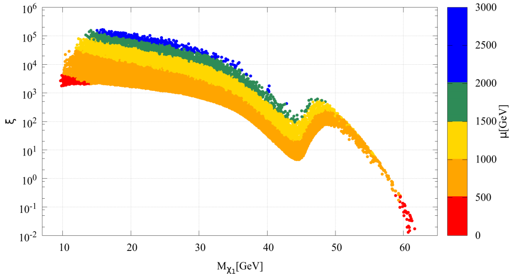
Figure 14: Scatter plot in the \xi - M_{\tilde{\chi}_1^0} plane for parameter space points which can be probed by Xenon-nT through the SI WIMP-nucleon interactions and also by ILC through the Higgs to invisible branching. The color palette corresponds to the value of the higgsino mass parameter ( \mu ).
