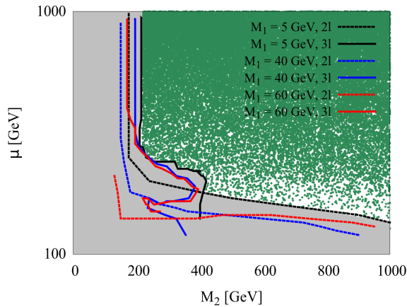
Figure 1: 95% C.L. contours in the \mu - M_2 plane from dilepton (dashed) and tripleton (solid) searches at LHC-8 TeV for M_1 = 5, 40, 60 GeV. Here \tan\beta = 10 . Green points correspond to the allowed points of the scan after imposing all constraints in Sec. 2. Only the region \mu < 1 TeV is displayed, as the contours are independent of \mu for low values of M_2 .
