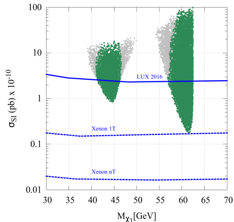
Figure 5: Unscaled SI WIMP-nucleon cross-section vs M_{\tilde{\chi}_1^0} for all points allowed by collider and relic density constraints. The blue-solid line shows the current limit from LUX-2016 [109] and the blue-dashed lines show the projected reach for Xenon-1T [110] and Xenon-nT [110].
