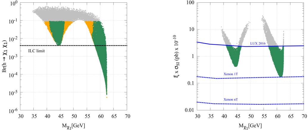
Figure 2: a) The Higgs to invisible branching Br(h \rightarrow \tilde{\chi}_1^0 \tilde{\chi}_1^0) vs. the LSP mass M_{\tilde{\chi}_1^0} . The grey (coloured) points distinguish the points allowed before (after) the Higgs signal strength constraints. Yellow (green) points are excluded (allowed) by the current limits on SI WIMP-nucleon cross-section from LUX-2016 [109]. The black-dashed line represents the ILC reach, Br(h \rightarrow \tilde{\chi}_1^0 \tilde{\chi}_1^0) > 0.4\% [25]. b.) SI WIMP-nucleon cross-section vs M_{\tilde{\chi}_1^0} for all points allowed by collider and relic density constraints. The blue-solid line show the current limit from LUX-2016 [109] and the blue-dashed lines shows the projected reach for Xenon-1T [110] and Xenon-nT [110].
