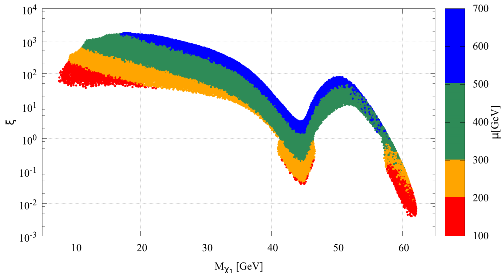
Figure 20: Scatter plot in the \xi - M_{\tilde{\chi}_1^0} plane for parameter space points which can be probed by PICO-250 through the SD WIMP-proton interactions, by LZ through the SD WIMP-neutron interaction, by Xenon-nT through the SI WIMP-nucleon based interactions, and also by ILC through the Higgs to invisible branching fraction. The color palette corresponds to the value of the higgsino mass parameter ( \mu ).
