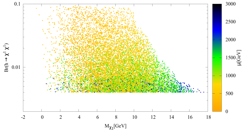
Figure 10: Scatter plot in the Br(h \rightarrow \tilde{\chi}_1^0 \tilde{\chi}_1^0) - M_{\tilde{\chi}_1^0} plane for parameter space points which can be probed by ILC only, through the Higgs to invisible branching fraction. The color palette corresponds to the value of the higgsino mass parameter ( \mu )
