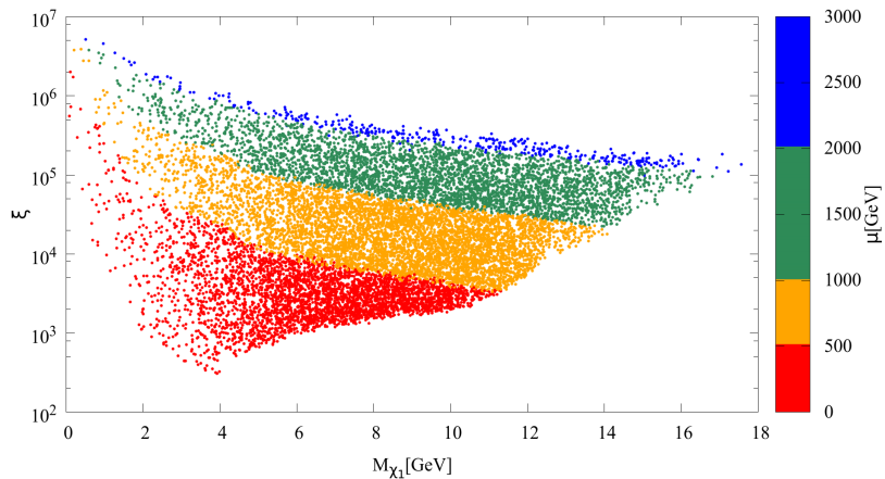
Figure 11: Scatter plot in the \xi - M_{\tilde{\chi}_1^0} plane for parameter space points which can be probed by ILC only, through the Higgs to invisible branching fraction ( Br(H \rightarrow \tilde{\chi}_1^0 \tilde{\chi}_1^0) \geq 0.4\% ). The color palette corresponds to the value of the higgsino mass parameter ( \mu )
