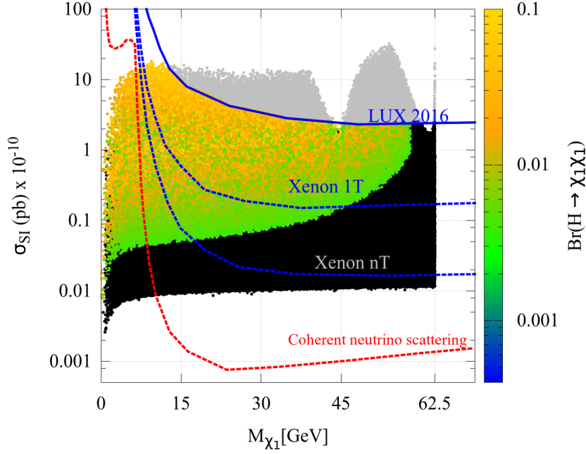
Figure 7: SI WIMP-nucleon cross-section vs M_{\tilde{\chi}_1^0} for all points allowed by collider and relic density constraints. The color code characterizes the value of Br(h \rightarrow \tilde{\chi}_1^0 \tilde{\chi}_1^0) , while black points have Br(h \rightarrow \tilde{\chi}_1^0 \tilde{\chi}_1^0) < 0.4\% . The blue-solid line shows the current limit from LUX-2016 [109] and the blue-dashed line shows the reach for Xenon-1T [110] and Xenon-nT [110].
