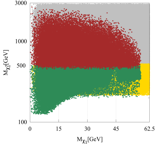
Figure 9: Represents the chargino mass ( M_{\tilde{\chi}_1^\pm} ) against M_{\tilde{\chi}_1^0} for the allowed parameter space points. The corresponding color code is mentioned in the text.
