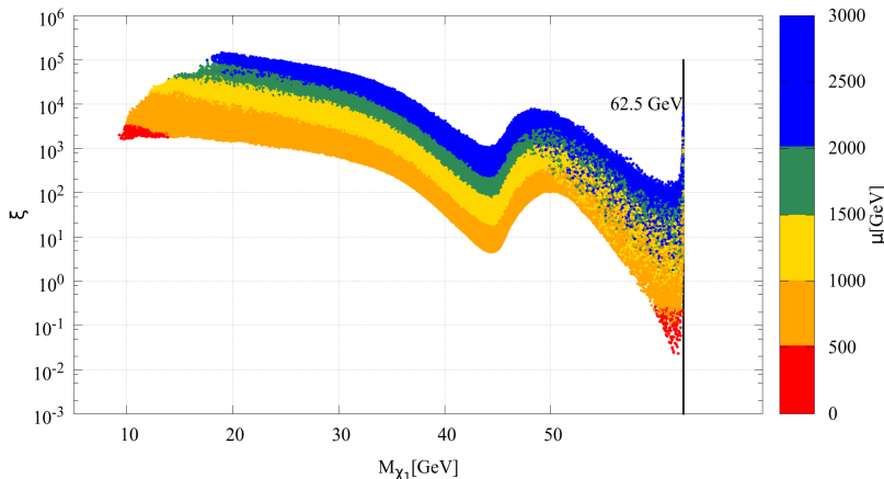
Figure 12: Scatter plot in the \xi - M_{\tilde{\chi}_1^0} plane for parameter space points which can be probed by Xenon-nT only, through the SI WIMP-nucleon interactions. The color palette corresponds to the value of the higgsino mass parameter ( \mu ).
