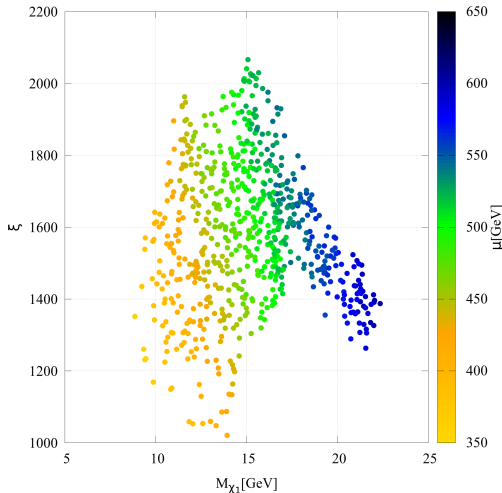
Figure 16: Scatter plot in the \xi - M_{\tilde{\chi}_1^0} plane for parameter space points which can be probed by PICO-250 through the SD WIMP-proton interactions and by Xenon-nT through the SI WIMP-nucleon based interactions. The color palette corresponds to the value of the higgsino mass parameter ( \mu ).
