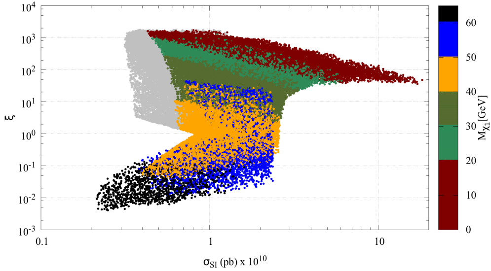
Figure 21: Scatter plot in the \sigma_{SI}-\xi plane for parameter space points which can be probed by PICO-250 through the SD WIMP-proton interactions, by LZ through the SD WIMP-neutron interaction, by Xenon-nT through the SI WIMP-nucleon based interactions, and also by ILC through the Higgs to invisible branching fraction. The color palette corresponds to the value of the LSP mass ( M_{\tilde{\chi}_1^0} ).
