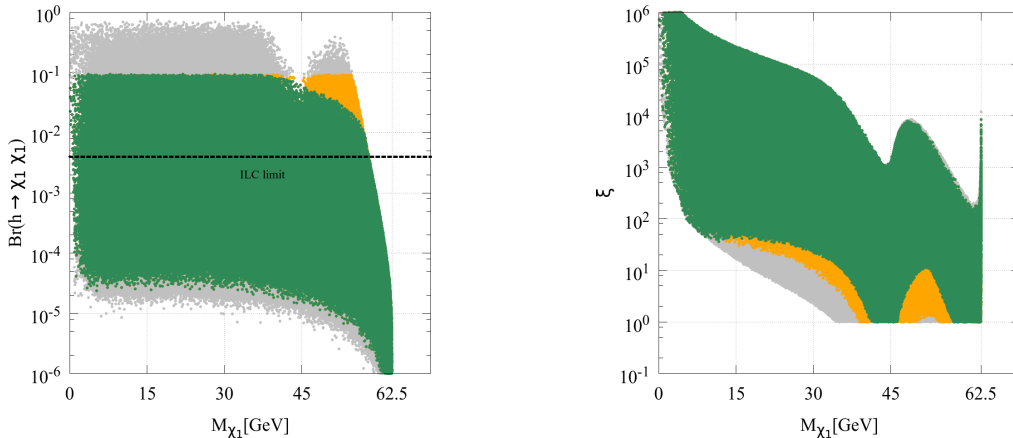
Figure 6: a) The Higgs to invisible branching fraction Br(h \rightarrow \tilde{\chi}_1^0 \tilde{\chi}_1^0) vs. the LSP mass M_{\tilde{\chi}_1^0} . b) The rescaled relic density, \xi , against M_{\tilde{\chi}_1^0} . Same colour code as Fig. 2.
