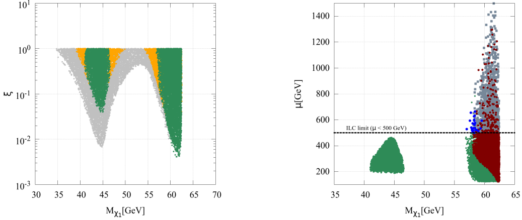
Figure 4: a) The normalized relic density, \xi = \Omega_{DM}/0.122 vs the LSP mass, same color code as in Fig. 2(a). b) higgsino mass parameter \mu against the LSP mass, the black dashed line represents the ILC sensitivity to probe \mu < 500 GeV. Here, only the parameter points allowed by collider constraints and LUX-2016 have been considered. The color code is described in the text.
