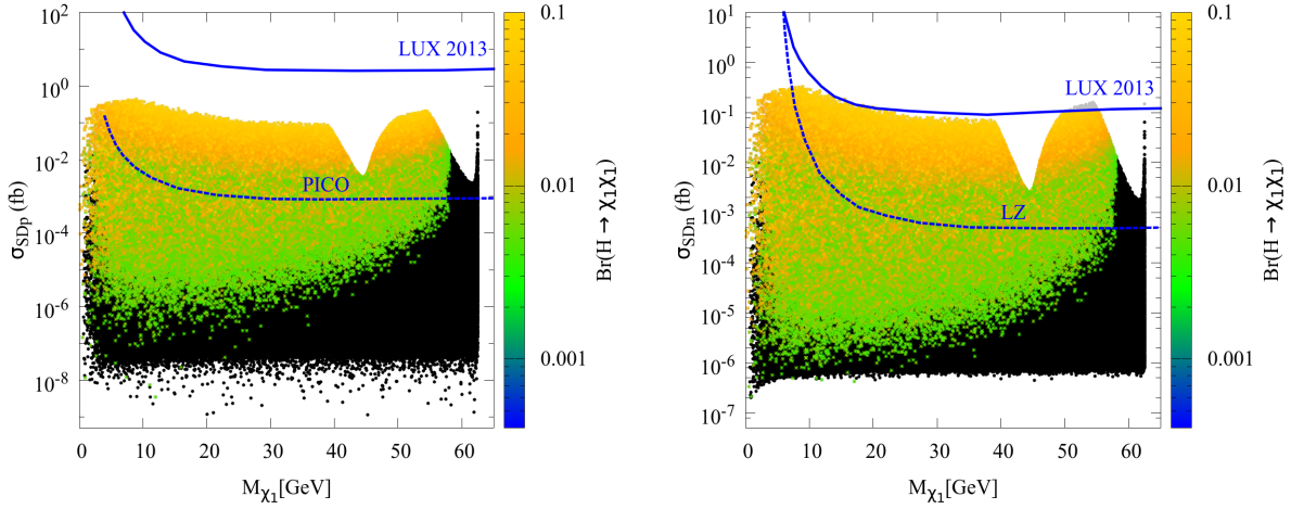
Figure 8: (a). SD WIMP-proton cross-section vs M_{\tilde{\chi}_1^0} for all points allowed by collider and relic density constraints. The blue-solid and blue-dashed line shows the current limits from LUX-2013 [112] and the reach of PICO-250 [113], respectively. (b). SD WIMP- neutron cross-section vs M_{\tilde{\chi}_1^0} for all points allowed by collider and relic density constraints. The blue-solid line and the blue-dashed line shows the current limits from LUX-2013 [112] and the reach of LZ [112], respectively. The color code characterizes the value of Br(h \rightarrow \tilde{\chi}_1^0 \tilde{\chi}_1^0) , black points have Br(h \rightarrow \tilde{\chi}_1^0 \tilde{\chi}_1^0) < 0.4\% .
