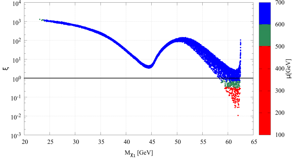
Figure 18: Scatter plot in the \xi - M_{\tilde{\chi}_1^0} plane for parameter space points which can be probed by LZ through the SD WIMP-neutron interactions and by Xenon-nT through the SI WIMP-nucleon based interactions. The color palette corresponds to the value of the higgsino mass parameter ( \mu ).
