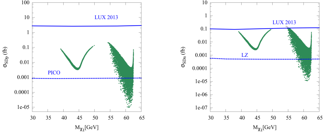
Figure 3: a) SD WIMP-proton cross-section vs M_{\tilde{\chi}_1^0} for all points allowed by collider and relic density constraints. The blue- solid line show the current limit from LUX-2013 [112] and the blue-dashed line shows the projected reach for PICO-250 [113]. b.) SD WIMP-neutron cross-section vs M_{\tilde{\chi}_1^0} for all points allowed by collider and relic density constraints. The blue-solid line show the current limit from LUX-2013 [112] and the blue-dashed line shows the projected reach for LZ [112].
