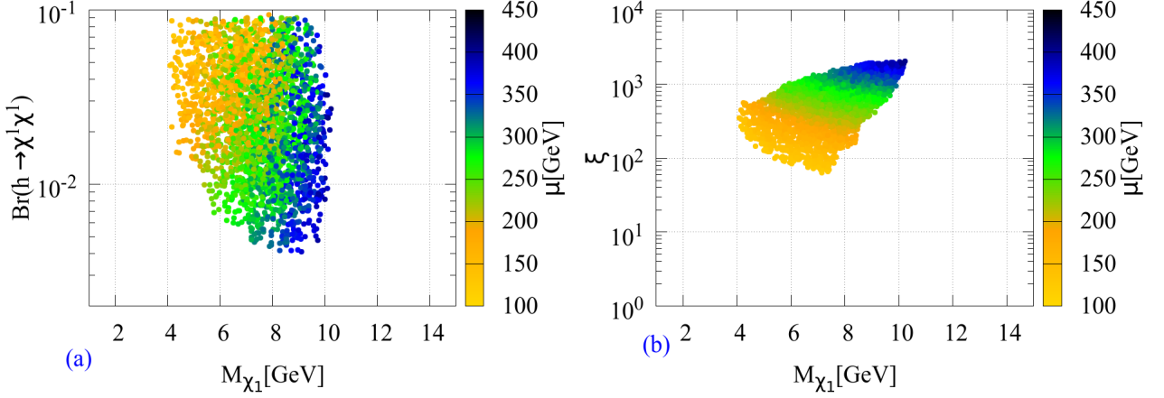
Figure 17: (a) represents scatter plot in the Br(h \rightarrow \tilde{\chi}_1^0 \tilde{\chi}_1^0) - M_{\tilde{\chi}_1^0} plane and (b) represents scatter plot in the \xi - M_{\tilde{\chi}_1^0} plane for parameter space points which can be probed by PICO-250 through the SD WIMP-proton interactions and also by ILC through the Higgs to invisible branching. The color palette corresponds to the value of the higgsino mass parameter ( \mu ).
