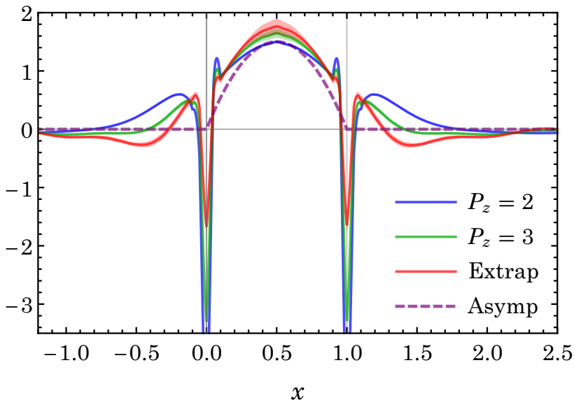
FIG. 1: The pion distribution amplitude (at \mu = 2 GeV) after implementing one-loop and mass correction for P_z = 2 (blue) and 3 (green) (in units of 2\pi/L ) to the quasi-distribution amplitude. The extrapolation to infinite momentum to remove the remaining higher-twist effects is shown in red. The Wilson-line renormalization that removes the power divergent contribution is not included in this plot, and will be implemented later in the results of improved pion quasi-DA. The purple dashed line is the asymptotic form 6x(1-x) .
