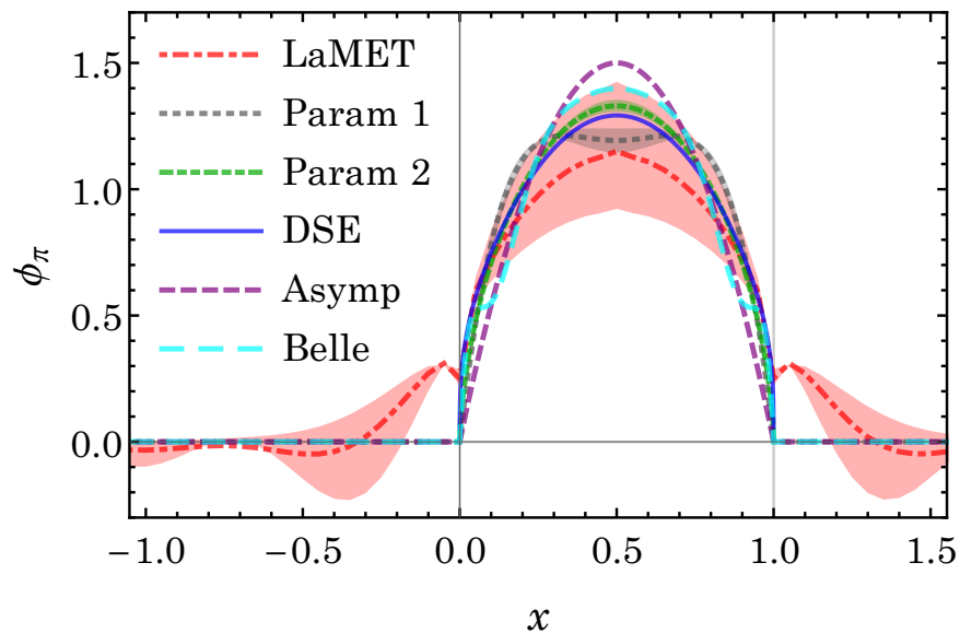
FIG. 4: Pion distribution amplitude at \mu = 2 GeV with \delta m = (0.38 \pm 0.28)\delta m_{1\text{-loop}} (red band with the central value denoted by red dot-dashed) obtained in this work (labeled as “LaMET”), along with that obtained from the Dyson-Schwinger equation (labeled “DSE”) analysis of the pion (blue), a fit to the Belle data (labeled “Belle”, cyan), parametrized fits to the lattice moments (labeled “Param 1” and “Param 2”, respectively, gray and green) and the asymptotic form (labeled “Asymp”, purple).
