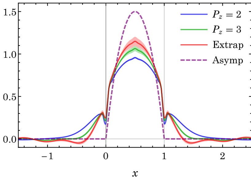
FIG. 3: Pion distribution amplitude at \mu = 2 GeV derived from the improved pion quasi-distribution amplitude of Eq. 13 and \delta m = 0.38\delta m_{1\text{-loop}} in Eq. 13 for P_z = 2 (blue) and 3 (green) (in units of 2\pi/L ) and extrapolation to infinite-momentum limit (red), along with the asymptotic form 6x(1-x) (dashed line).
