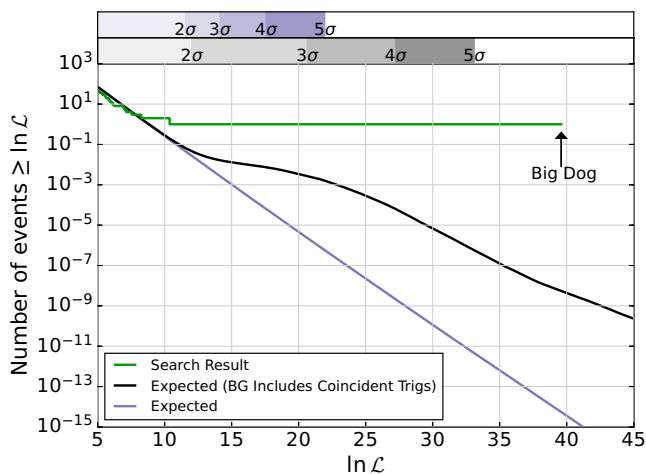
FIG. 11. Number of observed events as a function of log likelihood ratio in an analysis of S6 data beginning on September 14, 2010, at 23:58:48 UTC and ending on September 21, 2010, at 23:58:48 UTC. The Big Dog injection, found with a false alarm probability of 5.4 \times 10^{-9} ( 5.7\sigma ), is marked on the observed distribution (green). The black line represents the predicted number of events when observed events are included in the background model, while the blue line is the predicted number when the observed events are not included in the background model.
