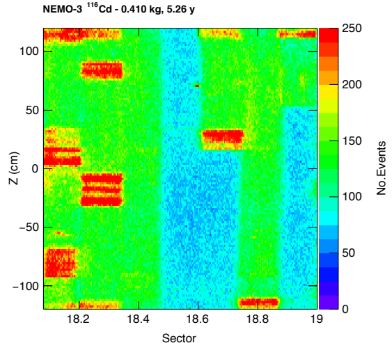
FIG. 4. Distribution of the track vertices on the source foil in the 1e channel. Three regions are defined based on the number of recorded events. The high activity regions, consistent with an excess of ^{234m}\text{Pa} on the surface of the foil, are rejected from the analysis.
