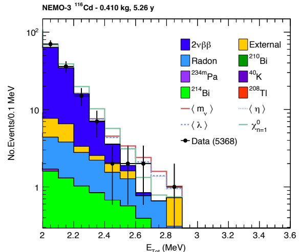
FIG. 10. Distribution of the total electron energy in two-electron channel above 2 MeV. The four open histograms stacked over the background model show the 90 % C.L. limits obtained on the 0\nu\beta\beta decay for different mechanisms (see text).
