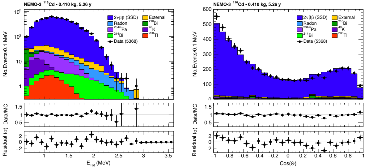
FIG. 6. Distribution of the total electron energy (left) and the angle between the two electron tracks (right) in the two-electron channel. Background contributions are due to external events, radon progeny in the tracker chamber, internal ^{208}\text{Tl} , ^{214}\text{Bi} and single- \beta emitters. The ratio of data events to the total Monte Carlo model and the residuals are shown in the bottom panels.
