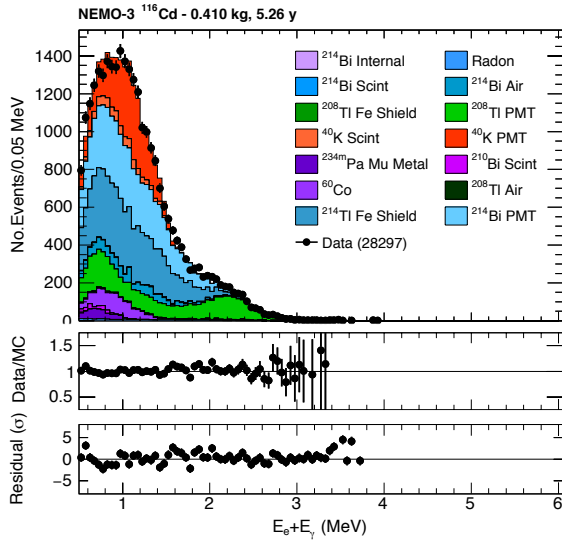
FIG. 1. Distribution of the total energy in the external \gamma - e channel. The external background is modelled with ^{40}\text{K} , ^{214}\text{Bi} , ^{228}\text{Ac}/^{212}\text{Bi}/^{208}\text{Tl} , ^{210}\text{Bi} , ^{60}\text{Co} and ^{234m}\text{Pa} in the PMT, scintillator surface, iron structure, iron shield and the air surrounding the detector. The ratio of data events to the total Monte Carlo model and the residuals are shown in the bottom panels.
