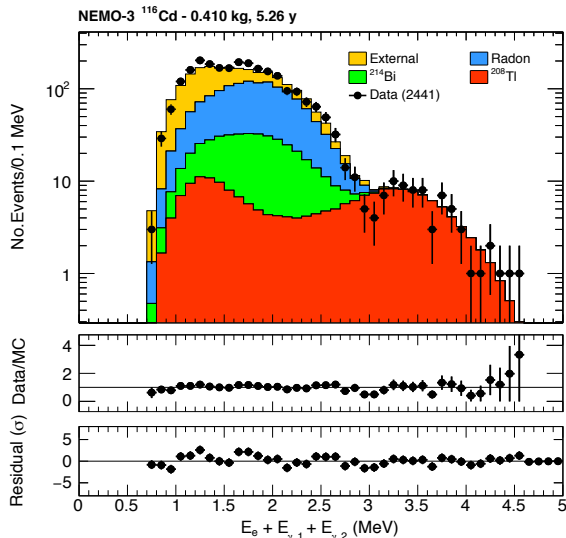
FIG. 3. Distribution of the total energy in the 1e2\gamma channel which provides the most sensitive measure of ^{208}\text{Tl} . The contribution from the external background, radon progeny in the tracking chamber and from ^{214}\text{Bi} are also considered. The ratio of data events to the total Monte Carlo model and the residuals are shown in the bottom panels.
