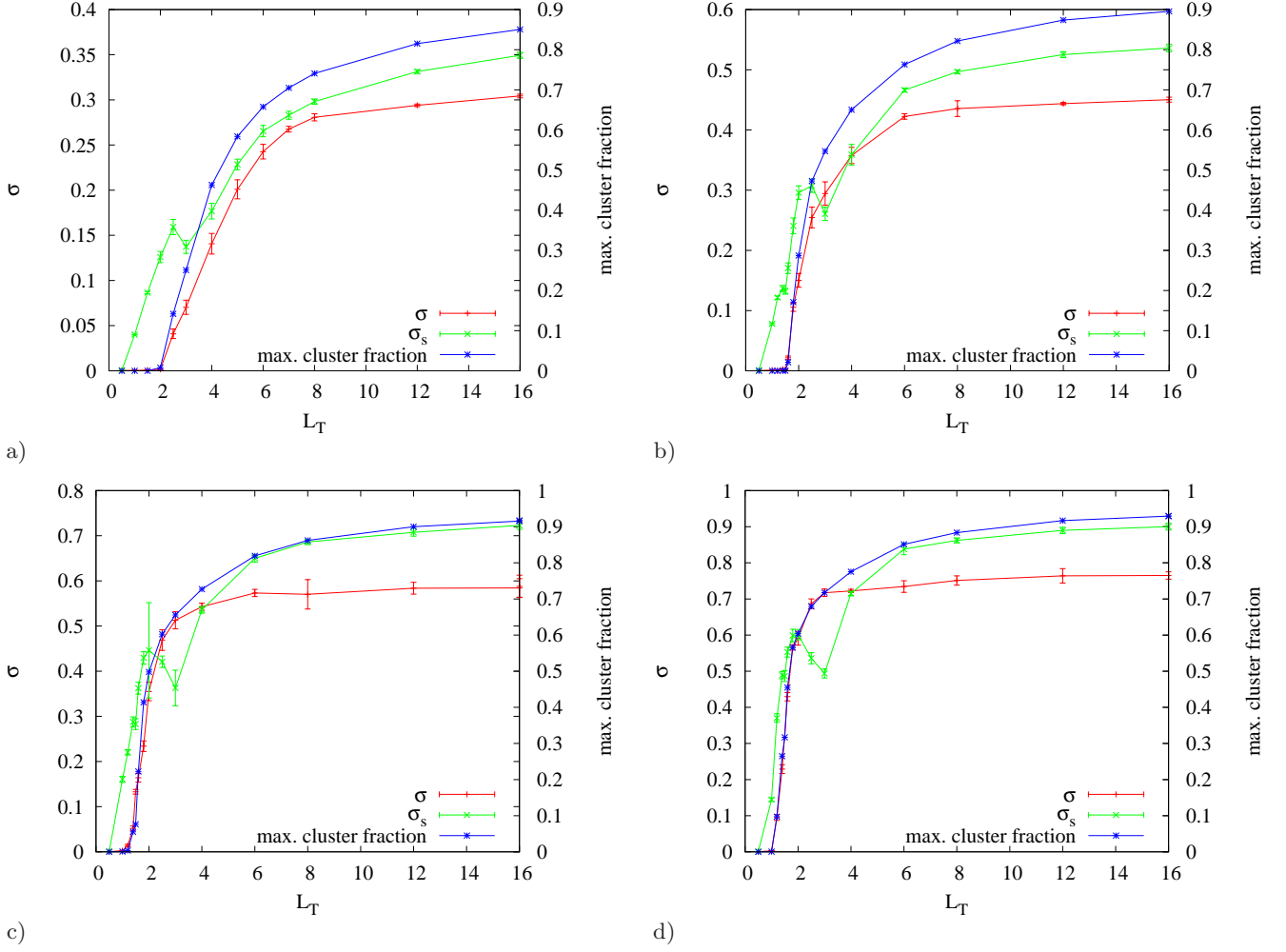
FIG. 9. Maximal cluster fraction, temporal and spatial string tensions \sigma and \sigma_s for 16^2 \times L_T volumes, density cutoff a) \rho = 6 , b) \rho = 8 , c) \rho = 10 , d) \rho = 12 , vortex lengths L_{max} = 1.7 , L_{min} = 0.3 .
