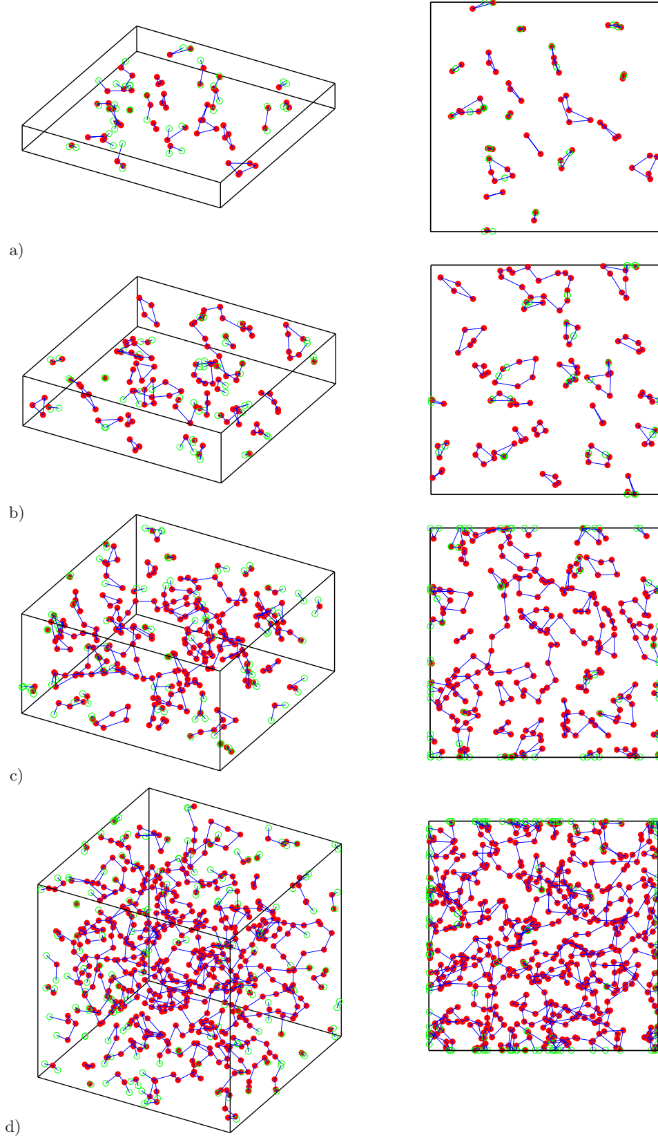
FIG. 11. 16^2 \times a) 2, b) 4, c) 8 and d) 16 sample configurations, density cutoff \rho = 4 , vortex lengths L_{max} = 1.7, L_{min} = 0.3 . The right-hand views are directly into the temporal direction.
