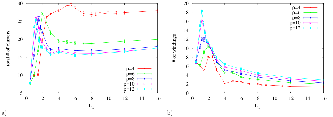
FIG. 10. a) Total number of vortex clusters and b) windings around the temporal dimension, for 16^2 \times L_T volumes, vortex lengths L_{max} = 1.7 , L_{min} = 0.3 .
