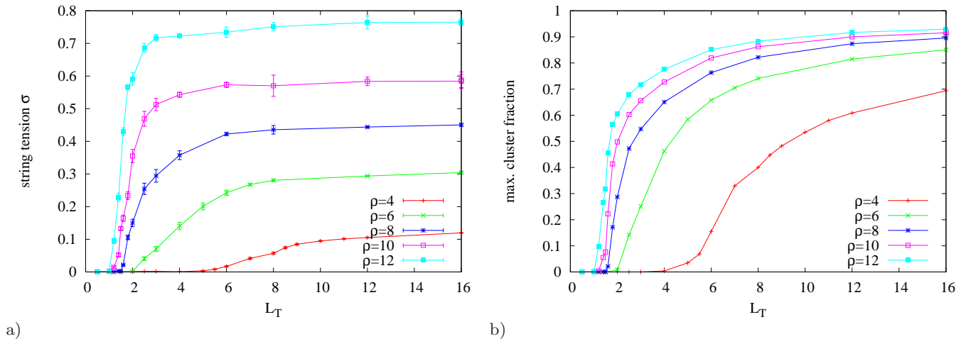
FIG. 7. String tension \sigma and maximal cluster fraction vs. time extent L_T of 16^2 \times L_T volumes, for different density cutoffs, vortex lengths L_{max} = 1.7, L_{min} = 0.3 .
