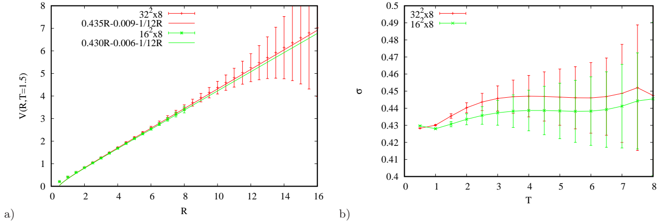
FIG. 16. a) Quark–anti-quark potential V(R, T = 1.5) and b) string tension \sigma saturating with temporal extent of Wilson loops T , for 16^2 \times 8 and 32^2 \times 8 volumes, density cutoff \rho = 8 , L_{max} = 1.7 and L_{min} = 0.3 .
