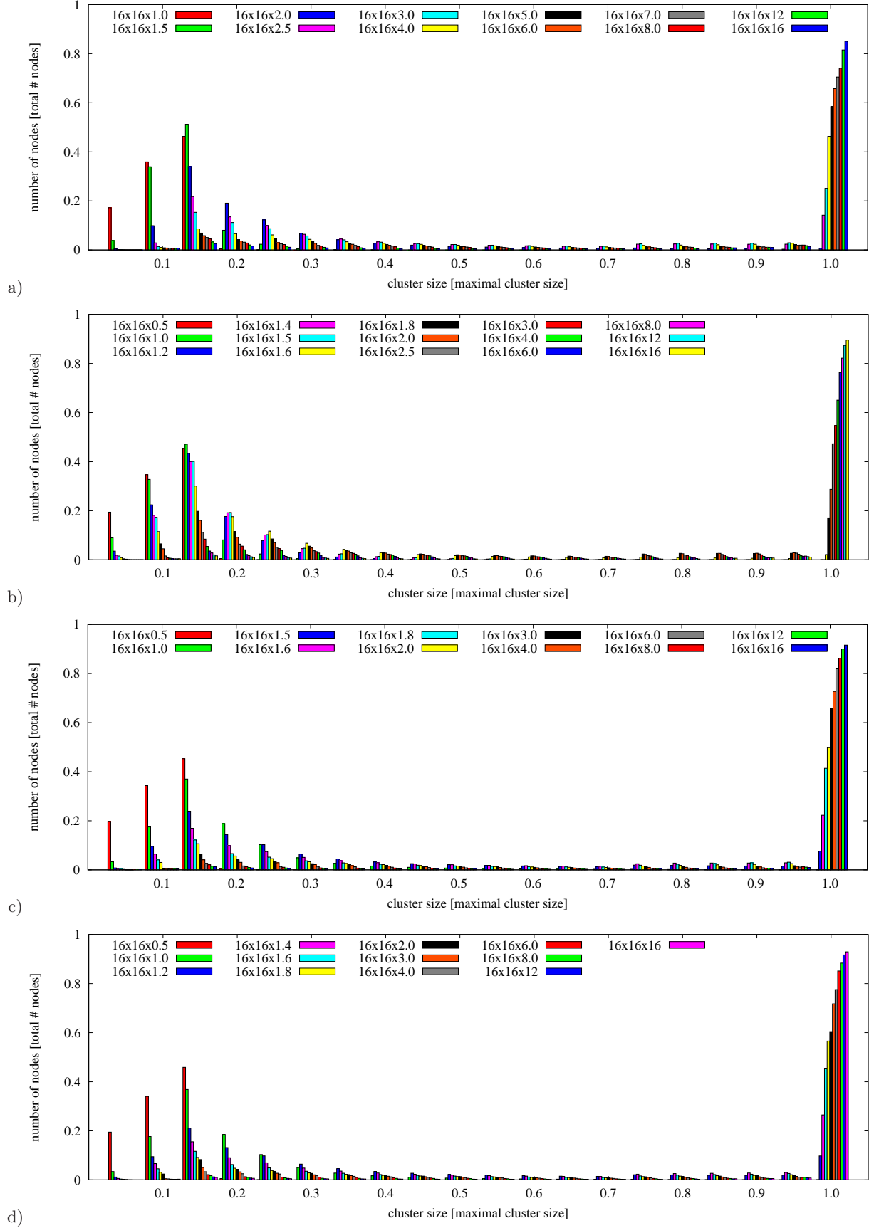
FIG. 8. Cluster size histograms for 16^2 \times L_T volumes, density cutoff a) \rho = 6 , b) \rho = 8 , c) \rho = 10 , d) \rho = 12 , vortex lengths L_{max} = 1.7 , L_{min} = 0.3 .
