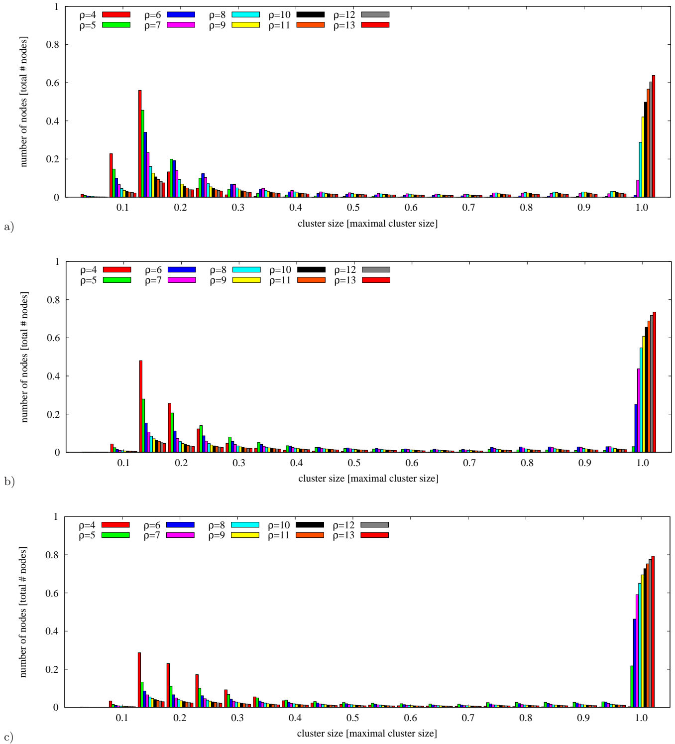
FIG. 13. Cluster size histograms for a) 16^2 \times 2 b) 16^2 \times 3 c) 16^2 \times 4 volumes and different density cutoffs \rho , vortex lengths L_{max} = 1.7 , L_{min} = 0.3 .
