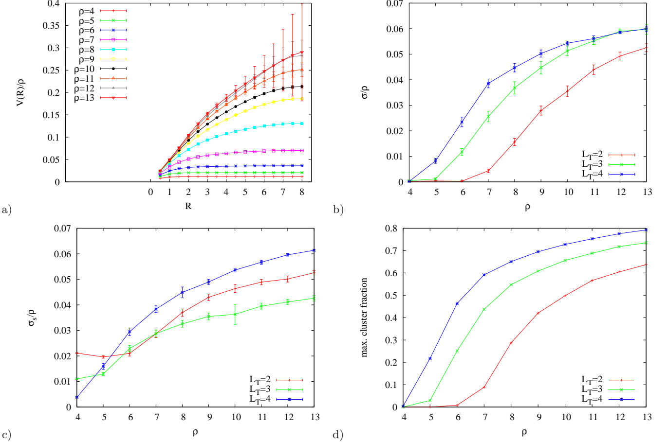
FIG. 12. a) Quark-anti-quark potentials on a 16^2 \times 2 volume, string tensions b) \sigma , c) \sigma_s and d) maximal vortex cluster fraction as a function of density cutoff \rho for 16^2 \times L_T volumes and vortex lengths L_{max} = 1.7, L_{min} = 0.3 .
