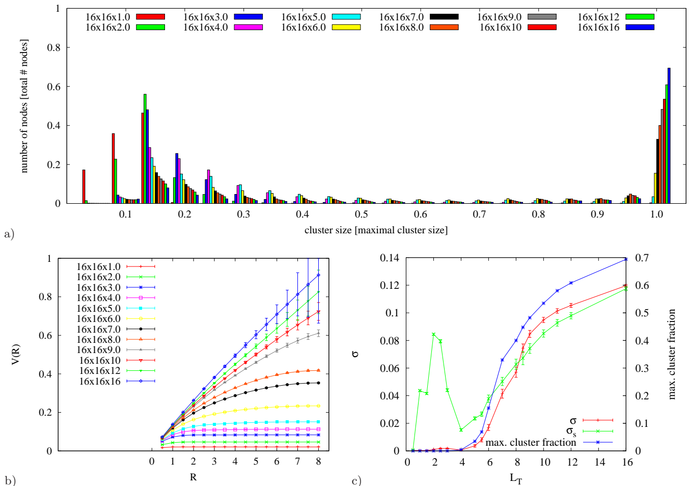
FIG. 6. a) Cluster size histogram, elucidating the percolation properties of the vortex structure: at high temperatures (small temporal lattice size, e.g. 16^2 \times 1 , 2 or 3) we find mainly small vortex clusters (histogram peaks on the left side), whereas for lower temperatures, most of the vortex material is found in clusters of maximal size (right peak), i.e. clusters percolating through the whole lattice. b) quark-anti-quark potentials and c) maximal cluster fraction ( i.e. , the fraction of vortex material in clusters of maximal size, the right peak of the histogram plot), temporal and spatial string tensions \sigma and \sigma_s for 16^2 \times L_T volumes, density cutoff \rho = 4 , vortex lengths L_{max} = 1.7 , L_{min} = 0.3 .
