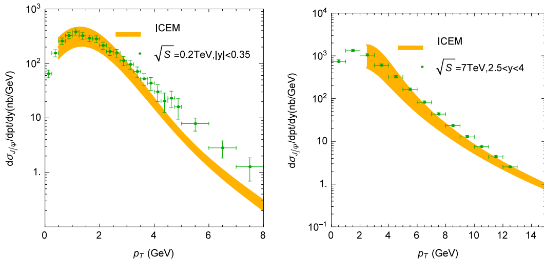
FIG. 2. Results for J/\psi production. The 0.2 TeV PHENIX data and 7 TeV LHCb data are taken from Ref. [19] and Ref. [22], respectively.
