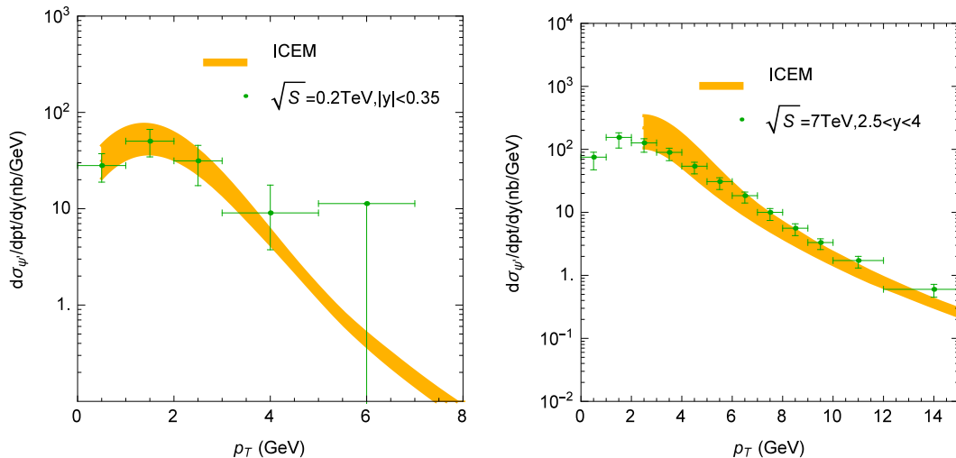
FIG. 3. Results for \psi' production. The 0.2 TeV PHENIX data and 7 TeV LHCb data are taken from Ref. [19] and Ref. [20], respectively.
