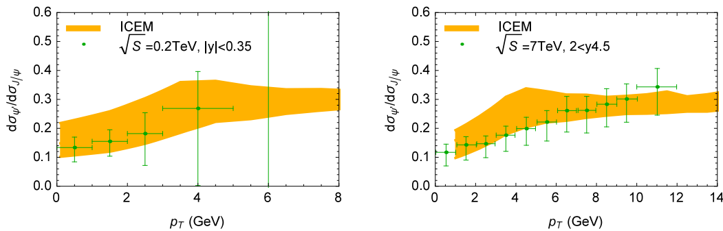
FIG. 4. Results for ratio of the \psi' production cross section to that of J/\psi . The 0.2 TeV PHENIX data and 7 TeV LHCb data are taken from Ref. [19] and Ref. [20], respectively.
