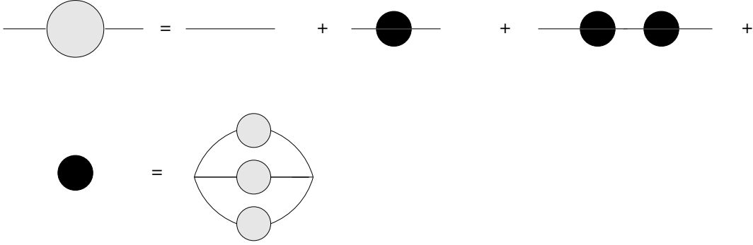
Figure 2: Equations that define the summation of the leading large N contributions, for the q = 4 case. The solid circle represents the one particle irreducible contributions. The dotted circle represents the full two point function. This is a graphical representation of the equations in (2.6).
