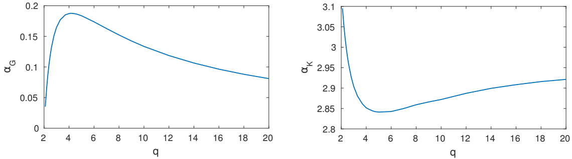
Figure 9: The functions \alpha_G(q) and \alpha_K(q) , computed by solving the Schwinger Dyson equations numerically for different values of q . The first three physical values are \alpha_G(2) = 0 , \alpha_G(4) \approx 0.1872 , and \alpha_G(6) \approx 0.1737 . Analytically, we know that \alpha_G behaves as 2/q at large q , and like \pi(q-2)/8 for q near two. \alpha_K never strays more than roughly five percent from the large q value of three.
