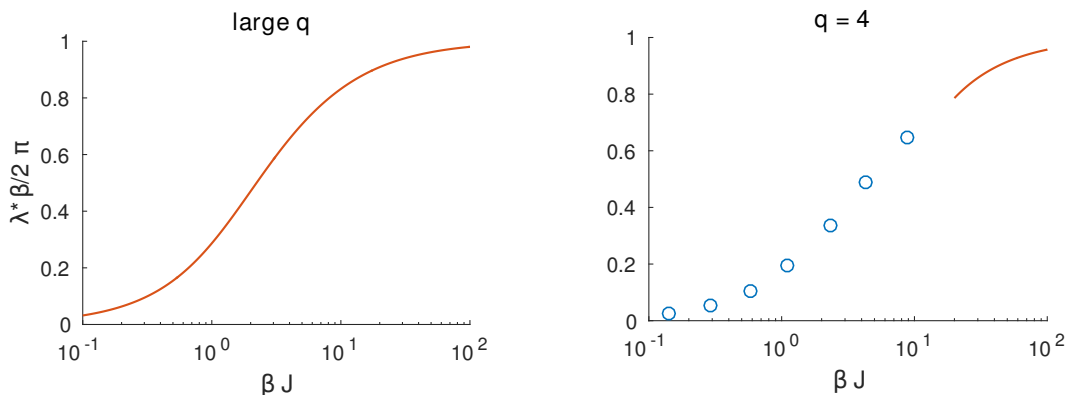
Figure 11: Left: the exact \lambda_L in the large q model. Right: \lambda_L for q = 4 . The red curve shows the formula (3.167) in a region of reasonable validity. The circles are exact values, obtained by numerically solving real-time Schwinger-Dyson equations and then diagonalizing the retarded kernel. Note that the x axis is \beta\mathcal{J} , not \beta J .
