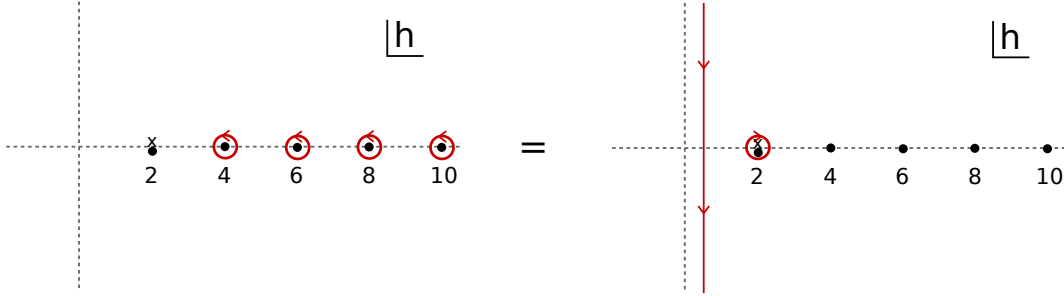
Figure 8: To continue the sum over residues to the chaos region, we first replace the k_c(h) by k_R(1-h) , and then pull the contour surrounding the poles back to the line 1/2 + is , picking up the double pole at h = 2 but no other poles. In this form the function can safely be continued. In addition we also have the original integral along h = 1/2 + is with the function k_c ; we leave this piece alone because it can already be continued.
