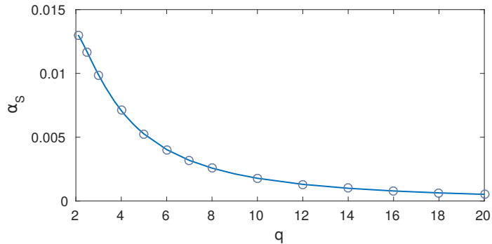
Figure 12: The coefficient of the Schwarzian action \alpha_S is plotted. The blue curve is the value given by the previously computed \alpha_G . The circles are values inferred from (5.182) and the numerical evaluation of the specific heat c . The agreement is a check that the Schwarzian action is correct nonlinearly, not just for small reparameterizations.
