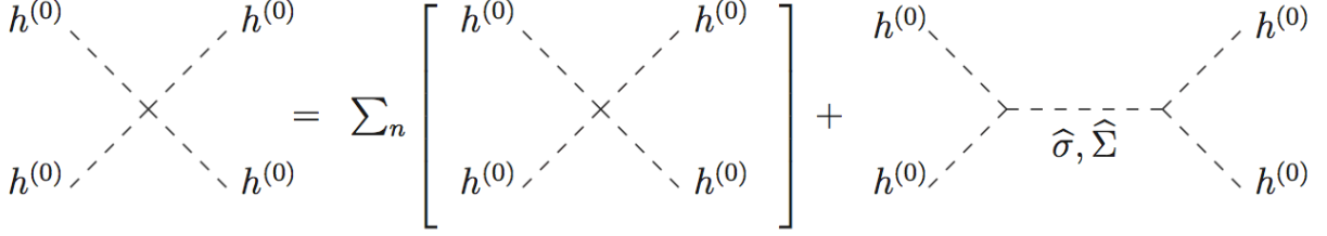
Figure 6: Matching of the low-energy and high-energy h^{(0)} four-point diagrams.
