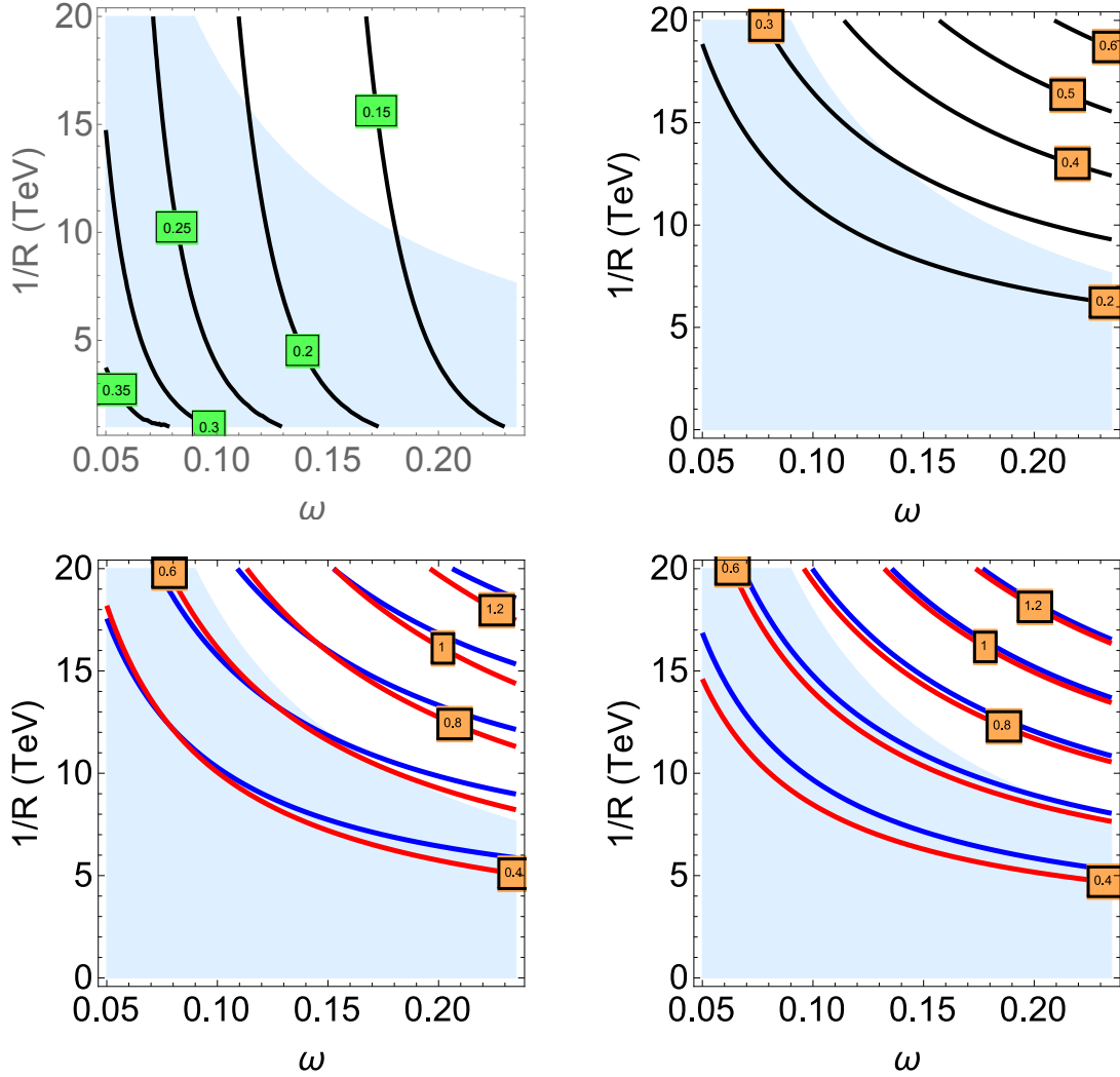
Figure 1: Contour plots of the most relevant loop-induced parameters. In light blue the region with gluino mass m_{\tilde{g}} < 1.8 TeV, in tension with LHC bounds (see Section 4.5). Mass labels are in TeV units. Upper left panel: Stop trilinear parameter normalized as X_t = A_t/m_Q . Upper right panel: Masses of the scalar left-handed tau \tilde{\tau}_L and the scalar left-handed tau neutrino \tilde{\nu}_\tau . Lower left panel: Masses of the lightest states of the stop \tilde{t}_1 and sbottom \tilde{b}_1 (red and blue lines respectively). Lower right panel: Masses of the heaviest states of the stop \tilde{t}_2 and sbottom \tilde{b}_2 (red and blue lines respectively).
