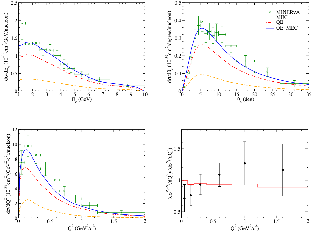
FIG. 16. (Color online) MINERνA flux-integrated differential \nu_e CCQE-like cross section vs. electron energy (top left) and electron angle (top right). The cross section vs. Q_{QE}^2 is shown in the bottom panel. Data are from [45].
