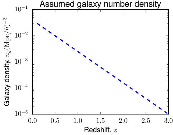
FIG. 2. The galaxy number density as a function of the redshift assumed in the Fisher matrix calculations. The function approximates the large galaxy count, low-accuracy redshift sample proposed for SPHEREx ( \tilde{\sigma}_z = 0.1 , cumulative) in Figure 10 of [6].
