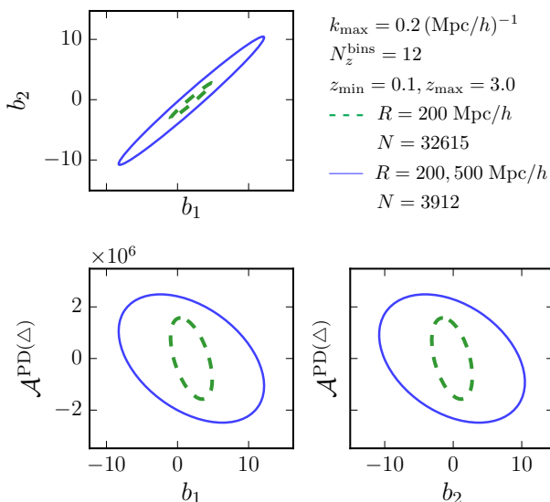
FIG. 5. Fisher forecast ellipses for two of (\mathcal{A}^{\text{PD}(\Delta)}, b_1, b_2) marginalized over the other and b_3 (which is not shown), assuming SPHEREx survey volume. The different colored ellipses represent different sets of sub-volume types: (i) dashed green – only one type of sub-volume with radius R = 200 Mpc/h, (ii) solid blue – two sizes of sub-volumes with R = 200, 500 Mpc/h in equal numbers. The Fisher constraints for these two cases are: \sigma(\mathcal{A}^{\text{PD}(\Delta)}) = 1.57 \times 10^6, 2.49 \times 10^6 ; \sigma(b_1) = 2.93, 10.2 ; \sigma(b_2) = 2.96, 10.6 . Note that while the two figures in the bottom panel look very similar, they have slightly different 1 - \sigma errors for b_1 and b_2 .
