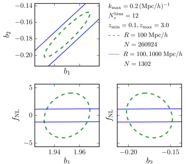
FIG. 4. Fisher forecast ellipses for two of (f_{\text{NL}}^{\text{local}}, b_1, b_2) marginalized over the other, assuming SPHEREx survey volume and other parameters given above in the figure. See Figure 2 for the assumed galaxy number density as a function of the redshift. The two different ellipses in each plot represent different choices for sub-volumes: (i) dashed green – only one type of sub-volume with radius R = 100 Mpc/h; this means that the total number of sub-volumes when dividing the whole survey is large ( N = 260924 ), (ii) solid blue – two sizes of sub-volumes with R = 100, 1000 Mpc/h in equal numbers (except for when the volume of a redshift bin is smaller than the volume of the larger sub-volume). The Fisher constraint for these two cases are: \sigma(f_{\text{NL}}) = 4.0, 1.2 ; \sigma(b_1) = 0.02, 0.16 and \sigma(b_2) = 0.03, 0.22 .
