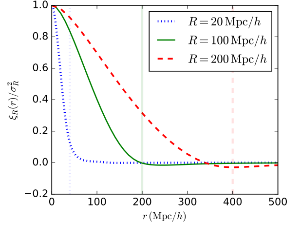
FIG. 3. The smoothed two-point correlation function \xi_R(r) as a function of the comoving distance r (normalized by \sigma_R^2 ), for three smoothing scales R = 200, 100, 20 Mpc/h. The vertical lines are r = 2R lines, and are plotted to show that the correlation is small for sub-volumes separated by r > 2R .
