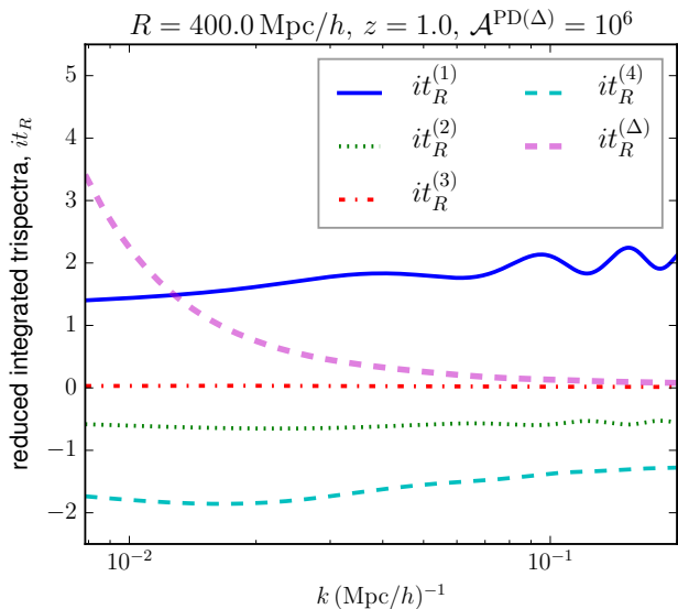
FIG. 1. The various reduced integrated trispectra, it_R^{(i)} (the expressions are given in Eq.(28) and Eq.(30)) for a large spherical sub-volume with radius R = 400 \text{ Mpc}/h at z = 1.0 . We have taken b_1 = 1.95, b_2 = -0.18, b_3 = -3.03 .
