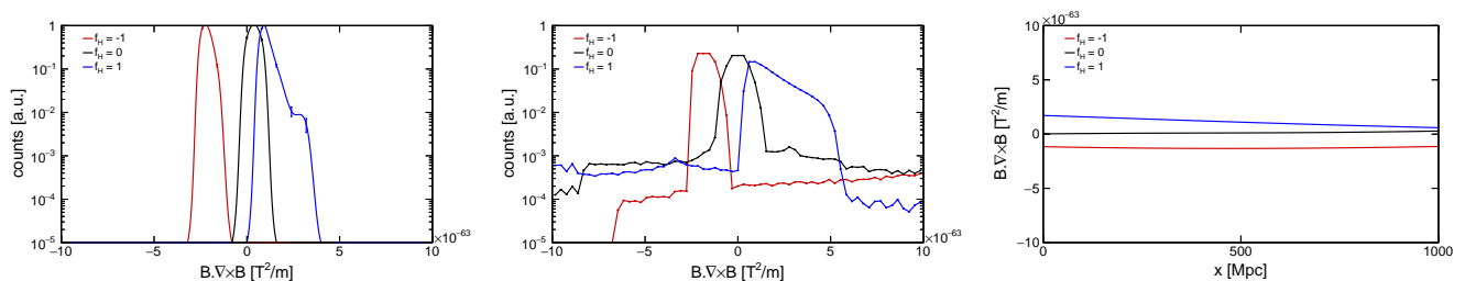
FIG. 5: Different current helicity measures for the three cases shown in Fig. 3, i.e. negative current helicity ( f_H = -1 , red), zero current helicity ( f_H = 0 , black) and positive current helicity ( f_H = +1 , blue). The left panel shows the total distribution of “current helicity”, defined as \mathbf{B} \cdot (\nabla \times \mathbf{B}) (which serves as a gauge-invariant proxy to the actual magnetic helicity), in the whole simulation box, normalized to 1. In the center panel the same measure is shown, however restricted only to the line of sight and the neighboring cells. Finally, the right panel shows the helicity values along the line of sight from the source (at x = 0 Mpc) to the observer (at x = 1000 Mpc).
