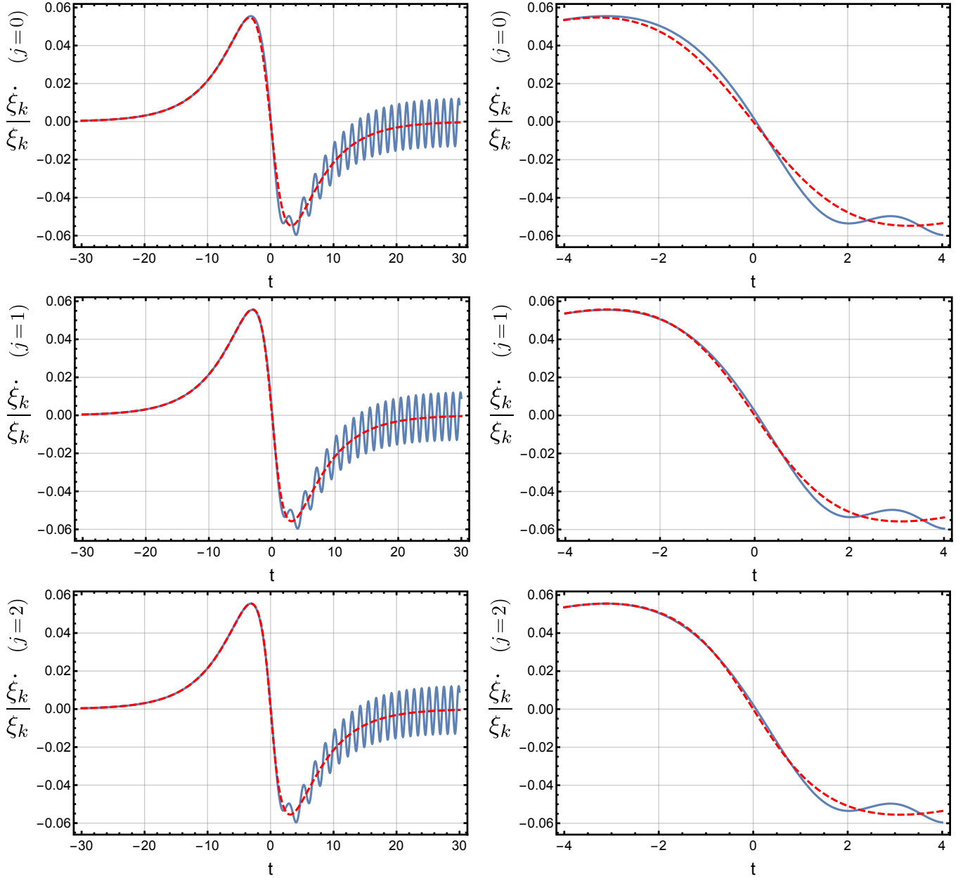
FIG. 6: Plots of approximation (86), the time derivative form of (85) as a ratio, by comparing \dot{\xi}_k/\xi_k (blue-solid line) with the adiabatic function V_k^{(j)} = -\dot{W}_k^{(j)}/(2W_k^{(j)}) (red-dashed line), for the first three orders of the adiabatic expansion, considering a time-dependent single-pulse electric field given by E_{\parallel}(t) = E_0 \text{sech}^2(at) with the same pulse parameters as for Figure 4. The left-hand panels show the time-evolution over a wide range of t , and the right-hand panels zoom in on the vicinity of the pulse. The approximate (red-dashed) curves accurately describe the averaged time evolution, but miss the late-time oscillations, which are more pronounced than those in Figures 4 and 5 because they are effectively the derivatives of those small oscillations.
