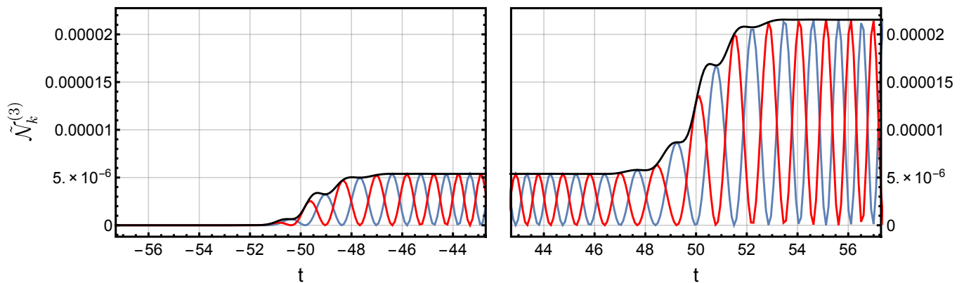
FIG. 12: The time evolution of the adiabatic particle number (91) (black-solid line), and its components, the first (blue-solid line) and second (red-solid line) terms on the right-hand-side of (91), at the optimal order of the adiabatic expansion, for the time-dependent double-pulse electric field given by (89) with E_0 = 0.25, a = 0.1, b = 50 , longitudinal momentum k_{\parallel} = 2.51555 , and transverse momentum k_{\perp} = 0 , in units with m = 1 . The longitudinal momentum was selected to correspond to maximum constructive interference, with the final value being 4 times the intermediate plateau value between the two pulses. At intermediate times, notice the phase difference of the oscillatory components of (91), which remarkably sum to a smooth evolution of the adiabatic particle number.
