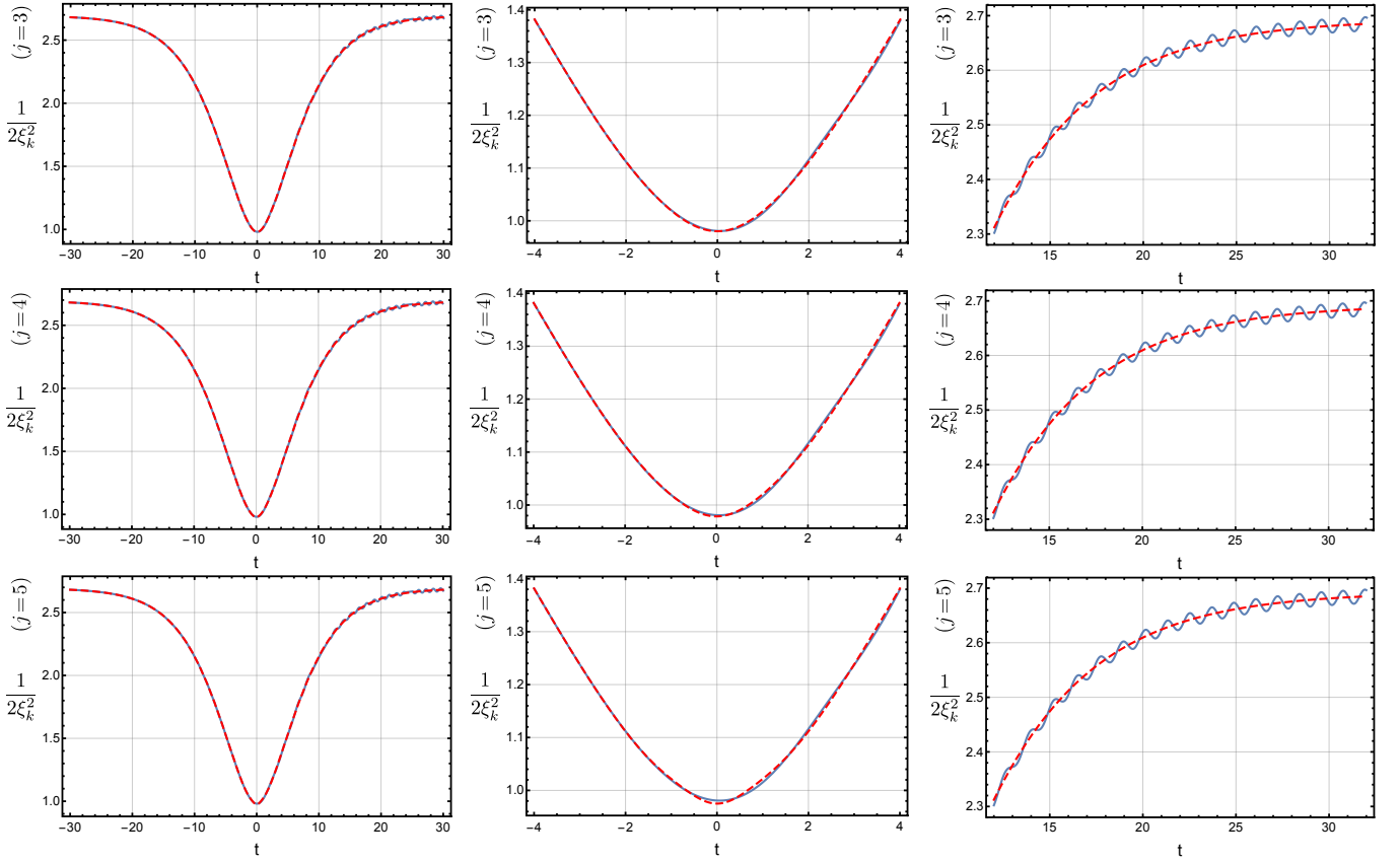
FIG. 5: As in Figure 4 but with plots of the next three adiabatic orders, j = 3, 4, 5 for the adiabatic approximation (85) of 1/(2\xi_k^2) (blue-solid line) compared to the adiabatic expansion function W_k^{(j)} (red-dashed line), considering a time-dependent single-pulse electric field given by E_{\parallel}(t) = E_0 \text{sech}^2(at) with the magnitude E_0 = 0.25 , a = 0.1 , longitudinal momentum k_{\parallel} = 0 , and transverse momentum k_{\perp} = 0 , in units with m = 1 . The central panels zoom in on time-scales near the pulse, while the right-hand panels zoom in on the late-time behavior. Notice that the deviations of the approximation from the exact form are typically very small, capturing well the averaged time dependence except near the peak of the pulse, and except for tiny oscillations about the average value at late times. The optimal order is reached at j = 3 , after which the deviations begin to grow again.
