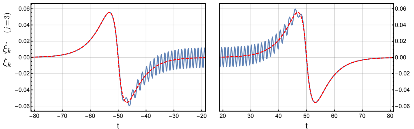
FIG. 10: Zoomed-in view of the right subplot of Figure 8, plotted for a closer examination of the approximation (86) in the vicinity of the pulse centers ( t = \pm 50 ), for the case of maximum destructive interference.
