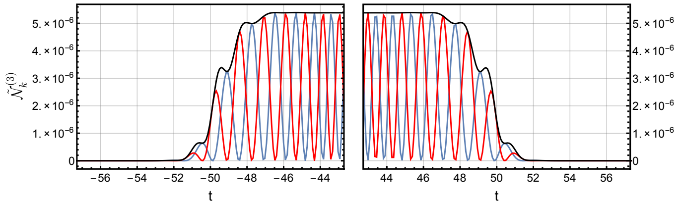
FIG. 13: The time evolution of the adiabatic particle number (91) (black-solid line), and its components, the first (blue-solid line) and second (red-solid line) terms on the right-hand-side of (91), at the optimal order of the adiabatic expansion, for the time-dependent double-pulse electric field given by (89) with E_0 = 0.25, a = 0.1, b = 50 , longitudinal momentum k_{\parallel} = 2.49887 , and transverse momentum k_{\perp} = 0 , in units with m = 1 . The longitudinal momentum was selected to correspond to maximum destructive interference, with vanishing final particle number at future infinity. At intermediate times, notice the phase difference of the oscillatory components of (91), which remarkably sum to a smooth evolution of the particle number.
