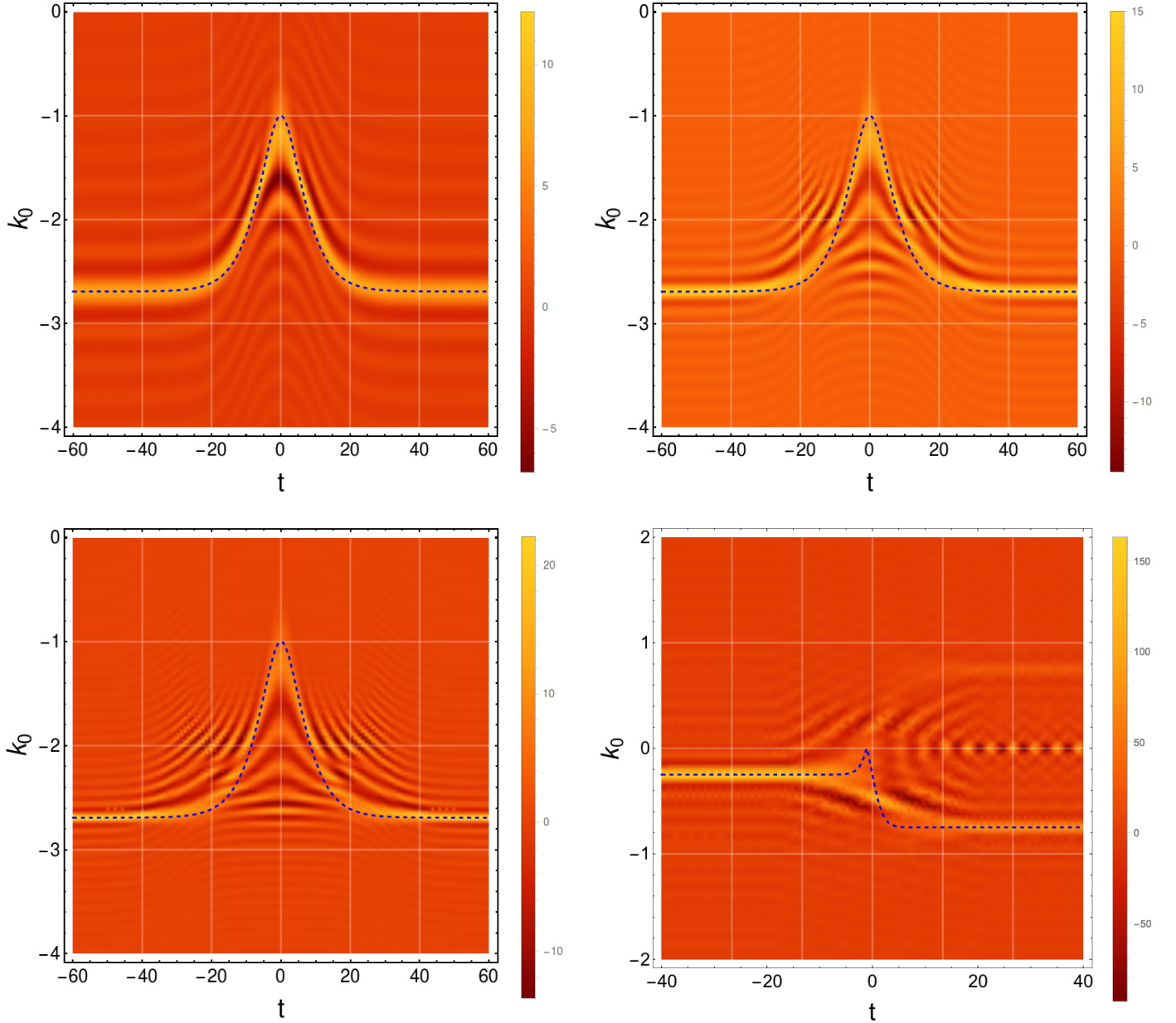
FIG. 2: Density plots with respect to t , and the conjugate energy variable k_0 , of the spectral function \mathcal{W}_k(t, k_0) for a time-dependent single-pulse electric field given by E(t) = E_0 \text{sech}^2(at) , obtained by numerically evaluating equation (54) over the range T = -T_0 to T = +T_0 , utilizing the exact solution \xi_k(t) to the mode-oscillator equation found in the Appendix V. The upper left, upper right and lower left subplots are plotted with the magnitude E_0 = 0.25 , a = 0.1 , longitudinal momentum k_{\parallel} = 0.25 , and transverse momentum k_{\perp} = 0 , in units with m = 1 , with the upper left plot integrated with T_0 = 20 , the upper right plot integrated with T_0 = 40 , and the lower left subplot integrated with T_0 = 60 . The lower right subplot is plotted for the physically unrealistic case with m = 0 , E_0 = 0.5 , k_{\parallel} = 0.25 , k_{\perp} = 0 , as discussed in [58], and integrated with T_0 = 40 . In each subplot the dominant features of \mathcal{W}_k(t, k_0) are well matched by the negative effective frequency, -\omega_k(t) (2) (blue-dashed line), artificially plotted over each density subplot for direct comparison.
