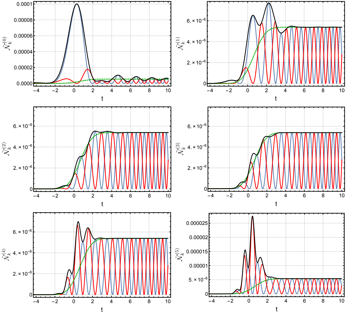
FIG. 11: The time evolution of the adiabatic particle number (91) (black-solid line), and its components, the first (blue-solid line) and second (red-solid line) terms on the right-hand-side of (91), for the first six orders of the adiabatic expansion, considering a time-dependent single-pulse electric field given by E(t) = E_0 \text{sech}^2(at) with E_0 = 0.25, a = 0.1 , longitudinal momentum k_{\parallel} = 0 , and transverse momentum k_{\perp} = 0 , in units with m = 1 . Berry's universal form for the particle number is plotted as green-dashed lines. Notice that each of the components (blue and red curves) is highly oscillatory, and out of phase, especially at late times, but the sum is smooth except in the vicinity of the pulse. Also note the difference in scales in the various sub-plots. The deviations decrease dramatically as the optimal order ( j = 3 ) is approached, and then grow again as this order is passed. Further features are discussed in the text.
