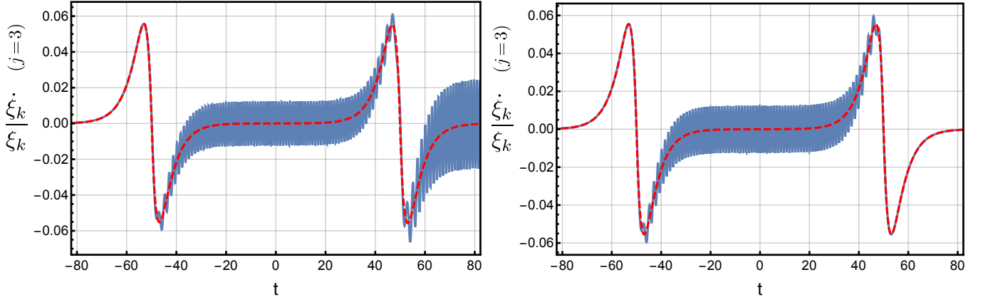
FIG. 8: Plots of the approximation (86) at the optimal truncation order ( j = 3 ), for the time derivative form of (85) as a ratio, by comparing \dot{\xi}_k/\xi_k (blue-solid line) and V_k^{(j)} = -\dot{W}_k^{(j)}/2W_k^{(j)} (red-dashed line), for a time-dependent electric field given by (89) with the magnitude E_0 = 0.25 , a = 0.1 , b = 50 , and transverse momentum k_\perp = 0 , in units with m = 1 . The longitudinal momentum k_\parallel was selected to correspond to maximum constructive ( k_\parallel = 2.51555 for left subplot), and maximum destructive interference ( k_\parallel = 2.49887 for right subplot) in the particle number at future infinity [37, 57]. In the maximum constructive case [left panel], the oscillations introduced after each pulse interfere to increase in magnitude, and double in scale. In the maximum destructive case [right panel], the oscillations introduced by the first and second pulse interfere to completely cancel.
