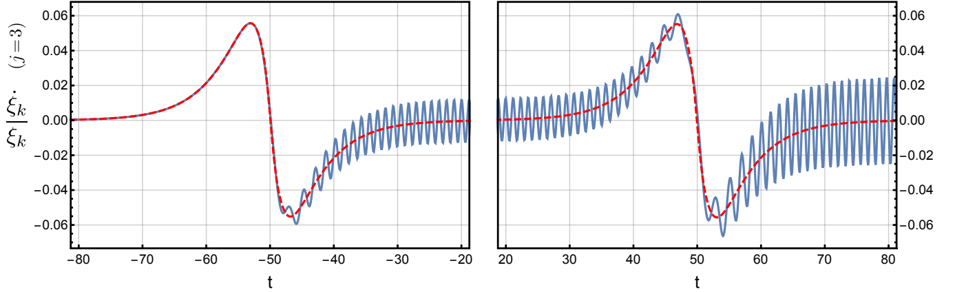
FIG. 9: Zoomed-in view of the left subplot of Figure 8, plotted for a closer examination of the approximation (86) in the vicinity of the pulse centers ( t = \pm 50 ), for the case of maximum constructive interference.
