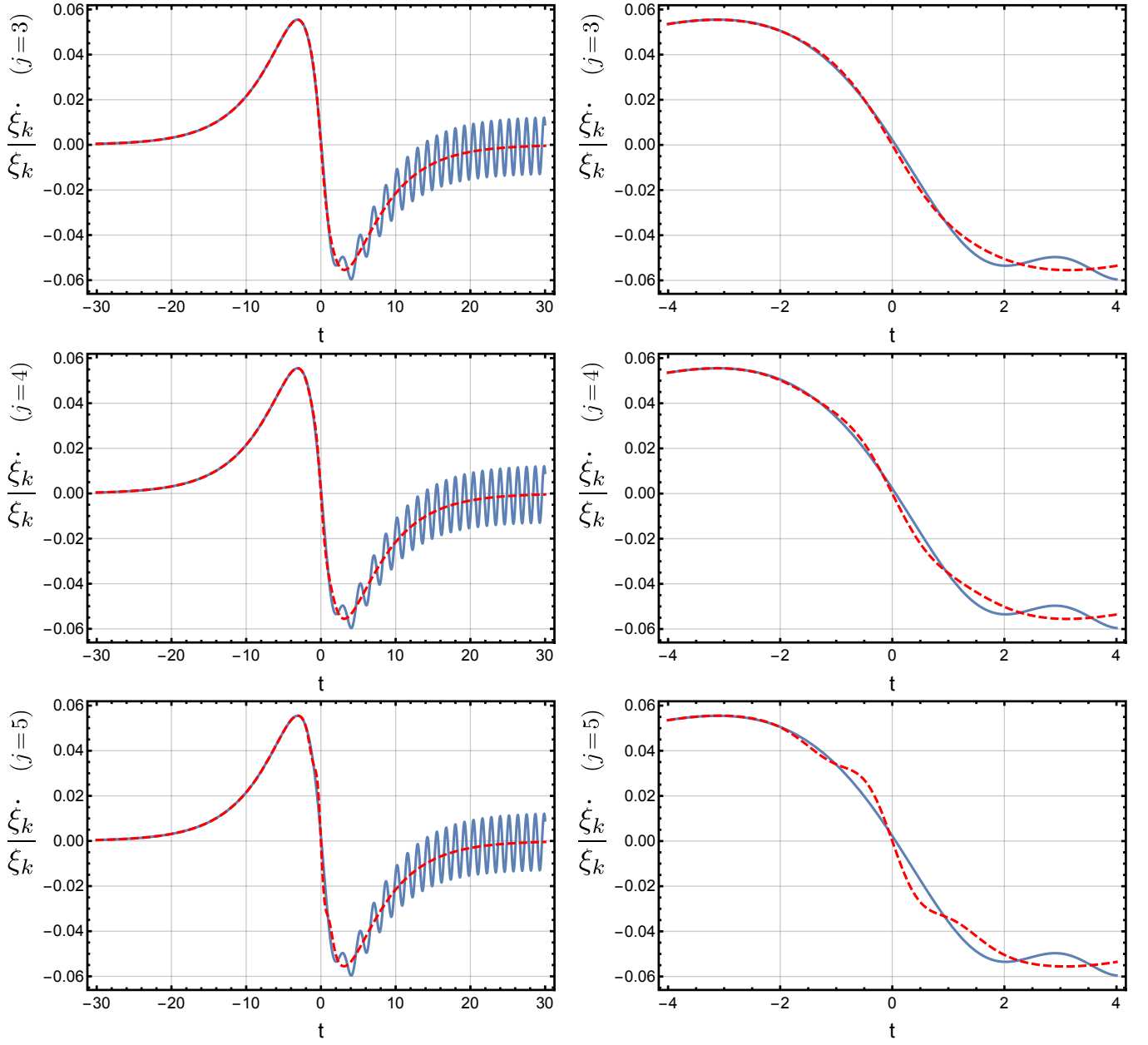
FIG. 7: As in Figure 6, but with plots of the next three adiabatic orders, j = 3, 4, 5 , showing the approximation (86), the time derivative form of (85) as a ratio, by comparing \dot{\xi}_k/\xi_k (blue-solid line) with the adiabatic function V_k^{(j)} = -\dot{W}_k^{(j)}/(2W_k^{(j)}) (red-dashed line), considering a time-dependent single-pulse electric field given by E_{\parallel}(t) = E_0 \text{sech}^2(at) with the same pulse parameters as for Figure 4. The left-hand panels show the time-evolution over a wide range of t , and the right-hand panels zoom in on the vicinity of the pulse. The approximate (red-dashed) curves accurately describe the averaged time evolution, but miss the late-time oscillations, which are more pronounced than those in Figures 4 and 5 because they are effectively the derivatives of those small oscillations. The optimal truncation order is at j = 3 , after which the deviations begin to increase again.
