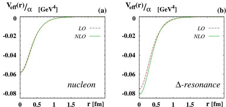
FIG. 2: The effective potential V_{\text{eff}}(r) normalized with respect to the polarizability \alpha for (a) nucleon, and (b) \Delta as function of r in LO and NLO order of the large- N_c expansion after the rescaling in Eq. (32), i.e. V_{\text{eff}}(r) is normalized according to (23) with respect to the physical value of the respective baryon mass.
