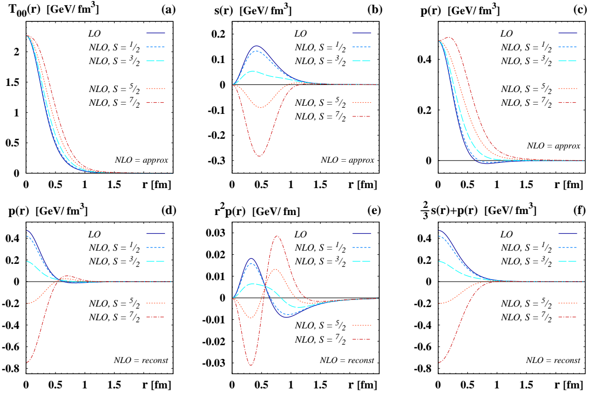
FIG. 1: EMT densities from the Skyrme model as functions of r . The LO results are valid for any S = I in the large- N_c limit. The estimates of NLO corrections in the 1/N_c -expansion are shown for states with the quantum numbers S = I = \frac{1}{2}, \frac{3}{2}, \frac{5}{2}, \frac{7}{2} . The Figures show: (a) energy density T_{00}(r) , (b) shear forces s(r) , (c) pressure p(r) with approximate NLO corrections, (d) p(r) with NLO corrections reconstructed according to (30), (e) same as Fig. 1d but for r^2 p(r) , (f) the local stability criterion (18). The NLO results in the upper panel, Figs. 1a–c, are estimated by simply evaluating the NLO expressions with the LO soliton profile, which yields unacceptable results especially for p(r) which are at variance with Eq. (14). The results in the lower panel, Figs. 1d–f, are obtained with the pressure reconstructed according to (30) which satisfies Eq. (14). Finally, Fig. 1f shows that the results for S = I = \frac{1}{2}, \frac{3}{2} , which correspond to nucleon and \Delta , comply with the local stability criterion (18). In contrast to this, states with the exotic quantum numbers S = I \geq 5/2 do not satisfy (18), i.e. in this way the rotating soliton approach explains why they are not realized in nature.
