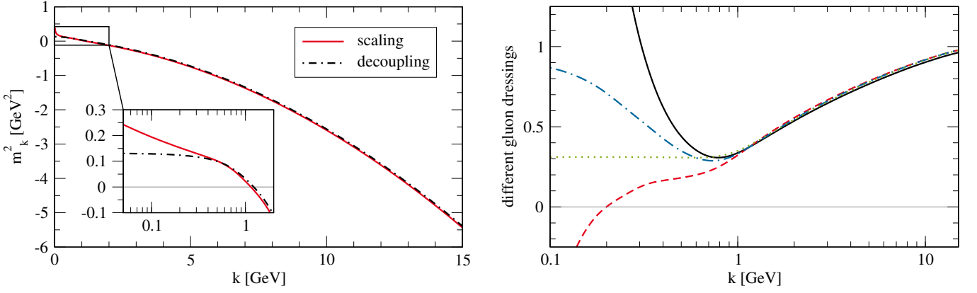
FIG. 10. Left: Gluon mass parameter m_k^2 = \Gamma_{AA,k}^{(2)}(p=0) over k . Right: Possible choices for the scaling prefactor in the gluon regulator: Z_{A,k}(k) (black, solid), \bar{Z}_{A,k}(k) (red, dashed), \hat{Z}_{A,k}(k) (blue, dot-dashed) and \tilde{Z}_{A,k} (green, dotted) as defined in (E3) and (E5). Independence of the results from the above choice has been checked explicitly.
