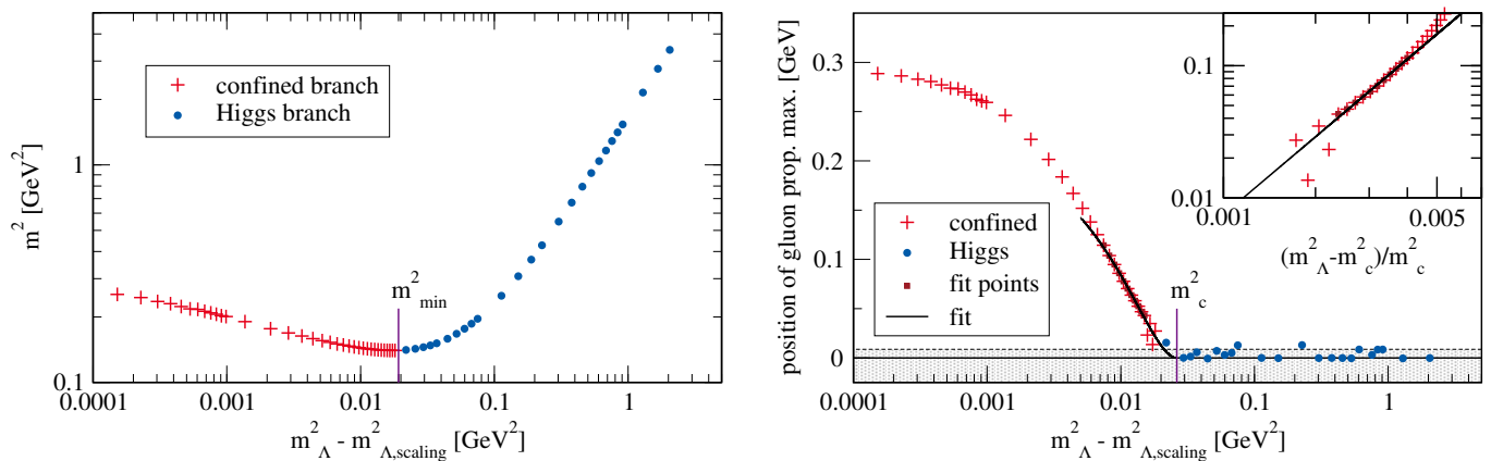
FIG. 9. Left: Gluon mass gap as a function of the gluon mass parameter m_\Lambda^2 - m_{\Lambda, \text{scaling}}^2 , where m_{\Lambda, \text{scaling}}^2 denotes the gluon mass parameter that yields the scaling solution. Right: Momentum value at which the gluon propagator assumes its maximum, as a function of the gluon mass parameter m_\Lambda^2 - m_{\Lambda, \text{scaling}}^2 . The inset exposes the power law behaviour of the gluon propagator maximum in the vicinity of the transition region, see (33). Both plots were obtained from our numerically less-demanding 1D approximation. We have repeated this analysis in the transition regime from Higgs-type to confinement branch also with the best approximation and find the same behaviour. The shaded area marks momentum scales that are not numerically resolved in the present work. The points in this region rely on a generic extrapolation.
