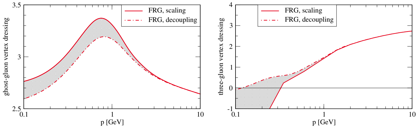
FIG. 5. Ghost-gluon vertex (left) and three-gluon (right) vertex dressing functions Z_{A\bar{c},\perp}(p, p, -\frac{1}{2}) and Z_{A^3,\perp}(p, p, -\frac{1}{2}) in the symmetric point configuration. More momentum configurations and comparisons to Dyson-Schwinger and lattice results can be found in Figs. 11-13. In contrast to Fig. 3, the decoupling dressings are normalised to the scaling solution in the UV.
