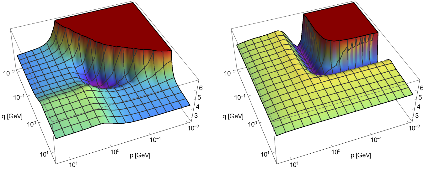
FIG. 11. Left: Four-gluon vertex dressing function Z_{A^4,\perp}(p, q, 0) in the tadpole configuration. The angular dependence is small compared to the momentum dependence. Right: Four-gluon tadpole configuration evaluated in the symmetric point approximation, showing a quantitative and qualitative deviation from the full calculation.
