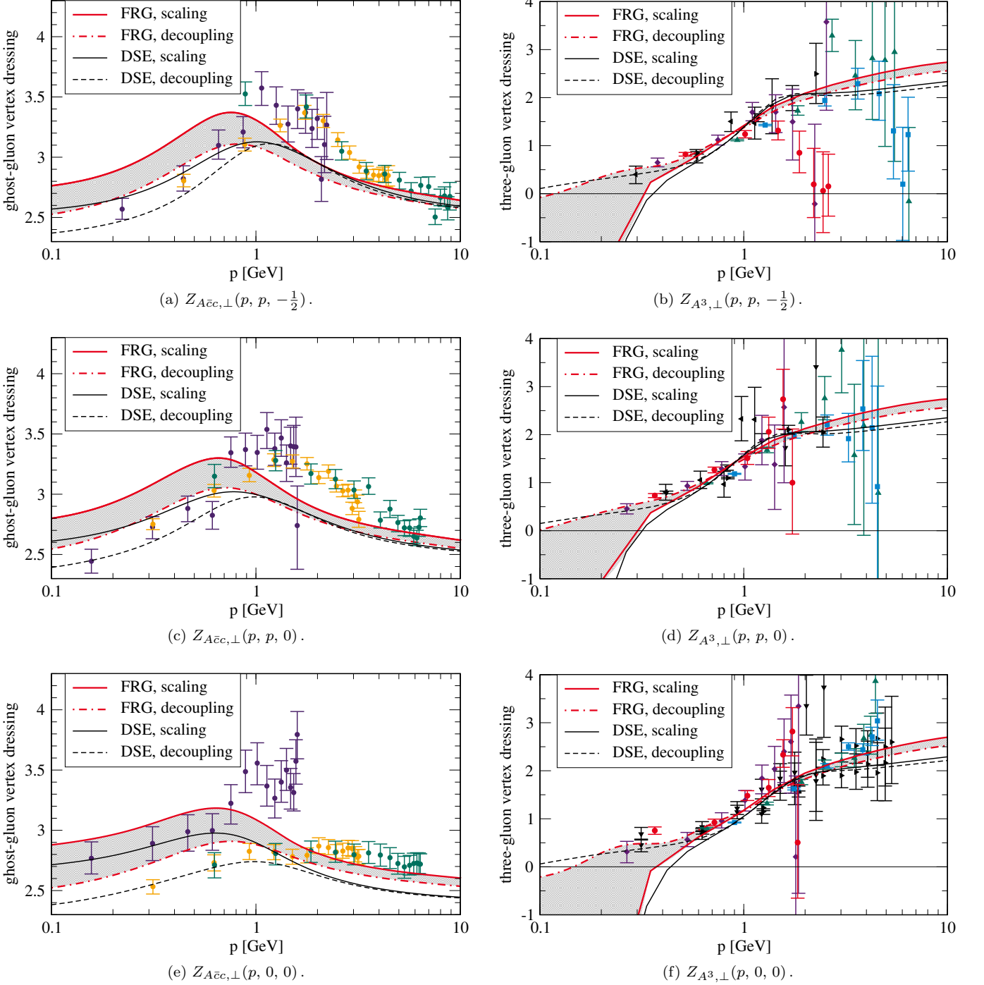
FIG. 13. Left: Ghost-gluon vertex dressing function Z_{A\bar{c}c,\perp}(p, q, \cos\angle(p, q)) in comparison to SU(2) lattice [105–107] and DSE results [44, 89]. The lattice results are obtained from N = 32^4 lattices. The magenta/orange/green points (colour online) correspond to \beta \in \{2.13, 2.39, 2.60\} and lattice spacing a^{-1} \in \{0.8 \text{ GeV}, 1.6 \text{ GeV}, 3.2 \text{ GeV}\} , respectively. Right: Three-gluon vertex dressing function Z_{A^3,\perp}(p, q, \cos\angle(p, q)) compared with SU(2) lattice [105–107] and Dyson-Schwinger [47] results. The coloured lattice points are taken from [105, 106] and correspond to \beta \in \{2.2, 2.5\} and different lattice sizes 1.4 \text{ fm} < L < 4.7 \text{ fm} . The lattice results shown in black are based on [105, 106] but stem from [107]. These are gained from N \in \{24^4, 32^4\} lattices with \beta \in \{2.13, 2.39, 2.60\} and lattice spacing a^{-1} \in \{0.8 \text{ GeV}, 1.6 \text{ GeV}, 3.2 \text{ GeV}\} . The comparison with SU(2) lattice simulations is justified since the propagators of SU(2) and SU(3) Yang-Mills theory agree well for a large range of momenta [108, 109] after a respective normalisation in this regime. We rescaled all DSE results such that they match the scaling solution in the symmetric point configuration at p = 2 \text{ GeV} . Note that the scaling and decoupling solutions differ in the UV just due to the different field renormalisations, cf. Fig. 3. The physically relevant couplings, given by (20), agree in the UV.
