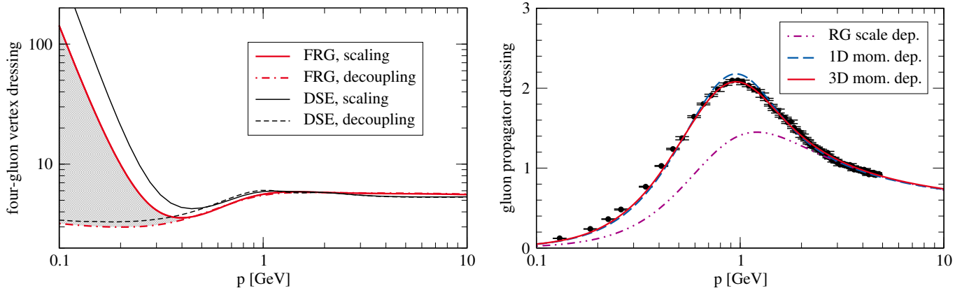
FIG. 6. Left: Four-gluon vertex dressing function as defined in (10) at the symmetric point in comparison to Dyson-Schwinger computations [39]. We normalised all curves to match the scaling result at p = 2 GeV. Right: Gluon propagator dressings obtained with different momentum approximations, see Sec. IV B for details.
