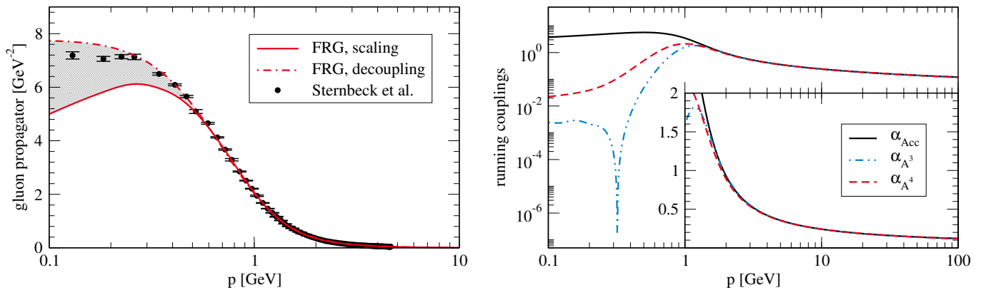
FIG. 4. Left: Gluon propagator in comparison to the lattice results from [65]. Right: Effective running couplings defined in (20) as obtained from different Yang-Mills vertices as function of the momentum.
