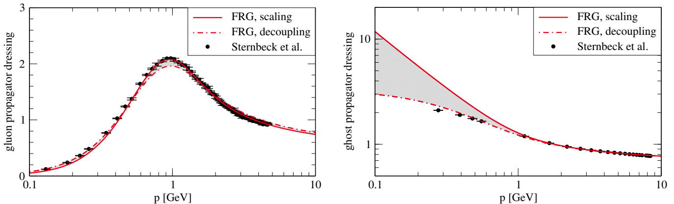
FIG. 3. Gluon dressing 1/Z_A (left) and ghost dressing 1/Z_c (right) in comparison to the lattice results from [65]. The scale setting and normalisation procedures are described in App. F.
