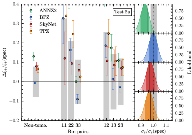
Figure 13. A comparison of the relative agreement of the n(z) estimates for ANNZ2, BPZ, SKYNET, and TPZ to the weighted 'deep' spectroscopic galaxy sample, showing the same information as described in Fig. 12.
