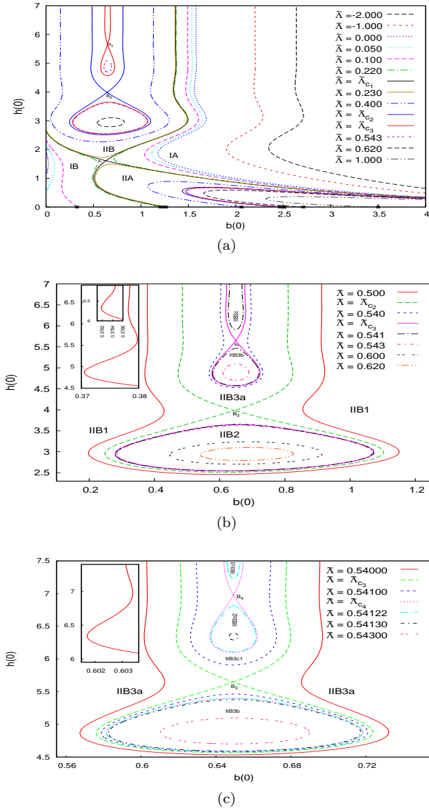
FIG. 1. (color online) Fig. (a) depicts the phase diagram of the theory for the vector field at the center of the star b(0) and the scalar field at the center h(0) for different values of the cosmological constant \tilde{\Lambda} in the range \tilde{\Lambda} = -2.000 to \tilde{\Lambda} = +1.000 . The points B_1 , B_2 , B_3 and B_4 represent the four bifurcation points. The entire region depicted in the phase diagram in Fig. (a) is divided into four regions IA, IB and IIA, IIB in the vicinity of B_1 . The region IIB of the phase diagram shown in Fig. (a) is separately depicted in details in Fig. (b). The region IIB of the phase diagram is subdivided into three regions IIB1, IIB2 and IIB3 in the vicinity of B_2 . The region IIB3 is further subdivided into the regions IIB3a, IIB3b and IIB3c in the vicinity of B_3 . Similarly the region IIB3c is subdivided in to the regions IIB3c1, IIB3c2 and IIB3c3 in the vicinity of B_4 . The asterisks shown in Fig. (a), corresponding to h(0) = 0 , represent the transition points from the boson stars to the boson shells. The Figure shown in the inset in Fig. (b) represents a part of the phase diagram with better precision.
