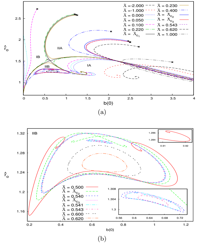
FIG. 2. (color online) Fig.(a) shows a plot of the vector field at the center of the star b(0) versus the radius \hat{r}_o of the boson star. The point B_1 corresponds to the bifurcation point and the entire region depicted in Fig. (a) is divided into four regions IA, IB and IIA, IIB in the vicinity of B_1 . The region IIB shown in Fig. (a) is separately depicted in details in Fig. (b). The asterisks shown in Fig. (a) represent the transition points from the boson stars to the boson shells. The spiral behavior of the solutions is visible in the regions IA and IIB. The Figure shown in the inset in Fig. (b) represents a part of the region IIB with better precision.
