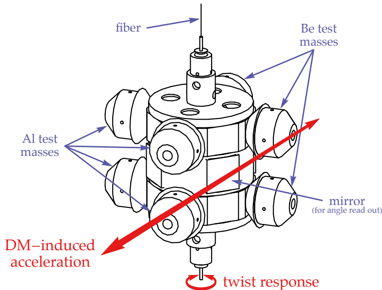
FIG. 1: A torsion pendulum for dark matter direct detection (figure adapted from [81]). The dark matter field directly induces an equivalence-principle violating acceleration on the test masses, resulting in an oscillating twist in the the pendulum. The twist angle is measured by observing the deflection of a laser reflected from the mirror.
