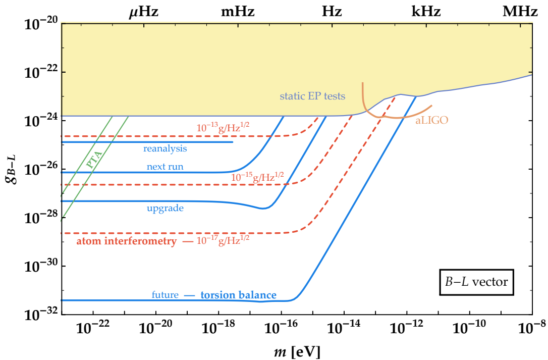
FIG. 2: Estimated reach of searches for B-L -coupled vector DM. Solid blue curves correspond to the torsion pendulum setups discussed in Sec. V A. Dashed red curves correspond to atom interferometers with acceleration sensitivities of 10^{-13} , 10^{-15} , and 10^{-17} \text{g Hz}^{-1/2} , as discussed in Sec. V B. Thin green curves correspond to the existing EPTA (upper) and upcoming SKA (lower) pulsar timing arrays, as discussed in Sec. V D. The orange curve shows our estimate of the reach of Advanced LIGO, as discussed in Sec. V A 4. The shaded region shows bounds from static EP tests using torsion pendulums [63]. For masses below \sim 10^{-22} eV the field cannot make up all of the dark matter due to its effect on structure formation – this bound may be improved in the future, as discussed in Sec. V E. Additional bounds from black-hole super-radiance may apply if the vector has no self interactions, as discussed in Sec. V E. We have not shown estimates for the sensitivity of lunar laser ranging to DM, but even existing data is potentially powerful (see Sec. V C).
