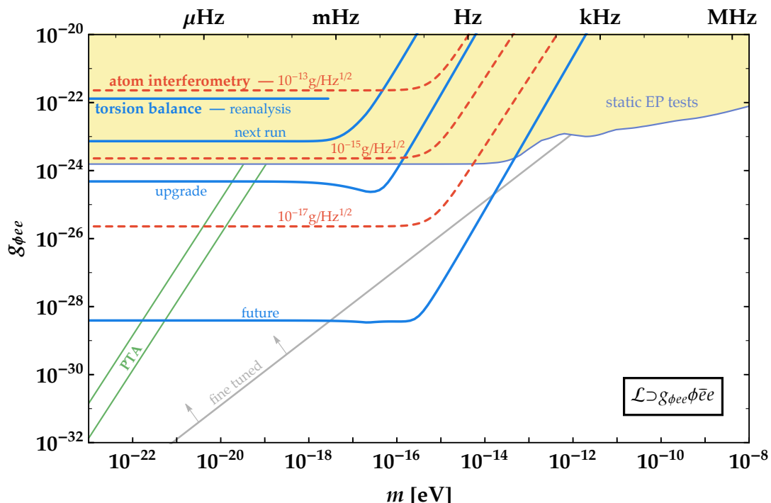
FIG. 4: Estimated reach of searches for scalar DM coupled through \mathcal{L} \supset g_{\phi ee} \phi \bar{e} e . The blue, red and green curves and the yellow shaded region are as in Fig. 2. Above the gray line the scalar mass is fine tuned if the cutoff \Lambda is above \sim \text{TeV} .
