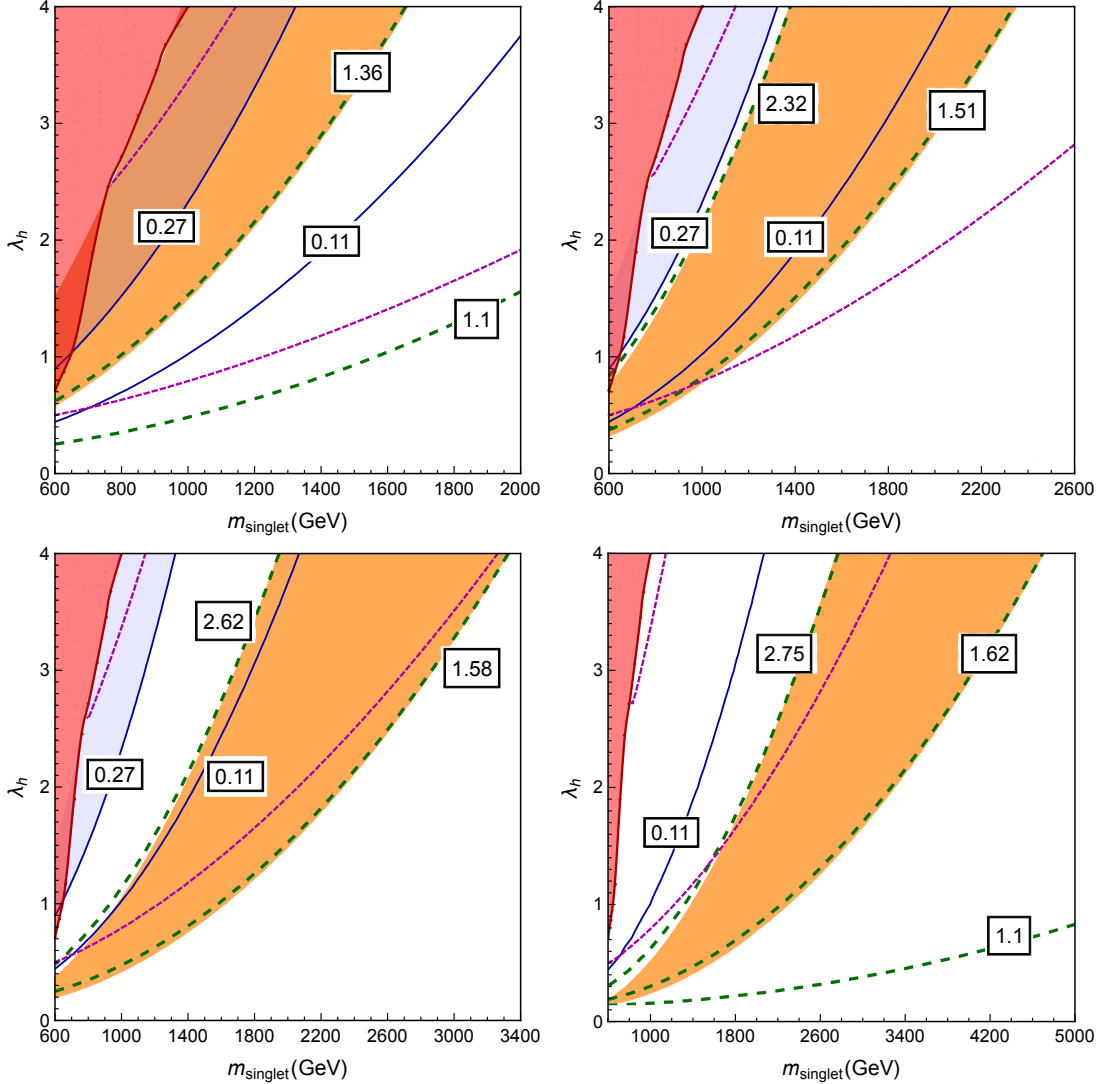
FIG. 3: Contours of the mixing parameter \sin^2 \theta (solid blue line) and of the enhancement of the triple-Higgs coupling (dashed green line) given by Eq. (29) in the m_{\text{singlet}}-\lambda_h plane. Blue shaded region denotes 2\sigma exclusion due to gluon fusion channel. The orange shaded region represents the region consistent with a FOEPT. The region excluded up to 2\sigma confidence level by Higgs precision measurements is shaded in red. The constraints coming from m_W are shown by magenta (short-dashed) lines. In the top-left panel we present results for \lambda_{hs} = 0.5 , while in the top-right, bottom-left and bottom-right panels we present results for \lambda_{hs} = 1, 2, 4 respectively.
