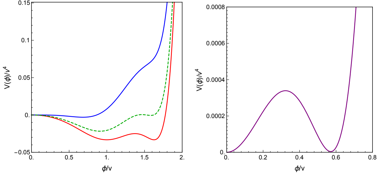
FIG. 2: Example of order (\phi^\dagger\phi)^5 potentials that correspond to the negative correction and also produce SFOEPT. In the left panel, the red line indicate the potential at T = 0 , the blue line correspond to the temperature where the curvature at \phi = 0 is 0. The green line correspond to the intermediate temperature of \sim 35 GeV. The purple curve on the right shows the potential at T = T_c . The coefficients c_6 = 0.906 , c_8 = -1 , c_{10} = 0.346 , while \Lambda \sim 263 GeV, T_c \sim 44 GeV assuming a_0 \sim 3 as in the SM and \delta = -1.23 .
