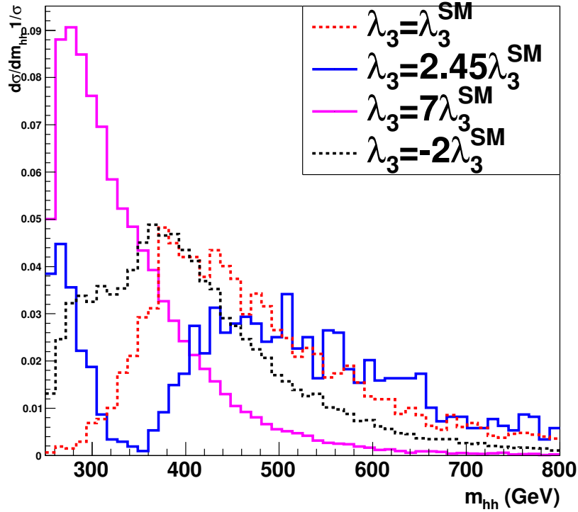
FIG. 4: Normalized m_{hh} distributions for \lambda_3 = \lambda_3^{SM} , \lambda_3 = 2.45\lambda_3^{SM} and \lambda_3 = 7\lambda_3^{SM} and \lambda_3 = -2\lambda_3^{SM} . The cancellation between the box and triangle diagram is exact at \lambda_3 = 2.45\lambda_3^{SM} at 2m_t threshold, that explains the dip. Note that the distribution shifts to smaller values as \lambda_3 increases
