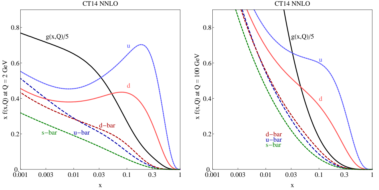
FIG. 5: The CT14 parton distribution functions at Q = 2 GeV and Q = 100 GeV for u, \bar{u}, d, \bar{d}, s = \bar{s} , and g .
