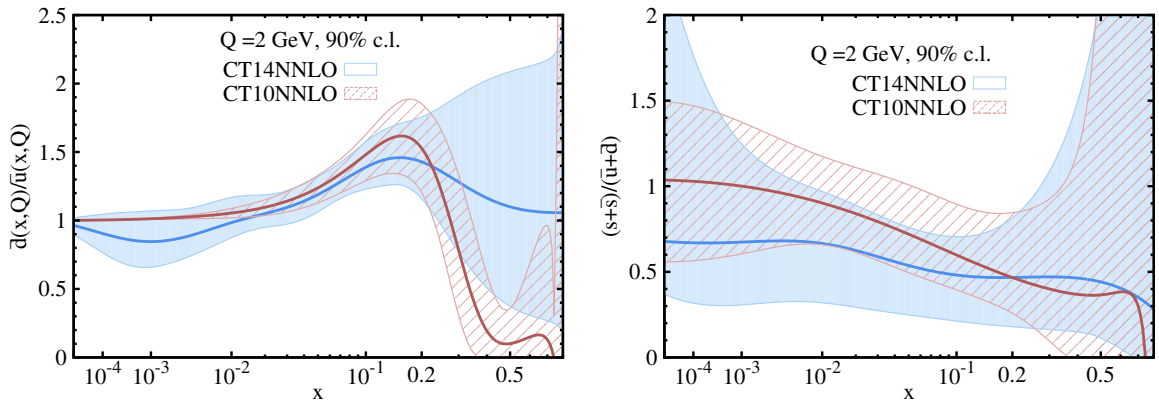
FIG. 8: A comparison of 90% C.L. uncertainties on the ratios \bar{d}(x, Q)/\bar{u}(x, Q) and (s(x, Q) + \bar{s}(x, Q))/(\bar{u}(x, Q) + \bar{d}(x, Q)) , for CT14 NNLO (solid blue) and CT10 NNLO (red dashed) error ensembles.
