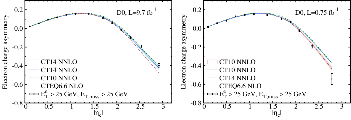
FIG. 25: Charge asymmetry of decay electrons from W^\pm production measured by the D\bar{O} experiment in Run-2 at the Tevatron with high (left) and low (right) luminosities, compared to several generations of CTEQ-TEA PDFs.
