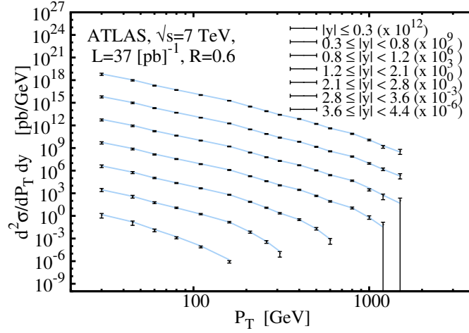
FIG. 16: Comparison of data on d^2\sigma/dp_T dy and NLO theory for the ATLAS 7 TeV inclusive jet production, using CT14 NNLO PDFs.
