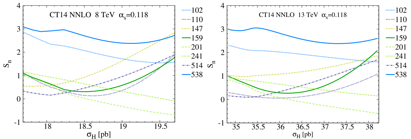
FIG. 37: The equivalent Gaussian variable S_n versus \sigma_H at the LHC with \sqrt{s} = 8 and 13 TeV.
