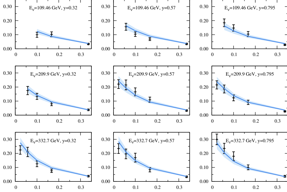
CCFR Neutrino, d^2\sigma(\nu_\mu N \rightarrow \mu^+ \mu^- X)/dx dy
