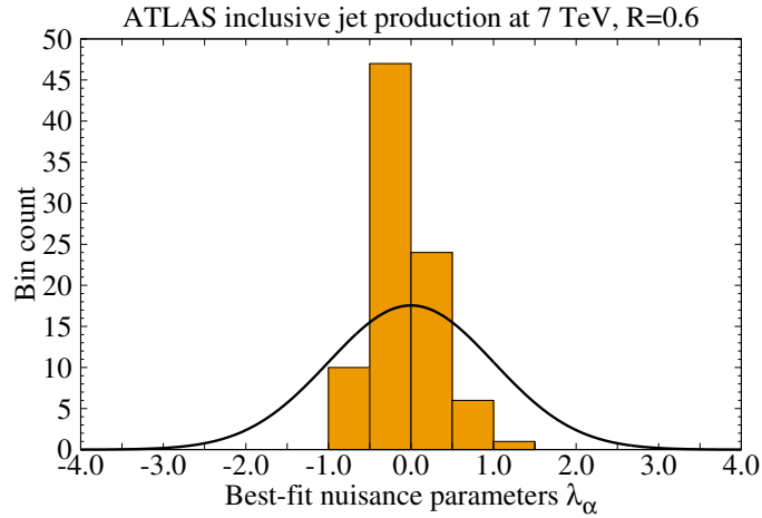
FIG. 18: Histogram of optimized nuisance parameters \lambda_\alpha for the sources of correlated systematic errors of the ATLAS 7 TeV inclusive jet production.
