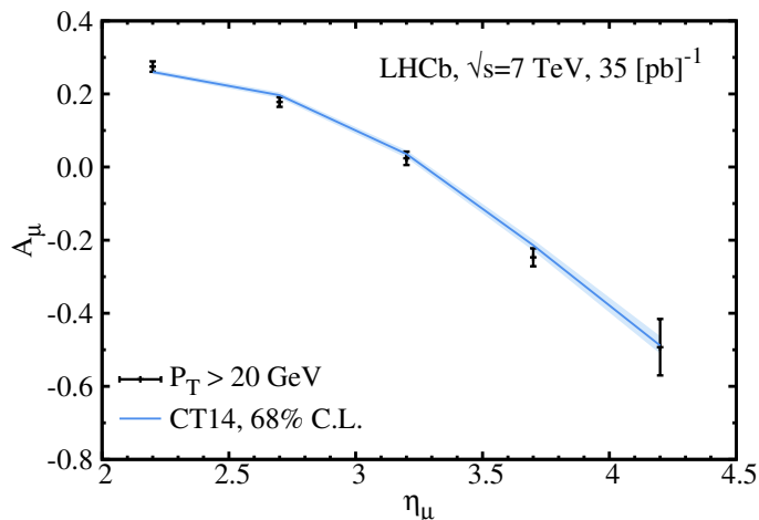
FIG. 22: Charge asymmetry of decay muons from W^\pm production measured by the LHCb experiment.
