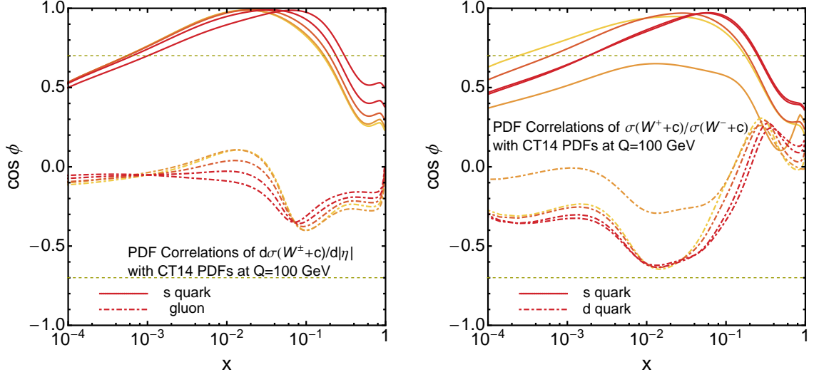
FIG. 32: Correlation cosines between the PDFs of select flavors, the W^\pm + c cross section, and the W^+/W^- cross section ratio, as a function of x in the PDF.
