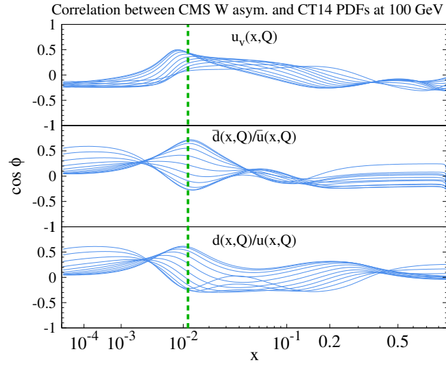
FIG. 2: The correlation cosine \cos \phi [13] between the PDF f(x, Q = 100 \text{ GeV}) at the specified x value on the horizontal axis and NNLO predictions for muon CMS charge asymmetry [46].
