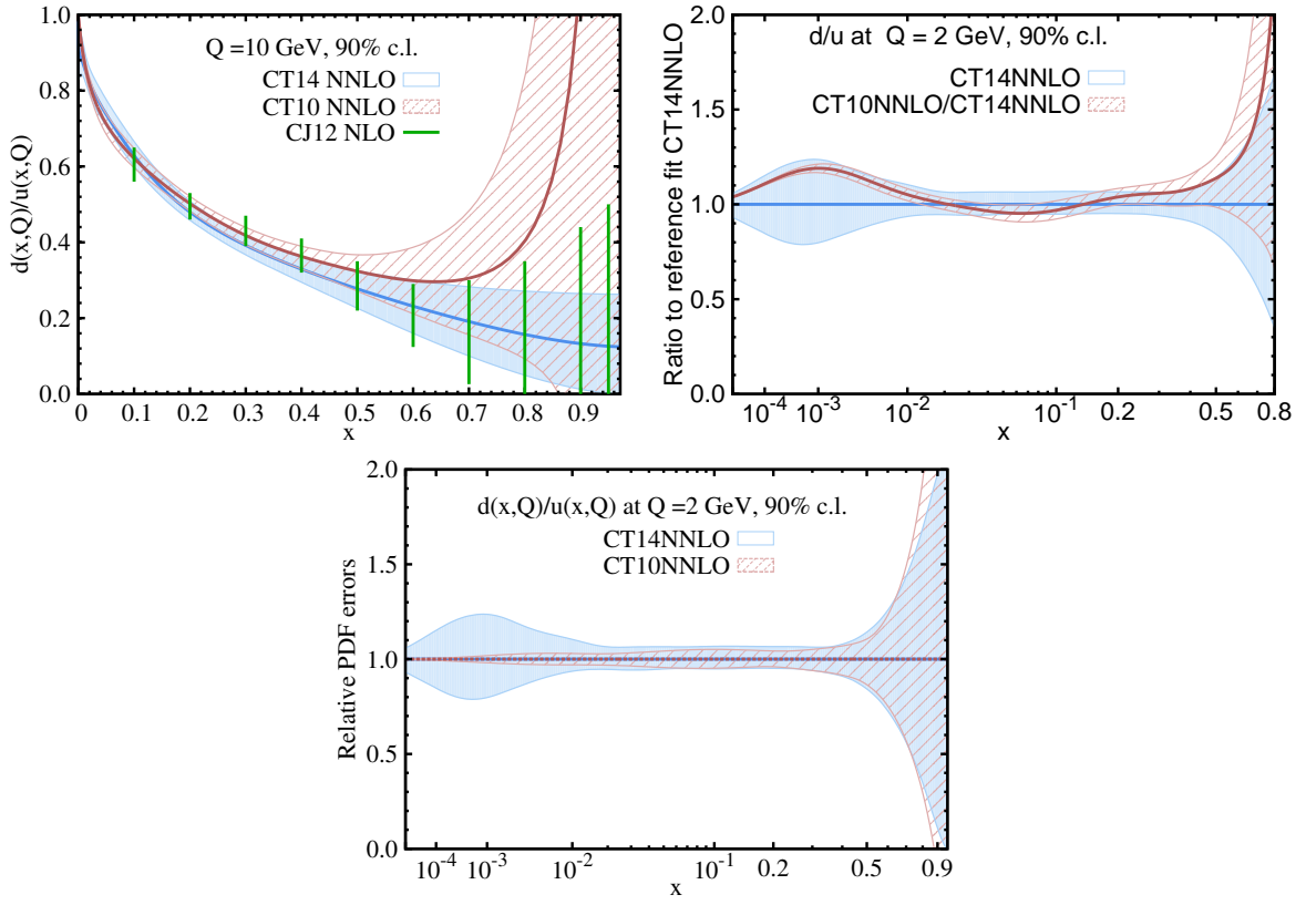
FIG. 7: A comparison of 90% C.L. uncertainties on the ratio d(x, Q)/u(x, Q) for CT14 NNLO (solid blue) and CT10 NNLO (red dashed) error ensembles.
