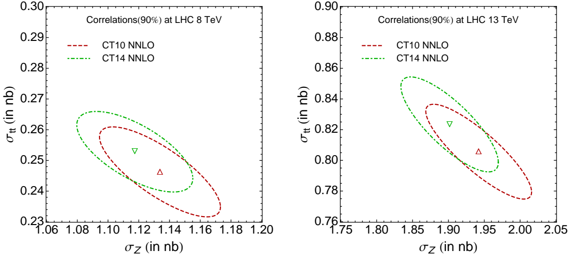
FIG. 11: CT14 and CT10 NNLO 90% C.L. error ellipses for t\bar{t} and Z cross sections, at the LHC 8 and 13 TeV.
