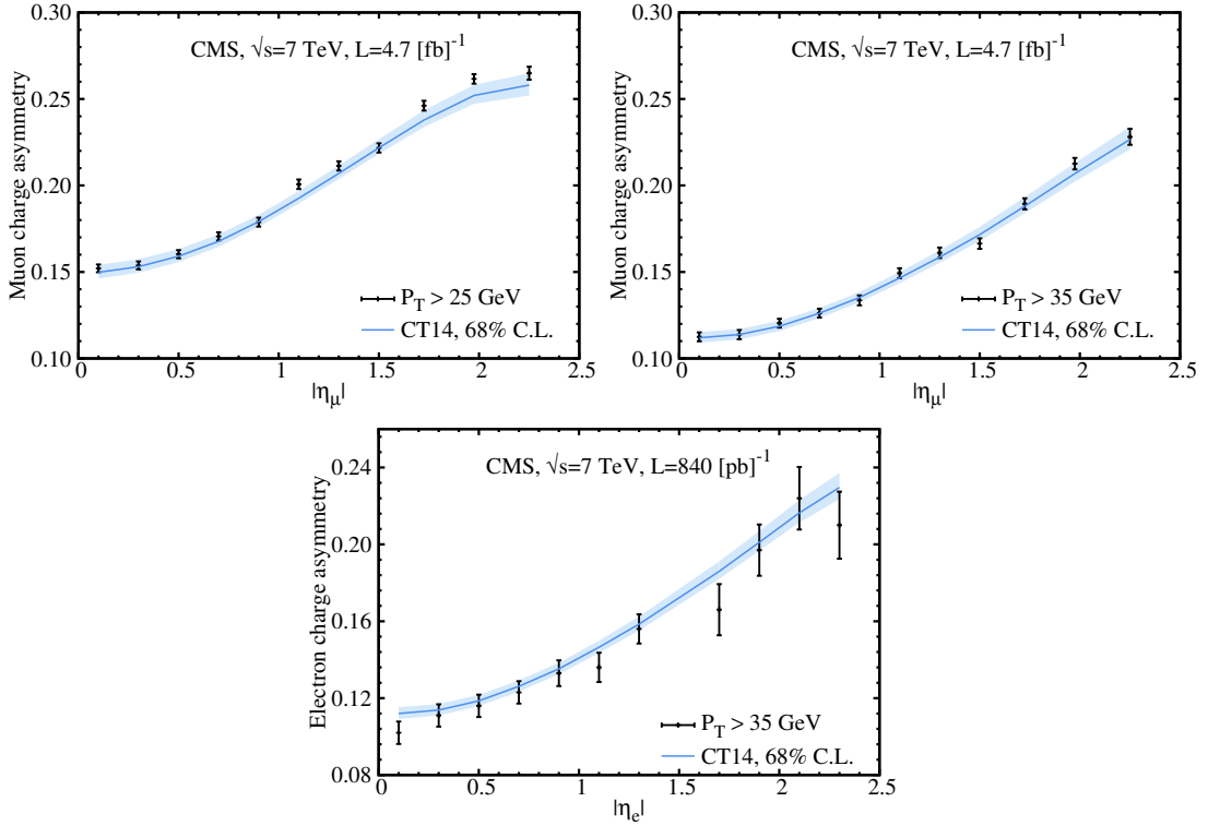
FIG. 21: Charge asymmetry of decay muons and electrons from W^\pm production measured by the CMS experiment. The data values have p_{T\ell} > 25 or 35 GeV for the muon data and p_{T\ell} > 35 GeV for the electron data. The vertical error bars on the data points indicate total (statistical and systematic) uncertainties. The curve shows the CT14 theoretical calculation; the shaded region is the PDF uncertainty at 68% C.L.
