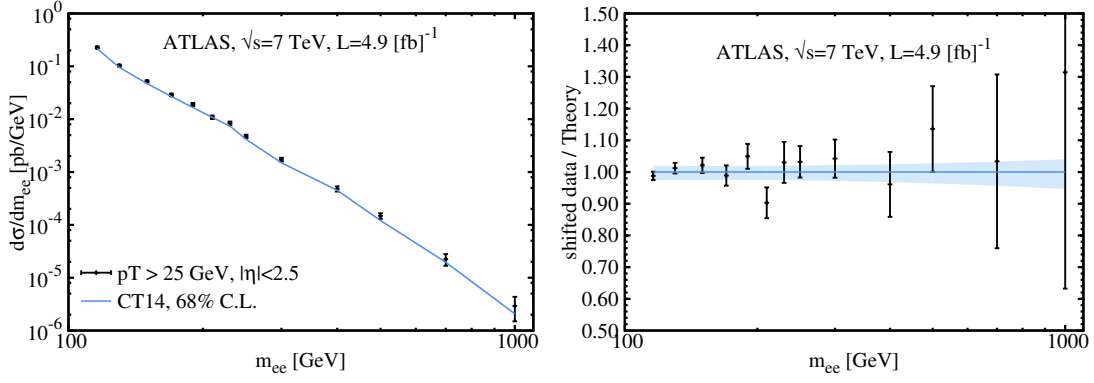
FIG. 23: Invariant mass distributions of Drell-Yan pairs in the high-mass region by ATLAS 7 TeV [108], with superimposed NNLO predictions based on CT14 NNLO PDFs. The left subfigure shows the differential cross sections as a function of the dilepton mass m_{ee} . The right subfigure shows the ratio of ATLAS shifted data to CT14 theory predictions.
