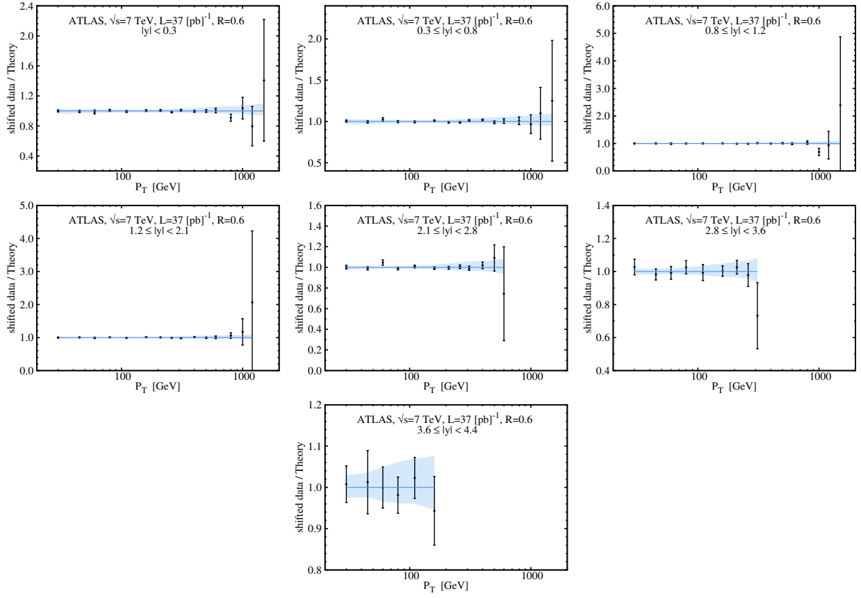
FIG. 17: Same as Fig. 16, shown as the ratio of shifted data for ATLAS 7 TeV divided by the NLO theory. The error bars correspond to total uncorrelated errors. The shaded region shows the 68% C.L. PDF uncertainties.
