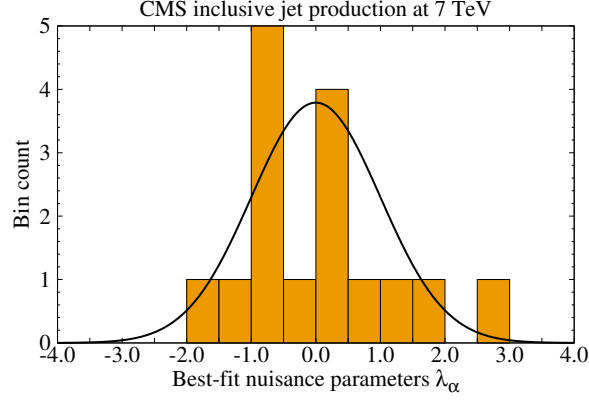
FIG. 15: Histogram of optimized nuisance parameters \lambda_\alpha for the sources of correlated systematic errors of the CMS 7 TeV inclusive jet production. The curve is the standard normal distribution expected in the ideal case.
