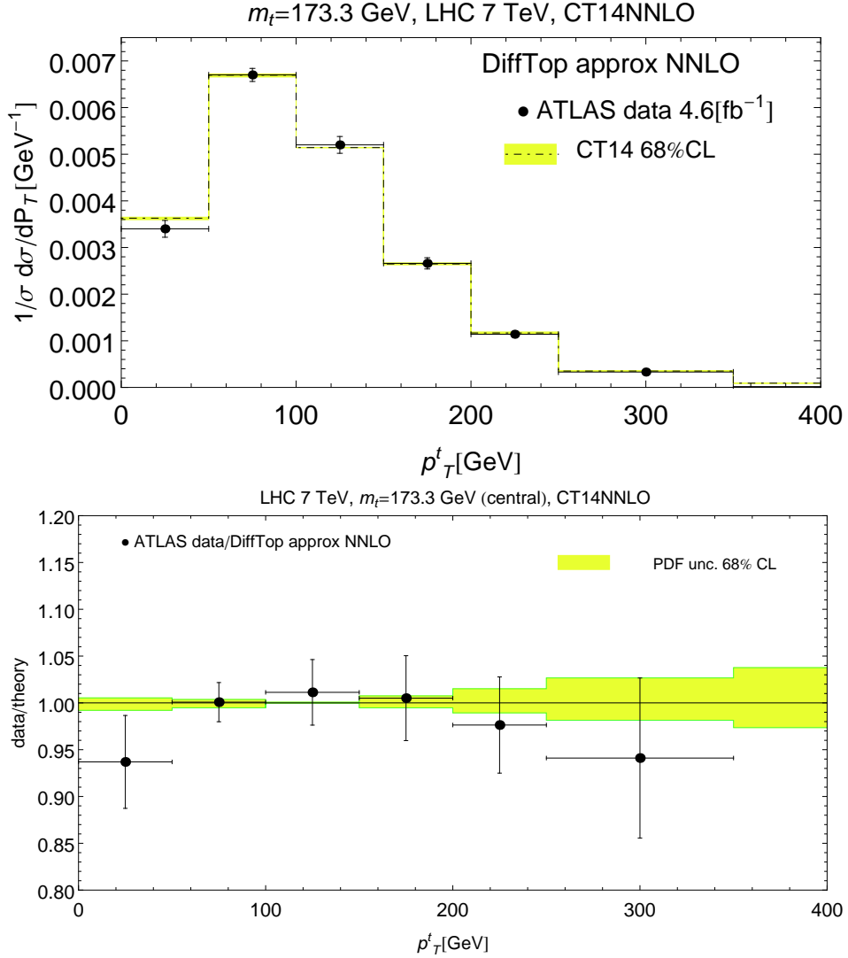
FIG. 40: Normalized final-state top-quark p_T differential distribution at ATLAS 7 TeV.
