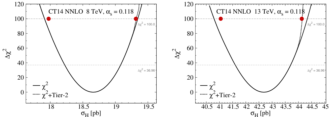
FIG. 34: Dependence of the increase in \chi^2 in the constrained CT14 fit on the expected cross section \sigma_H at the LHC 8 and 13 TeV, for \alpha_s(M_Z) = 0.118 . The solid and dashed curves are for the constrained fits without and with the Tier-2 penalties, respectively. The red dots correspond to the upper and lower 90% C.L. limits calculated by the Hessian method.
