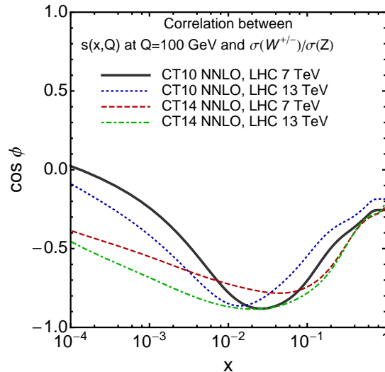
FIG. 33: Correlation cosines between the ratio of total cross sections for W^\pm production and Z boson production, and s quark PDF from CT14 and CT10 NNLO sets, for LHC 7 and 13 TeV.
