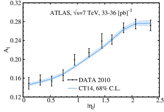
FIG. 20: W^\pm charge asymmetry as a function of lepton pseudorapidity measured by the ATLAS Collaboration, compared to the 68% C.L. CT14 NNLO uncertainty band. The kinematic requirements are p_{T\ell} > 20 GeV, p_{T\nu\ell} > 25 GeV and M_T^{\ell\nu\ell} > 40 GeV.
