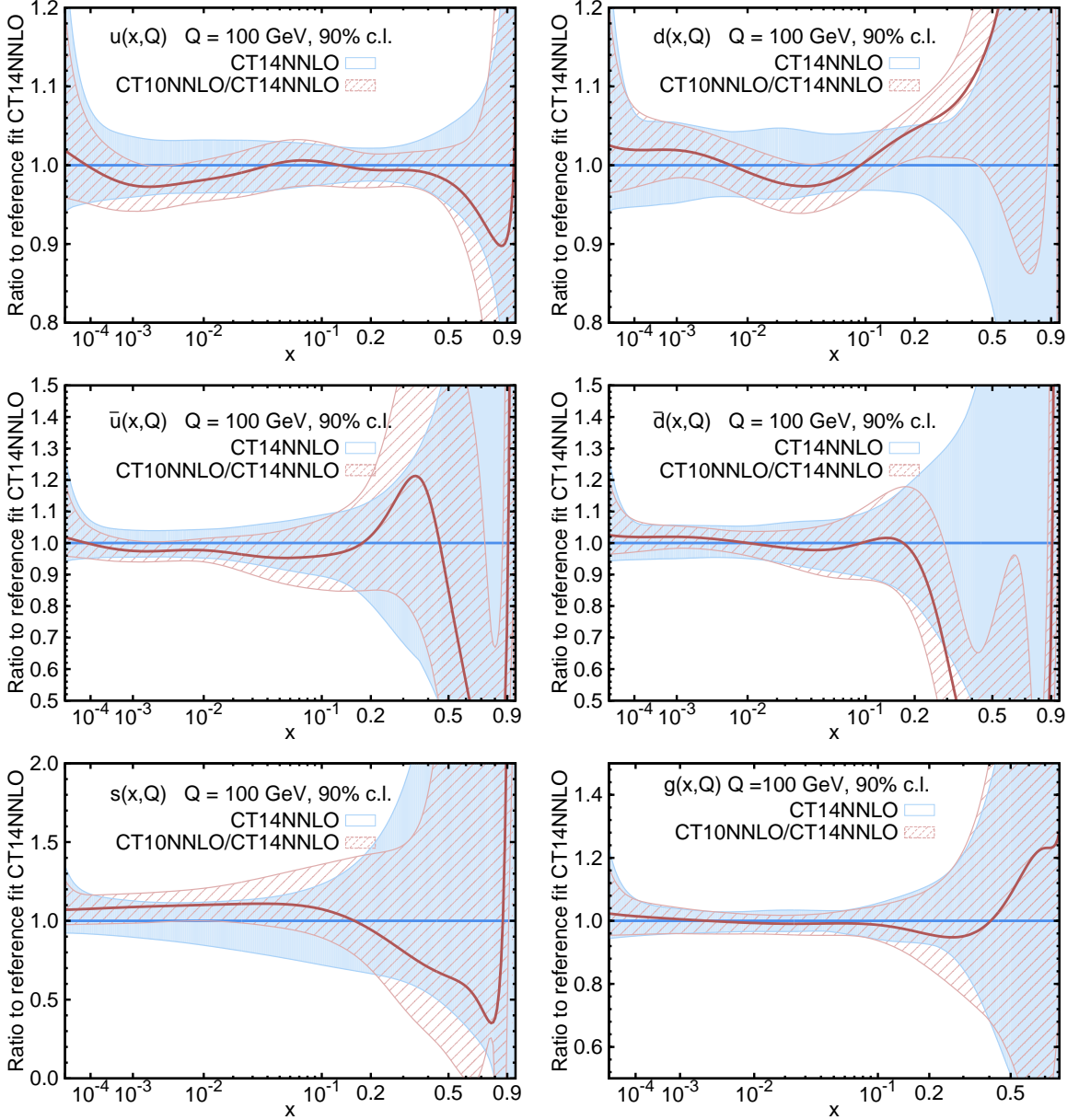
FIG. 6: A comparison of 90% C.L. PDF uncertainties from CT14 NNLO (solid blue) and CT10 NNLO (red dashed) error sets. Both error bands are normalized to the respective central CT14 NNLO PDFs.
