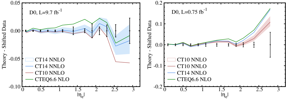
FIG. 26: Same as Fig. 25, plotted as the difference between theory and shifted data for A_{ch} from D\bar{O} Run-2 ( 9.7 \text{ fb}^{-1} ).
