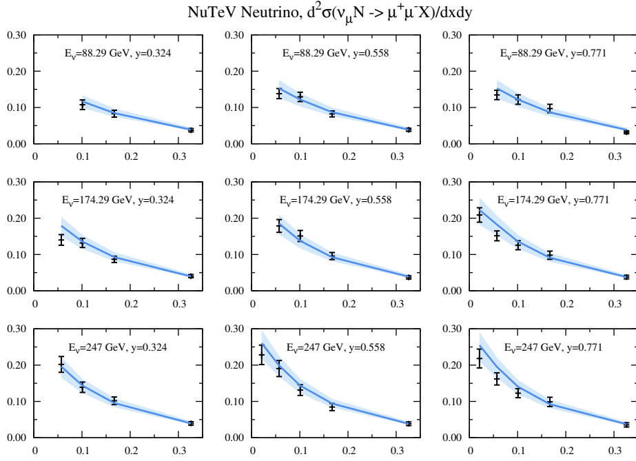
FIG. 27: Comparison of data and theory for the NuTeV measurements of dimuon production in neutrino-iron collisions. The data are expressed in the form of d^2\sigma/dx dy and shown as a function of x for a certain y and neutrino energy.
