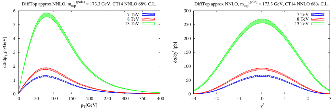
FIG. 42: Absolute differential p_T and y distributions for the final-state top-quark in t\bar{t} production at the LHC at \sqrt{s} = 7, 8, and 13 TeV.
