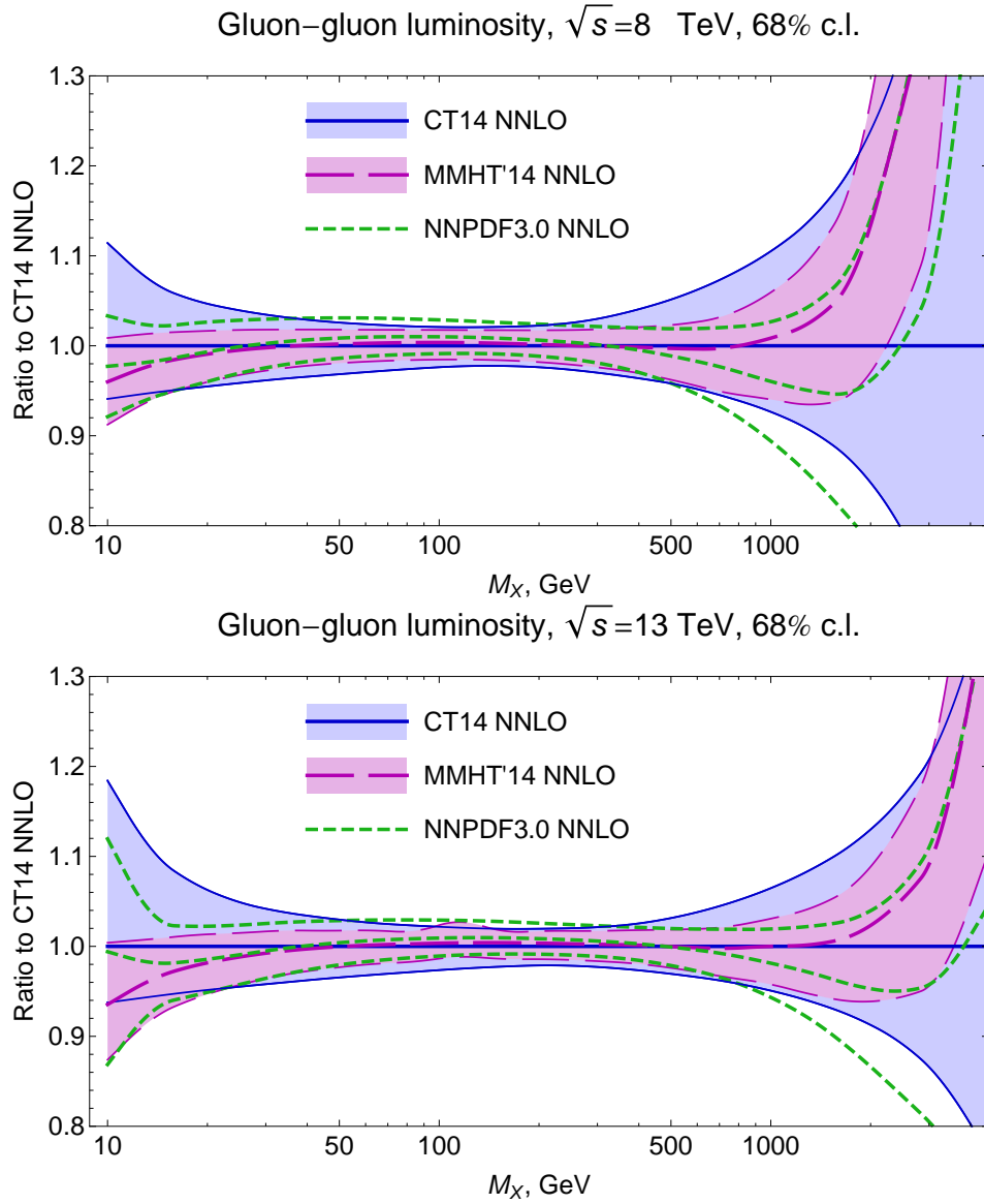
FIG. 36: The gg PDF luminosities for CT14, MMHT2014 and NNPDF3.0 PDFs at the LHC with \sqrt{s} = 8 and 13 TeV, with \alpha_s(M_Z) = 0.118 .
