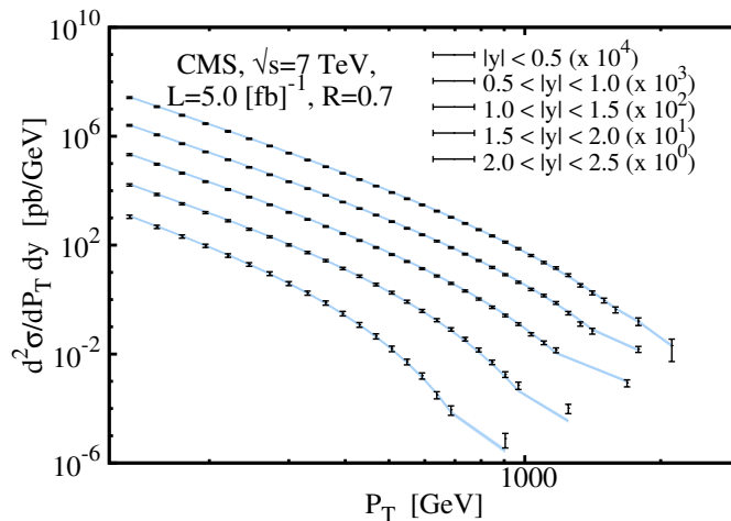
FIG. 13: Comparison of data and theory for the CMS 7 TeV inclusive jet production, for CT14 NNLO PDFs. Measurements of d^2\sigma/dp_T dy for 5 rapidity bins are plotted as functions of jet p_T . The points are data with total experimental errors, obtained by adding the statistical and systematic errors in quadrature. The bands are theoretical calculations with 68% C.L. PDF uncertainties.
