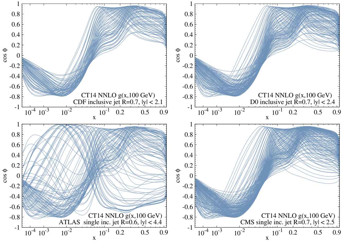
FIG. 3: The correlation cosine \cos \phi [13] between the g-PDF at the specified x value on the horizontal axis and NLO predictions for the CDF [49] (upper left panel), D0 [50] (upper right panel), ATLAS [51] (lower left panel) and CMS [52] (lower right panel) inclusive jet cross sections at Q = 100 GeV.
