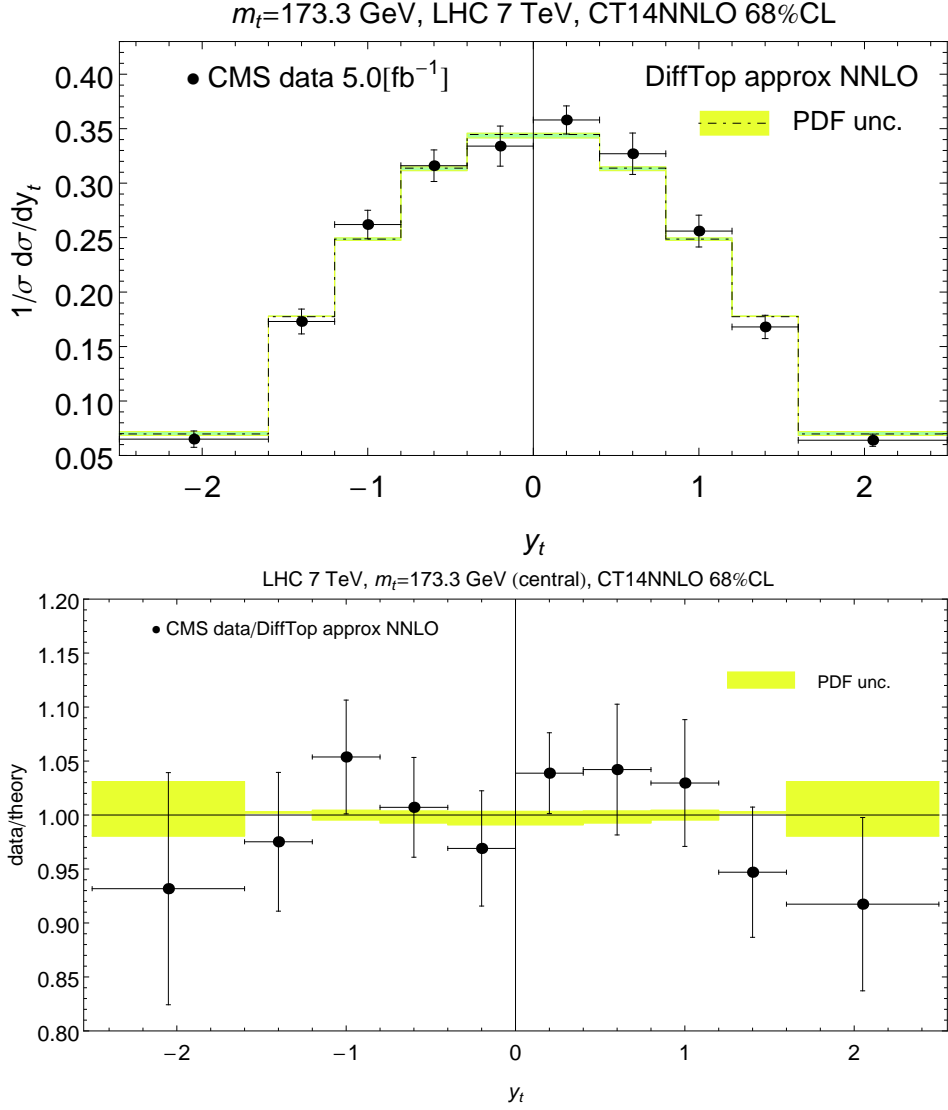
FIG. 39: Normalized final-state top-quark rapidity distribution at CMS 7 TeV.
