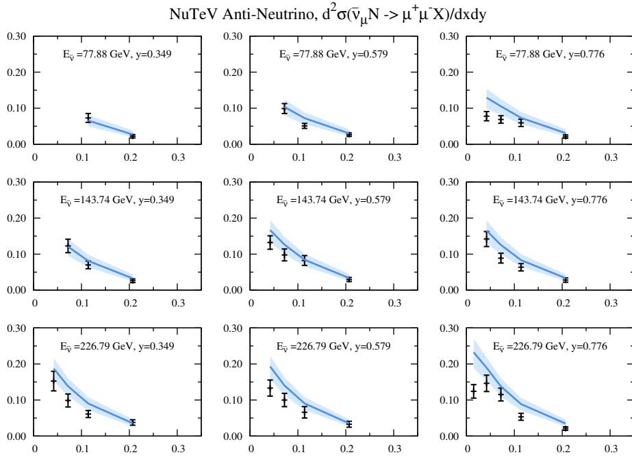
FIG. 28: Same as Fig. 27, for the NuTeV measurements of dimuon production in antineutrino-iron collisions.
