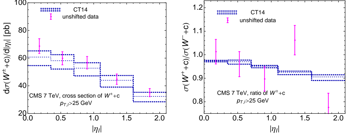
FIG. 31: Comparison of the CT14 prediction for W^\pm + c differential cross sections (left) and for the ratio of W^+ + \bar{c} to W^- + c cross sections (right) from the CMS measurement at 7 TeV.
