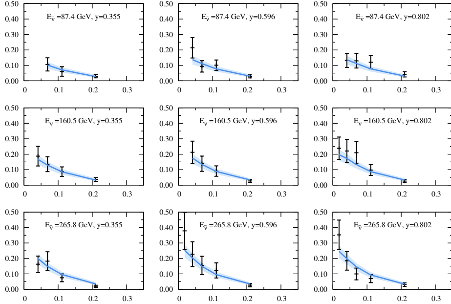
CCFR Anti-Neutrino, d^2\sigma(\bar{\nu}_\mu N \rightarrow \mu^+ \mu^- X)/dx dy
