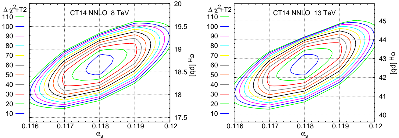
FIG. 35: Contour plots of \Delta\chi^2(\alpha_s(M_Z), \sigma_H) plus Tier-2 penalty in the (\alpha_s(M_Z), \sigma_H) plane, for \sigma_H at the LHC 8 and 13 TeV.
