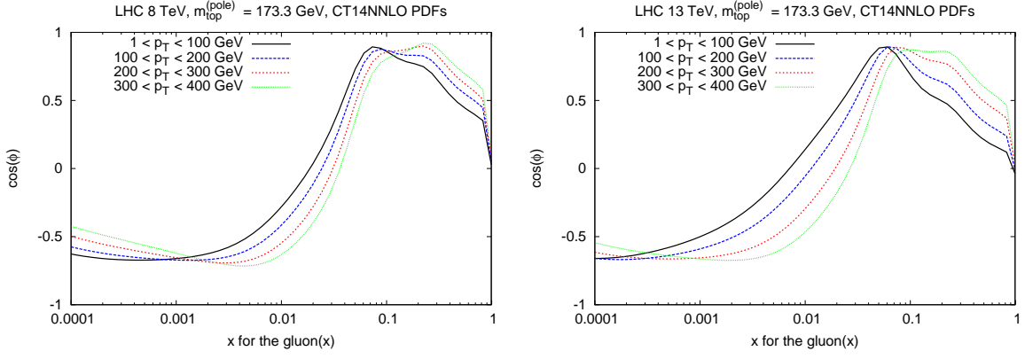
FIG. 41: Theoretical correlation cosine as a function of x -gluon for the top-quark p_T distribution in t\bar{t} production at the LHC at \sqrt{s} = 8 and 13 TeV.
