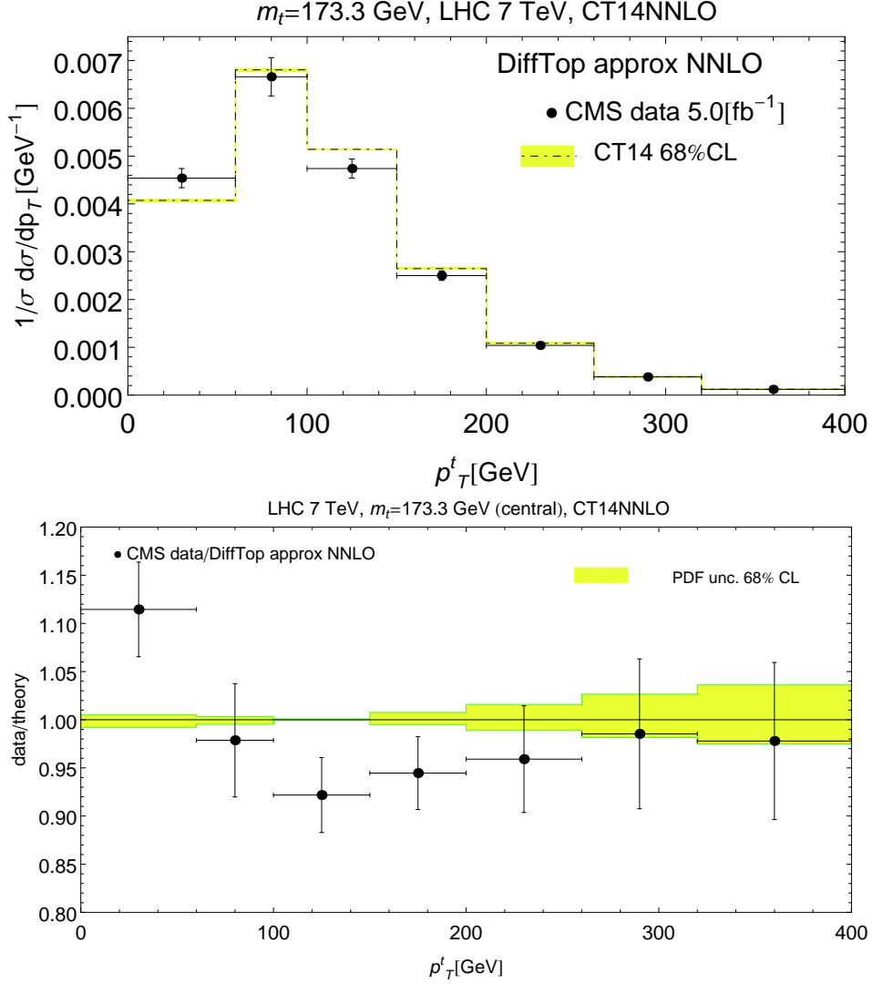
FIG. 38: Normalized final-state top-quark p_T differential distribution at CMS 7 TeV.
