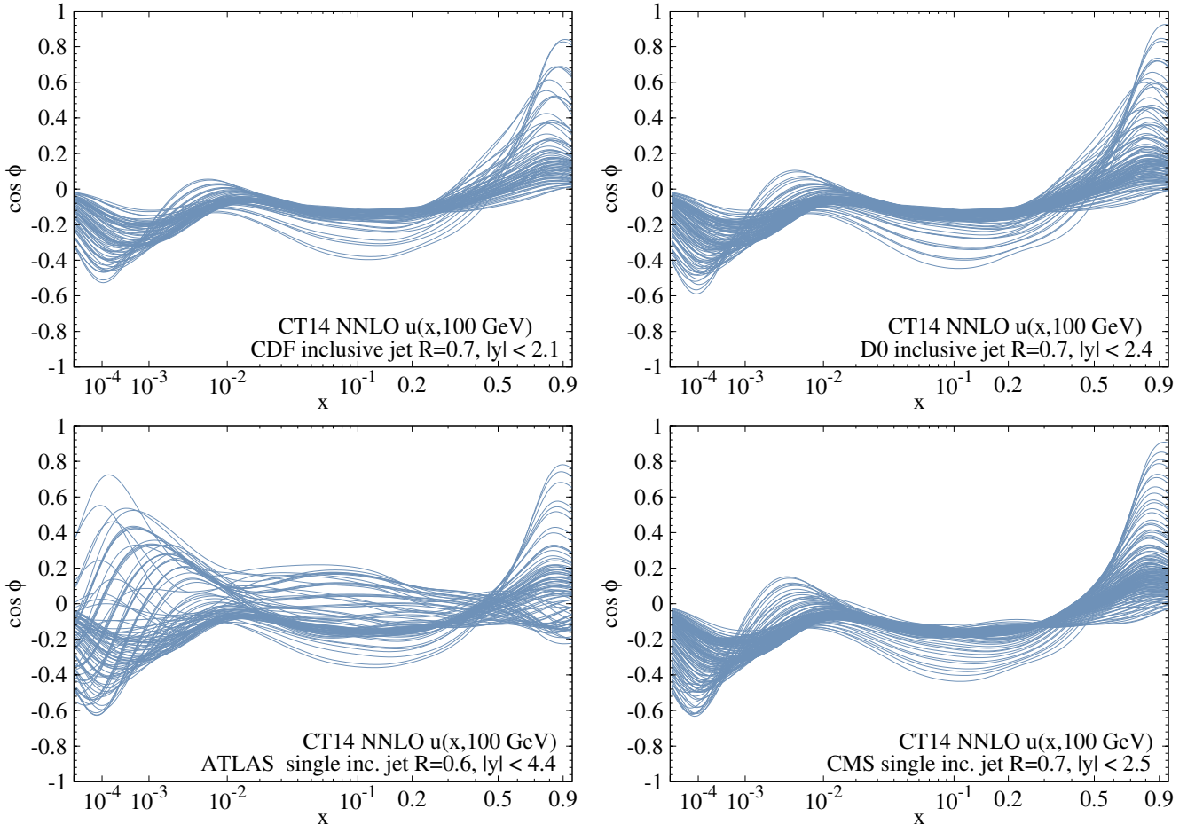
FIG. 4: The correlation cosine \cos \phi [13] between the u -PDF at the specified x value on the horizontal axis and NLO predictions for the CDF [49] (upper left panel), DØ [50] (upper right panel), ATLAS [51] (lower left panel) and CMS [52] (lower right panel) inclusive jet cross sections at Q = 100 \text{ GeV} .
