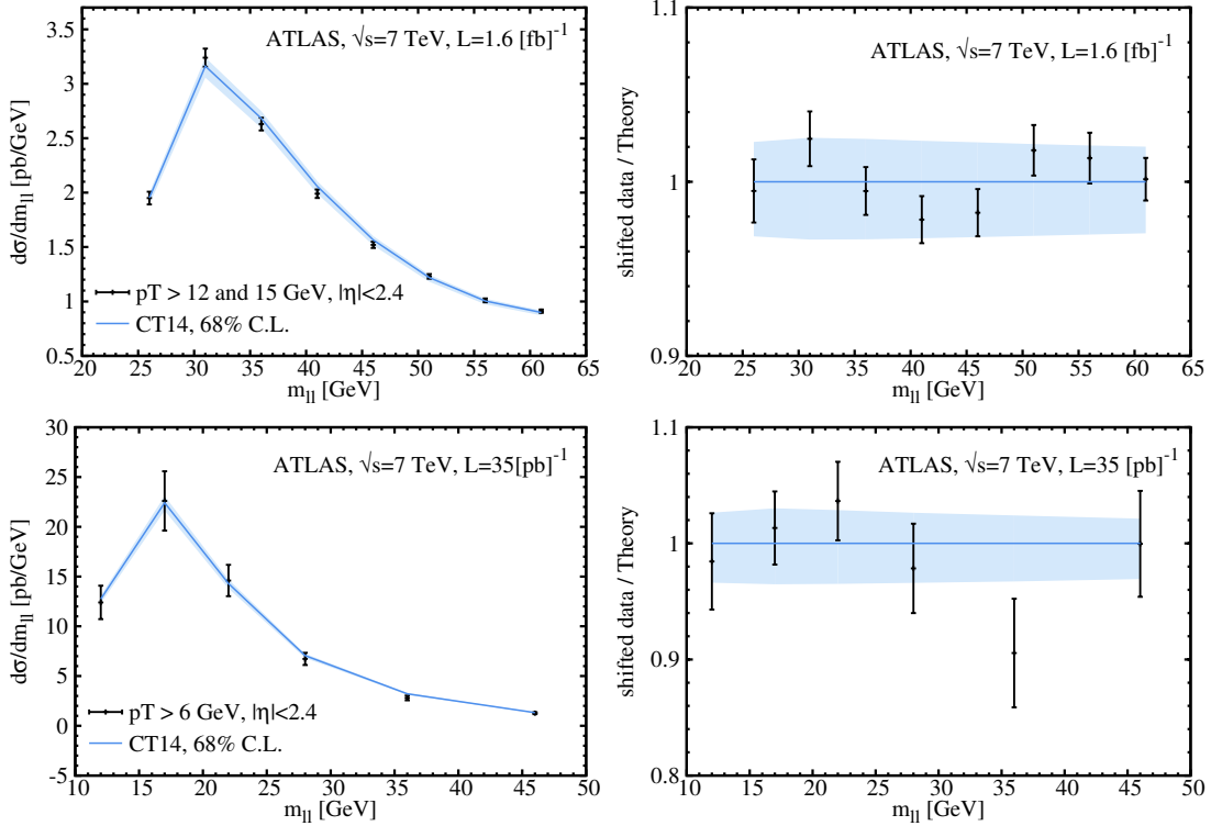
FIG. 24: Same as in Fig. 23, for ATLAS 7 TeV differential distributions of Drell-Yan pairs in the low-mass and extended low-mass regions [109].
