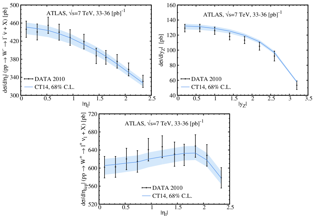
FIG. 19: Comparison between the 2010 ATLAS measurements [48] of the W^\pm charged-lepton pseudorapidity and Z boson rapidity distributions at \sqrt{s} = 7 TeV, and the RESBOS theory using CT14 NNLO PDFs.
