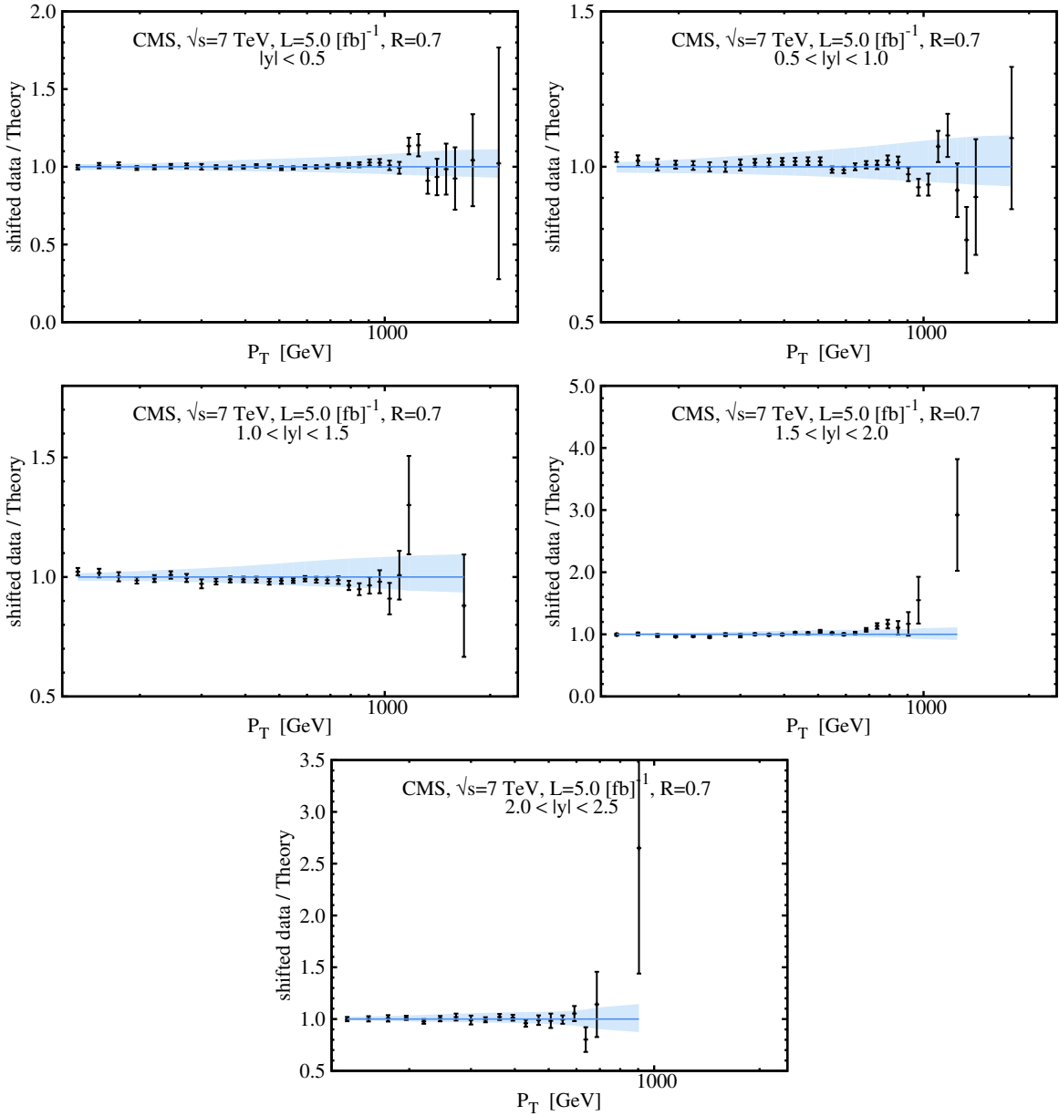
FIG. 14: Same as Fig. 13, shown as the ratio of shifted data for CMS 7 TeV divided by theory. The error bars correspond to total uncorrelated errors. The shaded region shows the 68% C.L. PDF uncertainties.
