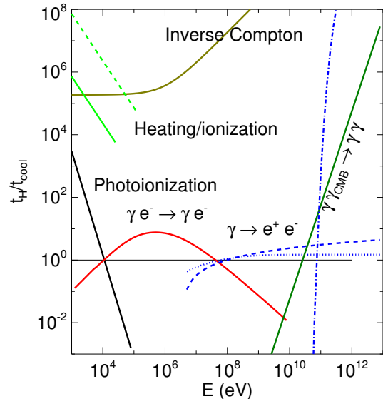
FIG. 4: Energy-loss processes for keV-TeV photons (black, red, blue and dark green lines) and electrons (light green and gold lines), and the corresponding cooling times ( t_{cool} ) relative to the Hubble time ( t_H ) at z = 600 . For photons, the dominant processes (in order of increasing energy) are photoionization (black solid line), Compton scattering (red solid line), pair production on the gas (blue dashed and dotted lines; dashed for ionized gas, dotted for neutral gas), photon-photon scattering (green solid line), and pair production on the CMB (blue solid line). For electrons, at low energies cooling is dominated by atomic processes (light green lines), whereas at higher energies inverse Compton scattering (solid gold line) takes over; both are much faster than a Hubble time. The dashed light green line corresponds to heating in an ionized medium (the characteristic timescale is increased proportionally if the ionized fraction is reduced); the solid light green line corresponds to ionization in a neutral medium (the characteristic timescale is increased proportionally if the neutral fraction is reduced). Estimates for the electron cooling rates are taken from [17].
