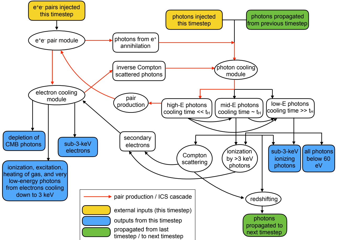
FIG. 5: Chart showing the structure of the high-energy electron/photon cooling code developed in [13]. This chart shows the processes modeled at each timestep; arrows indicate the direction of particle flow, ellipses mark processes and sub-modules, whereas boxes describe the particles tracked at each stage. Green boxes indicate particle data that are propagated forward to the next timestep, or taken as inputs from the previous timestep; yellow boxes show data that are input at each new timestep (any new particle injection from e.g. DM annihilation); blue boxes describe outputs of the code that are logged to an external file at each timestep. Red lines mark steps in the rapid pair production / inverse Compton scattering cascade that dominates the initial cooling of high-energy electrons and photons; this cascade is iterated until all (primary and secondary) particles have lost enough energy that pair production is no longer possible. See the text for a brief description of the code, and [13] for details.
