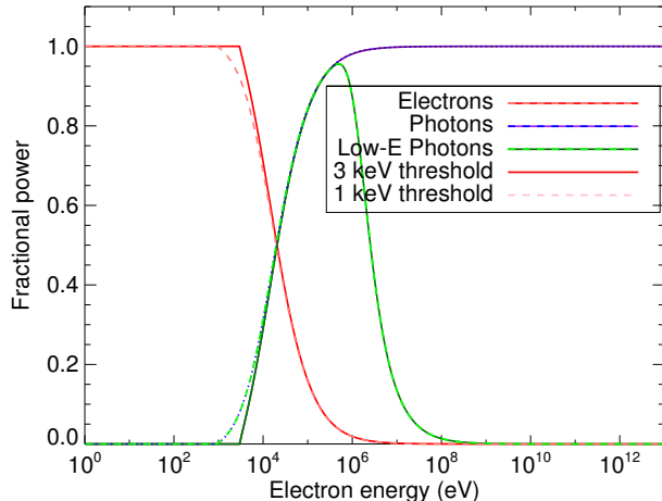
FIG. 3: Fraction of electron kinetic energy eventually partitioned into (red/pink) excitation/ionization/heating of the gas, plus electrons below the energy cutoff where atomic cooling processes dominate, and (blue/violet) photons produced by inverse Compton scattering of the electron on the CMB. Photons below 10.2 eV, which no longer interact significantly with the gas, constitute a subset of the latter contribution (light/dark green). All curves are for electrons depositing their energy at redshift 600. Dashed and dotted lines (pink, blue, light green) correspond to a 1 keV threshold, whereas solid lines (red, violet, dark green) correspond to a 3 keV threshold; we see that the behavior is fairly independent of the chosen threshold except very close to it.
