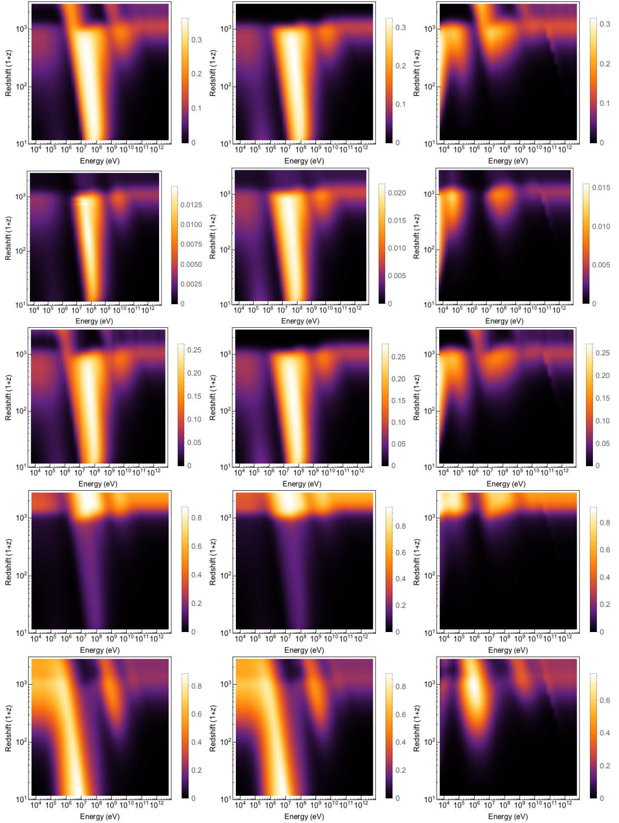
FIG. 7: Total power deposited (down to 1+z=10 ) into each channel, as a function of injection energy and redshift. From top to bottom, the rows correspond to H ionization, He ionization, Lyman- \alpha photons, heating, and sub-10.2 eV continuum photons. The left column describes energy absorption for e^+e^- pairs (the x -axis “energy” label here indicates the kinetic energy of a single member of the pair at injection), while the right column describes energy absorption for photons. The center column is an alternate method of estimating the same quantities shown in the left column, as described in Section IV A 1, and should be regarded as a cross-check.
