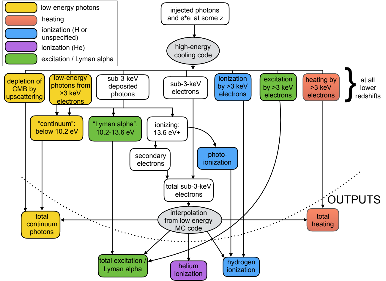
FIG. 6: Chart showing how the outputs of the high-energy code (see Section III) are converted into contributions to each of the energy-absorption channels, for all redshifts lower than the initial injection redshift. Boxes below the dotted line denote outputs. Different colors denote contributions to the different channels. Gray ellipses denote the use of the high-energy cooling code or results from a low-energy Monte Carlo code, taken from [15]. See text for details.
