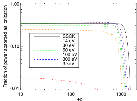
FIG. 2: Fraction of deposited power that contributes to (hydrogen) ionization as a function of redshift, employing the “SSCK” prescription (solid black line), and the results presented in [15] for electrons at a range of energies. The “3 keV” prescription corresponds to the purple dashed line.
