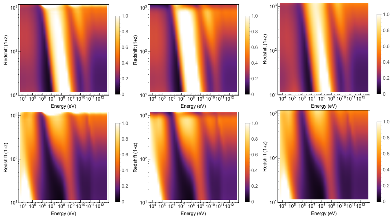
FIG. 11: Corrected f(z) curve for particles injected by DM annihilation, as a function of injection energy and redshift of absorption. In the left panel we use the “3 keV” baseline ionization fractions (so these f(z) curves should be used with analyses that employed the same prescription); in the center panel we use the “SSCK” baseline. In the right panel we correct for the continuum losses using the results of Figure 12, and thus derive an alternate channel-independent f^{\text{sim}}(z) curve. The upper row describes e^+e^- pairs (the x -axis “energy” label here indicates the kinetic energy of a single member of the pair at injection), the lower row describes photons.
