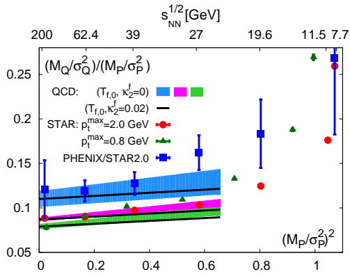
FIG. 2. The ratio of ratios of mean and variance for net-electric charge and net-proton number fluctuations measured by the STAR and PHENIX Collaborations. For the STAR electric charge data [16] we show results obtained by normalizing with net-proton results from the published STAR0.8 data set [14] (triangles) as well as the preliminary STAR2.0 data set [15] (circles). The experimental data is compared to QCD predictions for two values of \kappa_2^f (see text). The electric charge results obtained by PHENIX [17] have been normalized by using the STAR2.0 data set on net-proton fluctuations (boxes). For orientation the upper x-axis shows \sqrt{s_{NN}} energies of the RHIC beam energy scan with labels put at the values for (M_P/\sigma_P)^2 corresponding to the STAR2.0 data set. Errors on (M_P/\sigma_P)^2 are not visible as they are smaller than the size of the symbols.
