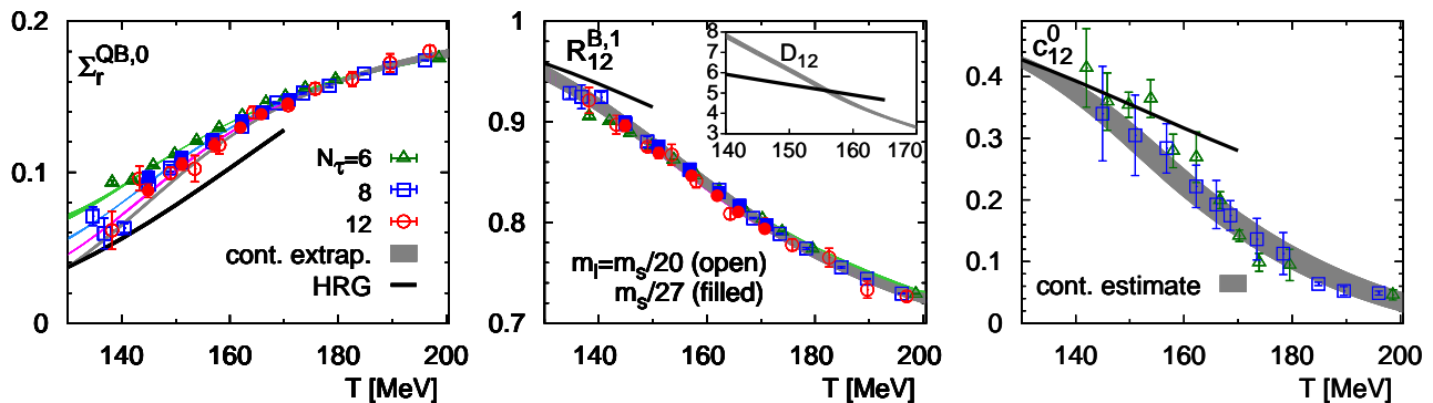
FIG. 1. Temperature dependence of the LO expansion coefficients of the ratio \Sigma_r^{QB} (left) and R_{12}^B (middle) and the NLO coefficient c_{12}^0 (right) introduced in Eq. 7. The NLO coefficient D_{12} (Eq. 7) is shown as an insertion in the middle panel. Shown are data from calculations with the HISQ action on lattices of size N_\sigma^3 \times N_\tau , with N_\sigma = 4N_\tau . Bands show continuum extrapolations for the LO observables and continuum estimates for the NLO observable c_{12}^0 (see text).
