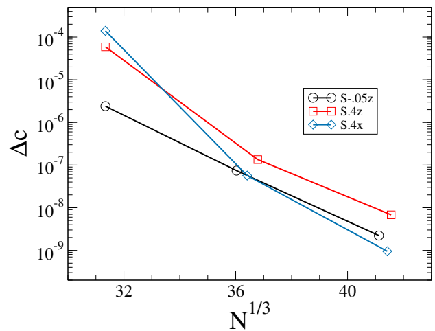
FIG. 4. Convergence of the location of the stellar surface. Plotted is \Delta c as defined in Eq. (63), for three representative configurations.
