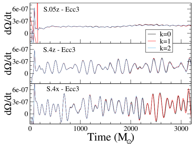
FIG. 12. Convergence of \dot{\Omega}(t) . Shown are \dot{\Omega}(t) at three different numerical resolutions ( k = 0, 1, 2 ) for the final, lowest-eccentricity initial data. The oscillations in \dot{\Omega}(t) are evidently not caused by numerical truncation error. Note that \dot{\Omega} has units of M_\odot^{-2} .
