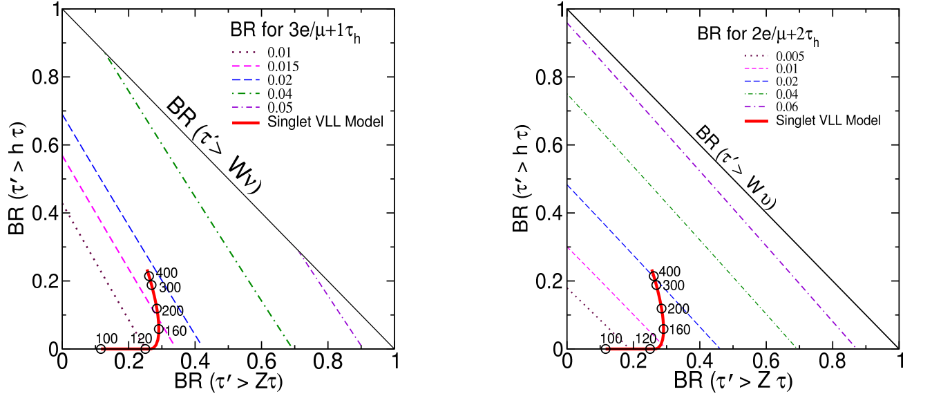
FIG. 11: Contour lines for total branching ratio of \tau'^+\tau'^- into \geq 3e/\mu + 1\tau_h (left) and \geq 2e/\mu + 2\tau_h (right) channels are shown in the plane of \text{BR}(\tau' \rightarrow h\tau) and \text{BR}(\tau' \rightarrow Z\tau) , assuming \text{BR}(\tau' \rightarrow W\nu) = 1 - \text{BR}(\tau' \rightarrow h\tau) - \text{BR}(\tau' \rightarrow Z\tau) . The prediction of the Singlet VLL model is shown by the thick red curve, with circles corresponding to M_{\tau'} = 100, 120, 160, 200, 300, 400 GeV.
