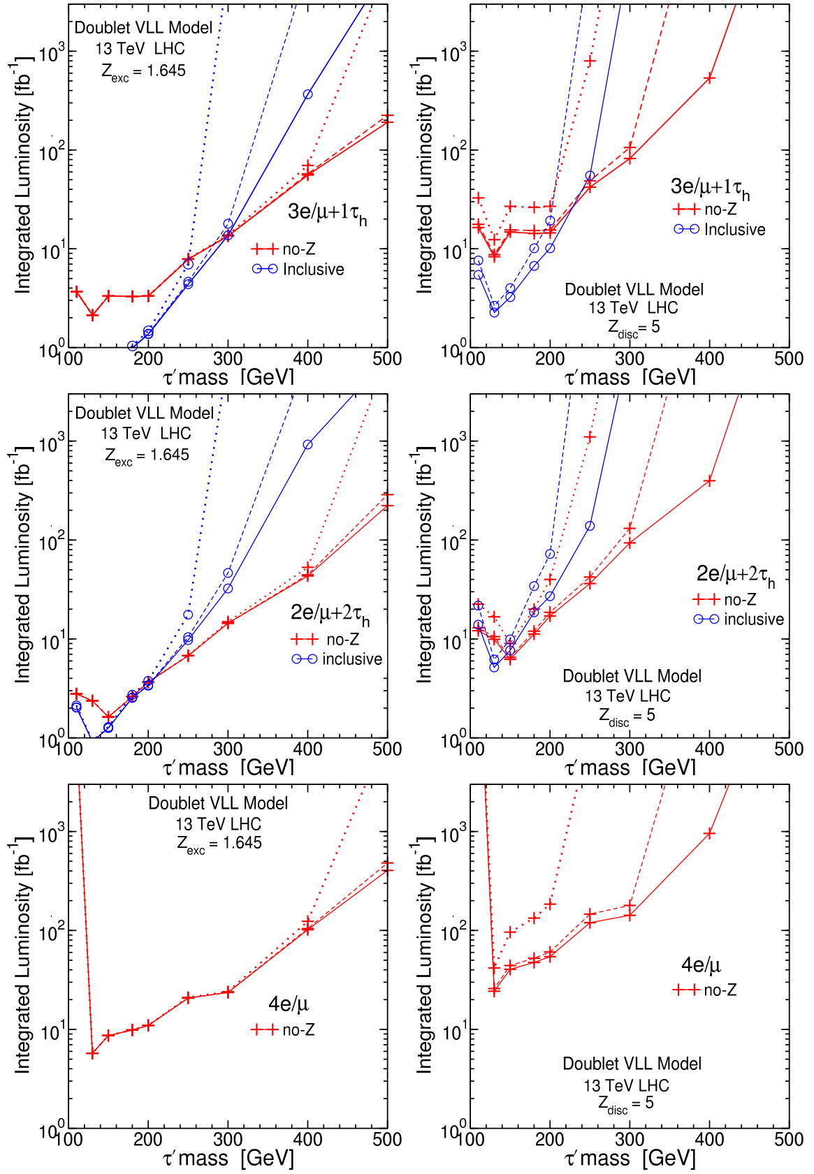
FIG. 8: Integrated luminosity needed for a median expected significance Z_{\text{exc}} \geq 1.645 for exclusion (left) and Z_{\text{disc}} \geq 5 for discovery (right) in \geq 3e/\mu + 1\tau_h , \geq 2e/\mu + 2\tau_h , and \geq 4e/\mu channels, for the Doublet VLL model, as a function of M_{\tau'} = M_{\nu'} , at \sqrt{s} = 13 TeV, based on the results of Table 6.2. The different lines correspond to assumed background uncertainties \Delta_b = 0.1b (solid) and \Delta_b = 0.2b (dashed) and \Delta_b = 0.5b (dotted), with blue lines (circle marks) for inclusive and red (plus marks) for no- Z on each figure.
