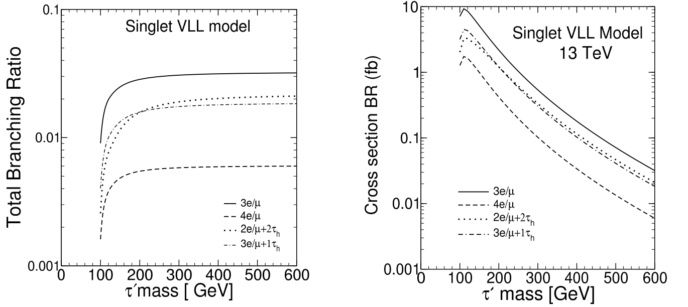
FIG. 10: The total Branching ratio (left) and cross section \times Branching Ratio (right) that contribute to different channels are shown as a function of \tau' mass for singlet VLL model. In the plot at right, the cross sections predicted by the Singlet VLL model at \sqrt{s} = 13 TeV are used.
