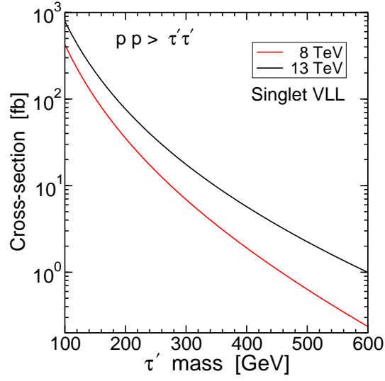
FIG. 1: The production cross section for pp \rightarrow \tau'^+ \tau'^- as a function of the mass M_{\tau'} , for the LHC at \sqrt{s} = 8 and 13 TeV, in the Singlet VLL model, mediated by the interactions in eq. (2.8).
