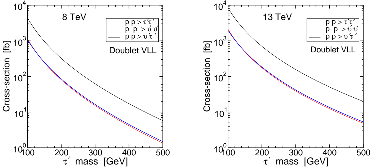
FIG. 2: The production cross sections for, from bottom to top, \nu' \bar{\nu}' and \tau'^+ \tau'^- and the combined cross-section for \nu' \tau'^+ and \bar{\nu}' \tau'^- , as a function of the common mass M_{\tau'} = M_{\nu'} , for the LHC at \sqrt{s} = 8 (left panel) and 13 TeV (right panel), in the Doublet VLL model, mediated by the interactions in eq. (2.9).
