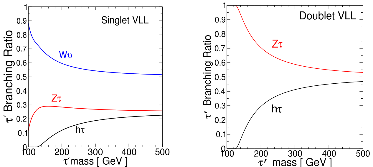
FIG. 3: The branching ratios for \tau' \rightarrow W\nu and Z\tau and h\tau , as a function of M_{\tau'} , for the Singlet VLL model (left panel) and the Doublet VLL model (right panel).
