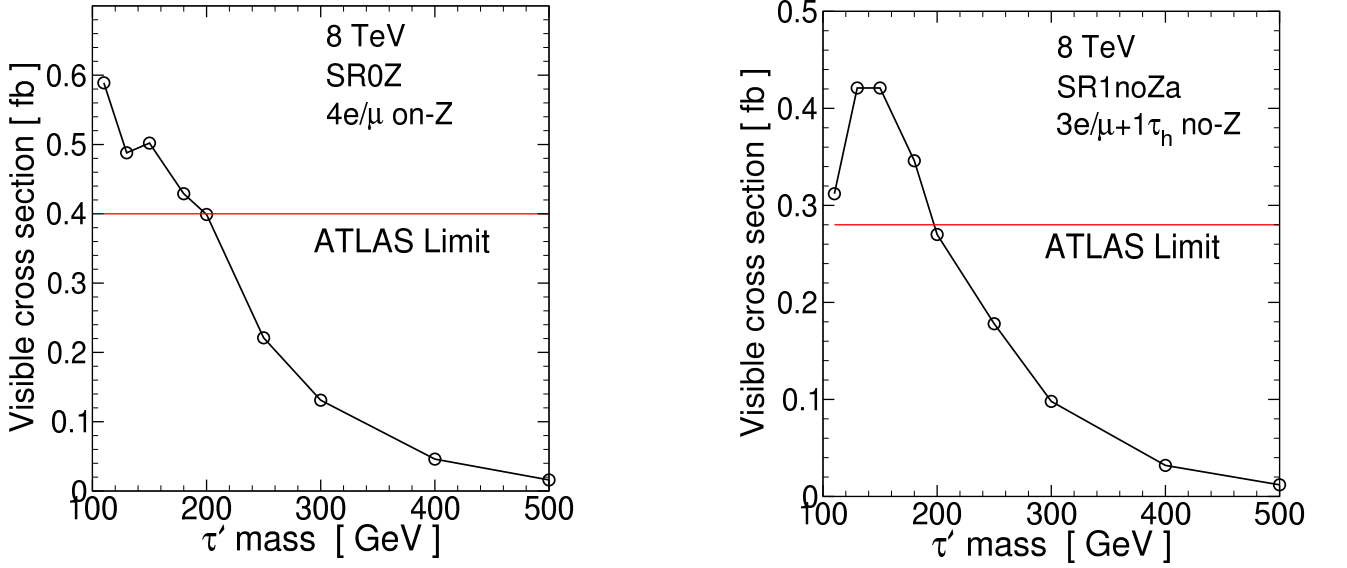
FIG. 5: Total visible cross sections \sigma_v , for the Doublet VLL model, that pass selections \geq 4e/\mu on- Z or SR0Z (left), and 3e/\mu + \geq 1\tau_h no- Z or SR1noZa (right). The results are shown as a function of M_{\tau'} = M_{\nu'} , at \sqrt{s} = 8 TeV, and correspond to entries in Tables 4.3 and 4.4. Also, the ATLAS limits at \sqrt{s} = 8 TeV and \int L dt = 20.3 \text{ fb}^{-1} from ref. [65] are represented by the horizontal red lines.
