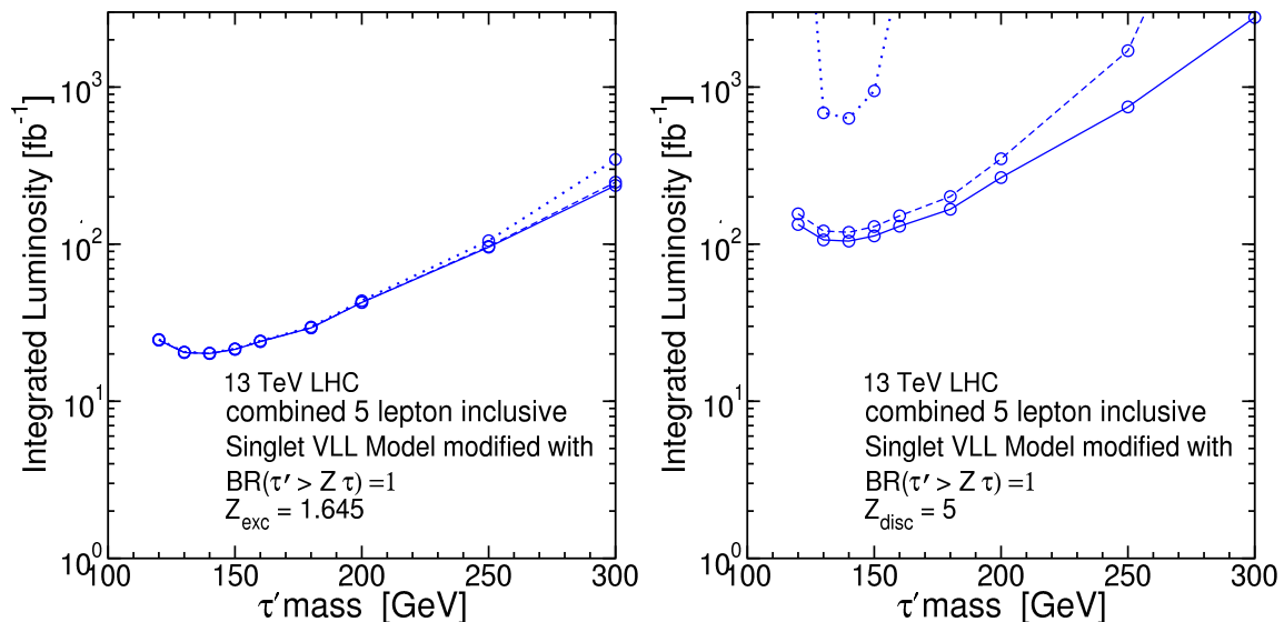
FIG. 16: Integrated luminosities needed for Z_{\text{exc}} = 1.645 (95% CL) exclusion (left) or Z_{\text{disc}} = 5 discovery (right) in the combined 5-lepton inclusive channel, for the modified Singlet VLL model with \text{BR}(\tau' \rightarrow Z\tau) = 1 , as a function of M_{\tau'} , at \sqrt{s} = 13 TeV, based on the results from Table 6.8. The different lines in each plot correspond to assumed background uncertainties \Delta_b = 0.1b (solid), \Delta_b = 0.2b (dashed), and \Delta_b = 0.5b (dotted).
