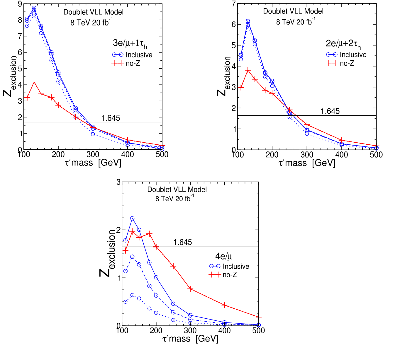
FIG. 7: Median expected significances for exclusion at \int L dt = 20 \text{ fb}^{-1} in \geq 3e/\mu + 1\tau_h (top left), \geq 2e/\mu + 2\tau_h (top right), and \geq 4e/\mu (bottom left) channels, for the Doublet VLL model, as a function of M_{\tau'} = M_{\nu'} , at \sqrt{s} = 8 \text{ TeV} , based on the results of Table 5.2. The different lines in each plot correspond to difference background variances, \Delta_b = 0.1b (solid) and \Delta_b = 0.2b (dashed) and \Delta_b = 0.5b (dotted), with blue lines (circle marks) for inclusive and red (plus marks) for no- Z on each figure. The horizontal black lines are Z_{exc}=1.645 for 95% CL.
