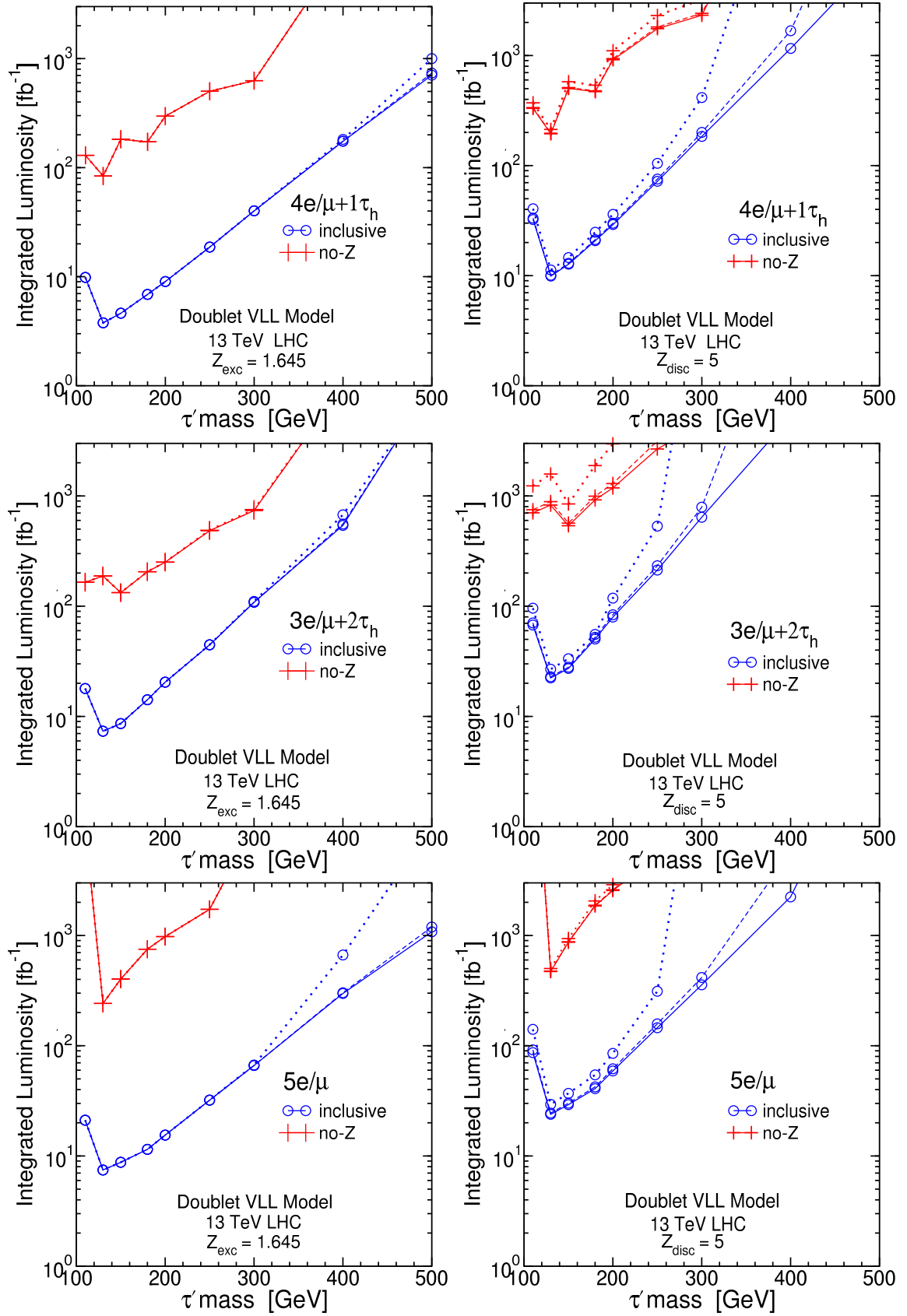
FIG. 9: Integrated luminosity needed for a median expected significance Z_{\text{exc}} \geq 1.645 for 95% CL exclusion (left) and Z_{\text{disc}} \geq 5 for discovery (right) in \geq 4e/\mu + 1\tau_h , \geq 3e/\mu + 2\tau_h , and \geq 5e/\mu channels, for the Doublet VLL model, as a function of M_{\tau'} = M_{\nu'} , at \sqrt{s} = 13 TeV, based on the results of Table 6.4. In the figures different lines correspond to \Delta_b = 0.1\text{b} (solid) and \Delta_b = 0.2\text{b} (dashed) and \Delta_b = 0.5\text{b} (dotted), with blue lines (circle marks) for inclusive, red (plus marks) for no-Z on each figure.
