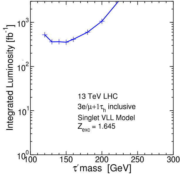
FIG. 12: Integrated luminosity needed for a median expected Z_{\text{exc}} \geq 1.645 (95% CL) exclusion in the inclusive \geq 3e/\mu + 1\tau_h channel, for the Singlet VLL model, as a function of M_{\tau'} , at \sqrt{s} = 13 TeV, based on the results of Table 6.5. The line with plus symbols represents the required luminosity in the most optimistic case of no uncertainty in the background cross-section ( \Delta_b = 0 ). We do not find any prospects for exclusion if the fractional uncertainty in the background is 10% or higher.
