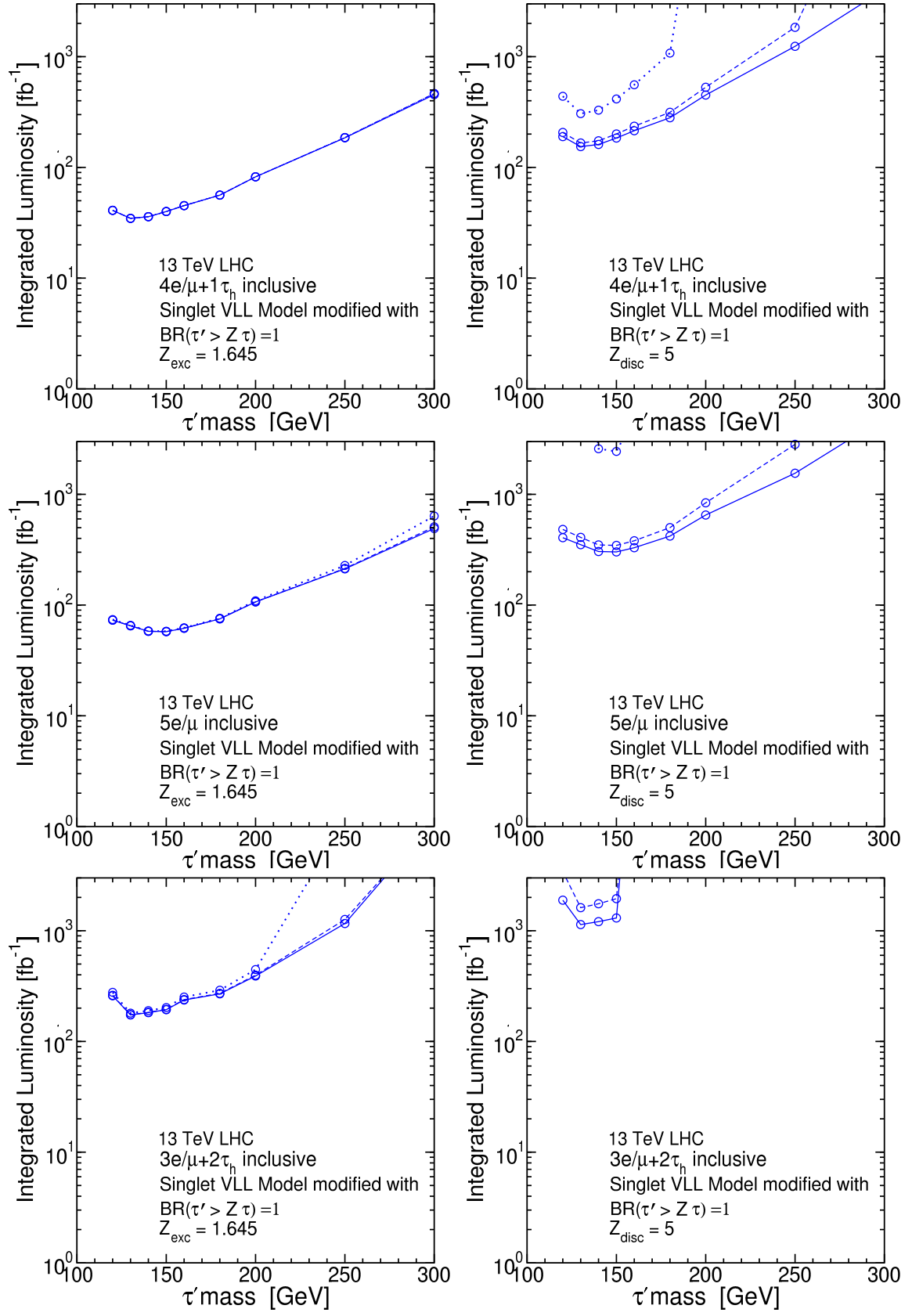
FIG. 15: Integrated luminosities needed for Z_{\text{exc}} = 1.645 (95% CL) exclusion (left) or Z_{\text{disc}} = 5 discovery (right), in the \geq 4e/\mu + 1\tau_h and \geq 5e/\mu and \geq 3e/\mu + 2\tau_h inclusive channels (from top to bottom), for the Singlet VLL model with \text{BR}(\tau' \rightarrow Z\tau)=1 , as a function of M_{\tau'} , at \sqrt{s} = 13 TeV, based on the results from Table 6.8. The different lines in each plot correspond to assumed background uncertainties \Delta_b = 0.1b (solid), \Delta_b = 0.2b (dashed), and \Delta_b = 0.5b (dotted).
