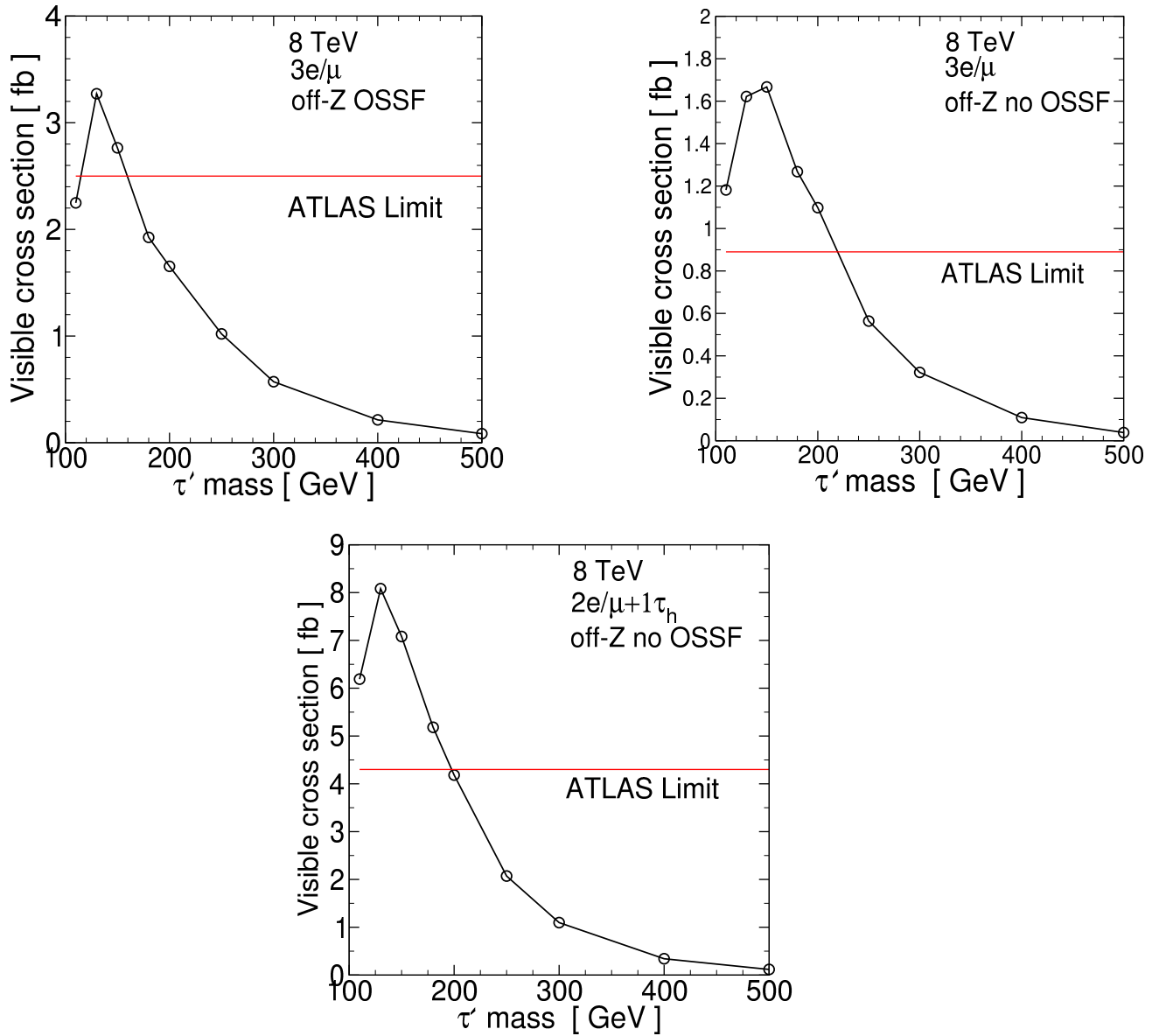
FIG. 4: Total visible cross sections \sigma_v , for the Doublet VLL model, that pass selections: \geq 3e/\mu off- Z OSSF (top left), \geq 3e/\mu off- Z no-OSSF (top right), and 2e/\mu + \geq 1\tau_h off- Z no-OSSF (bottom left). The results are given as functions of M_{\tau'} = M_{\nu'} , at \sqrt{s} = 8 TeV, and are as given in Tables 4.1 and 4.2. For comparison, the ATLAS limits at \sqrt{s} = 8 TeV and \int L dt = 20.3 fb ^{-1} from ref. [64] are represented by the horizontal red lines.
