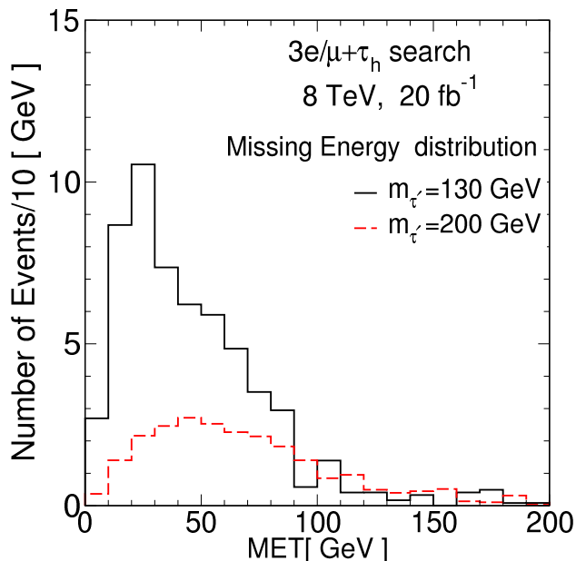
FIG. 6: The expected E_T^{\text{miss}} distribution at \sqrt{s} = 8 TeV in the \geq 3e/\mu + 1\tau_h channel after inclusive event selection for the Doublet VLL model with M_{\tau'} = 130 and 200 GeV. The distributions are normalized according to 20 \text{ fb}^{-1} of integrated luminosity.
