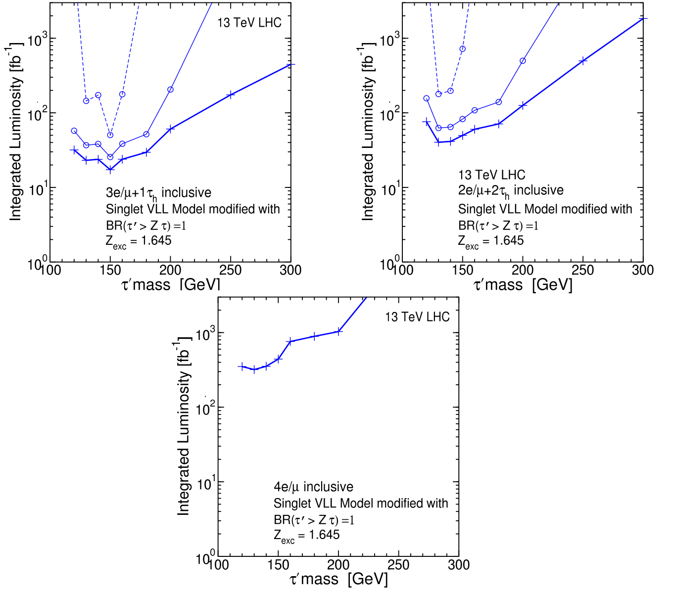
FIG. 13: Integrated luminosities needed for Z_{\text{exc}} = 1.645 (95% CL) exclusion, in the inclusive \geq 3e/\mu + 1\tau_h and \geq 2e/\mu + 2\tau_h and \geq 4e/\mu channels, for the modified Singlet VLL model with \text{BR}(\tau' \rightarrow Z\tau) = 1 , as a function of M_{\tau'} , at \sqrt{s} = 13 TeV, based on the results from Table 6.6. The different lines in each plot correspond to assumed background uncertainties \Delta_b = 0 (thicker solid, with + signs), \Delta_b = 0.1b (solid, with circles) and \Delta_b = 0.2b (dashed, with circles).
