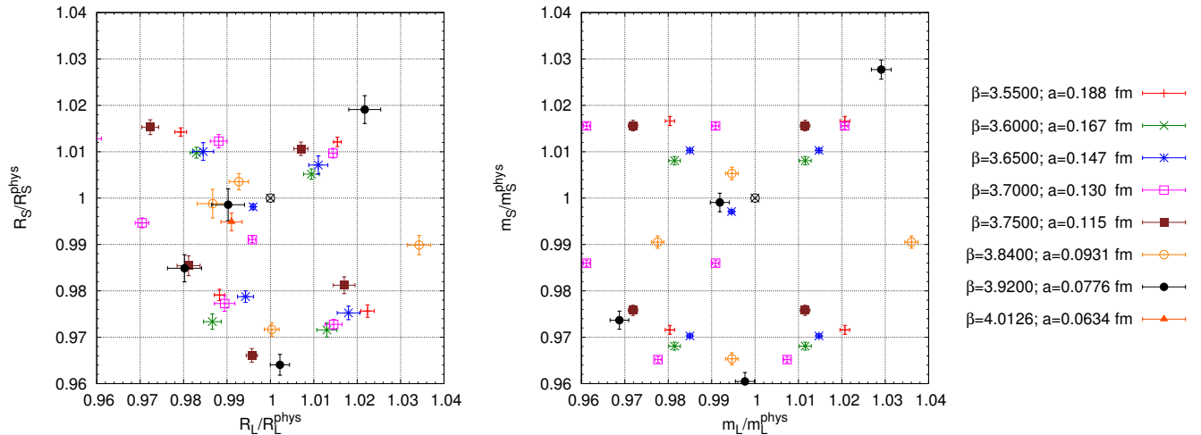
FIG. 1. Summary of our large volume zero temperature runs. The left panel shows the combinations in Eq. (44) where R_S/R_S^{\text{phys}} = 1 and R_L/R_L^{\text{phys}} = 1 define the physical point. We determine the physical bare quark masses by interpolating the bare parameters to precisely restore the R_S and R_L ratios (see Ref. [77] for details). The right panel shows the bare parameters rescaled by the interpolated quark mass. The errors on the rescaled run parameters come solely from the errors of the interpolation.
