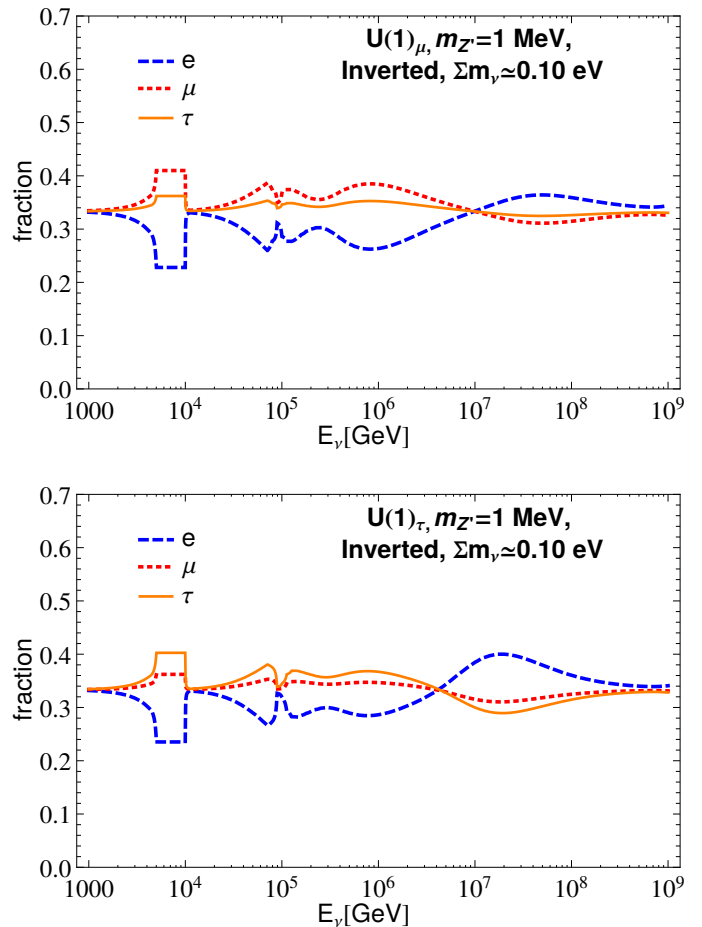
FIG. 4. The fractions of neutrinos of each flavor predicted for a Z' associated with the U(1)_\mu (upper frame) and U(1)_\tau (lower frame) gauge groups. Results are shown for the case of an inverted hierarchy, \sum m_\nu \approx 0.10 eV, and m_{Z'} = 1 MeV.
