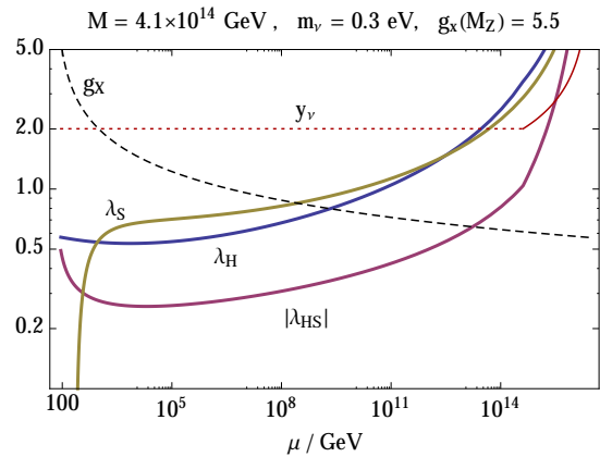
FIG. 4: The RG evolution for the quartic couplings in the communicated CW setup. Choosing the active neutrino mass and Majorana mass, determines the compositeness scale, where the quartics are given values such that \lambda_H = |\lambda_{HS}| = \lambda_S \approx y_\nu^2 at this scale. The final assumption is that g_x(m_Z) = 5.5 , which determines the IR behavior and symmetry breaking pattern. The evolution shown above yields v \simeq 174 GeV and m_H \simeq 126 GeV.
