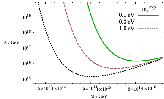
FIG. 2: Numerical results displaying the relation between the Majorana mass and the scale associated with the Landau pole for the neutrino HY coupling for different values of the neutrino mass.
