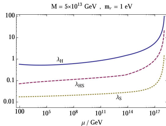
FIG. 3: The RG evolution for the quartic couplings for a specific choice of initial conditions at the UV scale. The IR phenomenology features a large quartic for the Higgs, while the effective coupling leads to a light Higgs mass m_H \sim 130 GeV.
