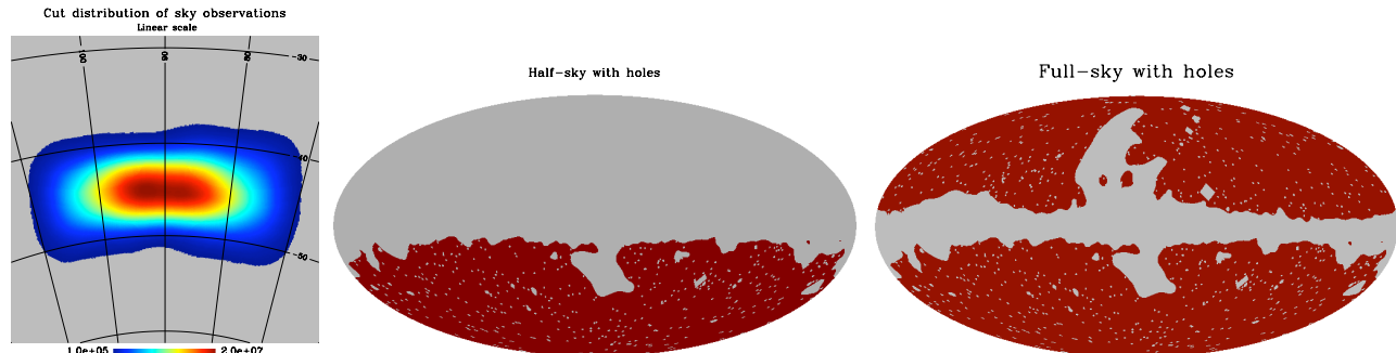
FIG. 4. Left Panel : A potential noise distribution (number of hits per pixel) for small-scale experiments covering \sim 1\% of the sky. The noisiest pixels have been discarded and the noise distribution ranges from 10^5 to 10^7 . Middle panel : Portion of the sky kept for estimating the B -mode angular power spectra for a possible array of ground-based telescopes. It roughly covers 36% of the sky (Note that for this analysis the choice of galactic or ecliptic south hemisphere is equivalent, see text for more information). Right panel : Portion of the sky kept for estimating the B -mode angular power spectra for a possible satellite mission, roughly covering 71% of the sky.
