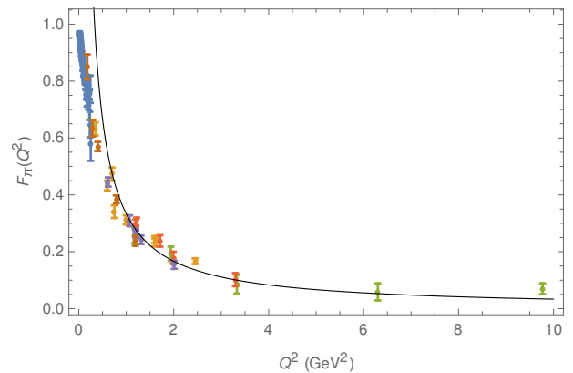
FIG. 4. (Color online) The data [32–40] for the pion form factor shown against the simple model F_\pi(Q^2) = \frac{1}{3}Q^{-2} (solid line).
