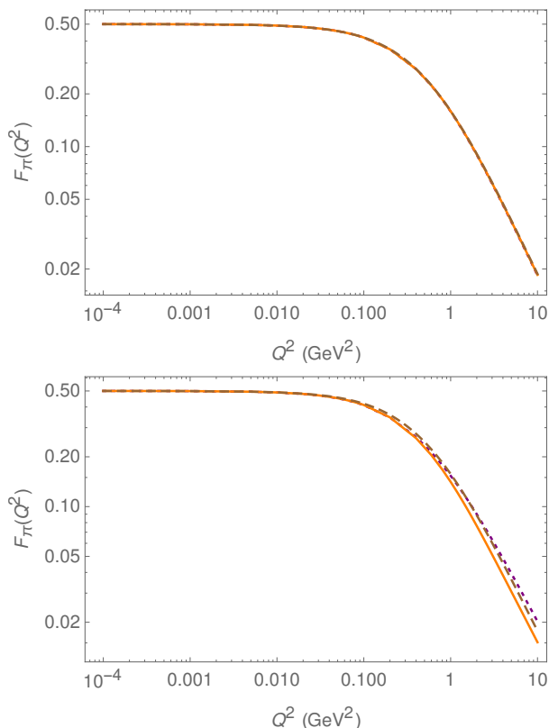
FIG. 6. (Color online) The pion form factor contributions calculated for \alpha = 3 (dashed, brown), \alpha = 1 (solid, orange), and \alpha = 0.5 (dotted, purple), with \mu = 0.42 GeV and with running quark masses. The top panel shows the spectator and the bottom panel shows the active pole contributions.
