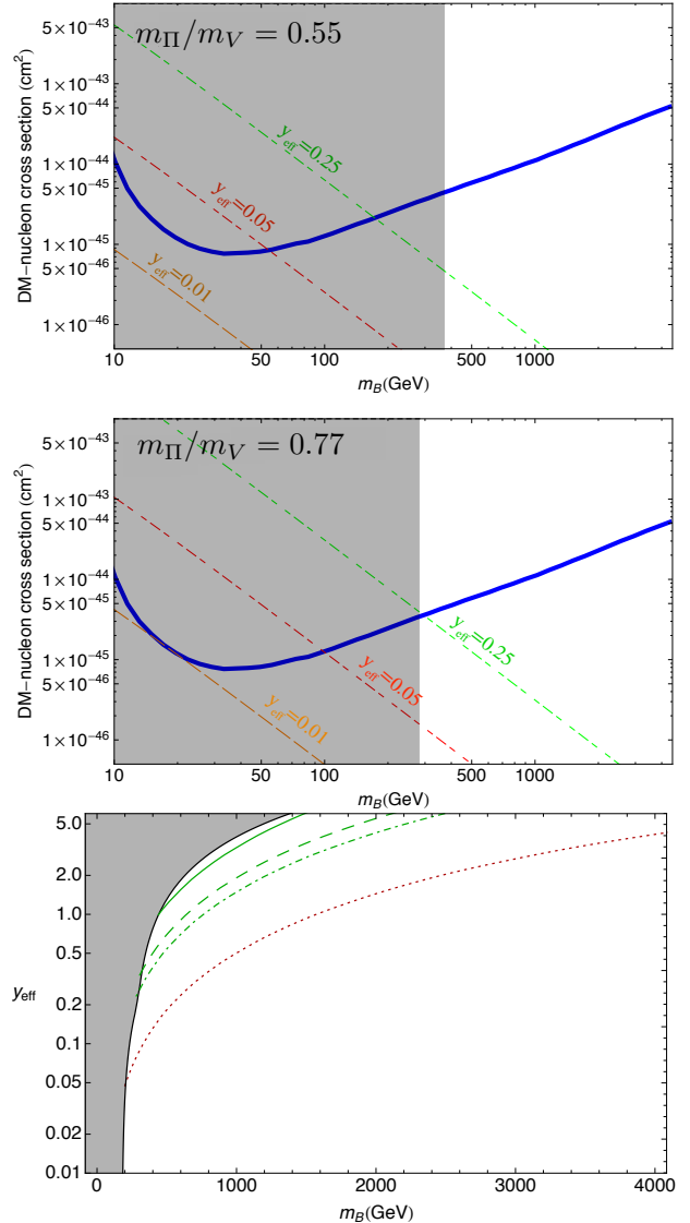
FIG. 3. Same as Fig. 2 but for the Quadratic Case of the model. In this case, y_{\text{eff}} \approx ym_B/\sqrt{M_1\Delta} .
