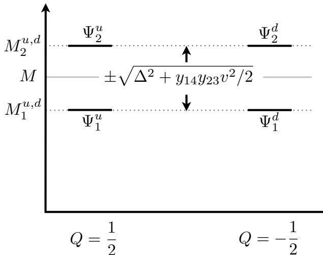
FIG. 1. Illustration of the fermion mass spectra considered in the paper. Four Dirac fermions ( \Psi_1^u , \Psi_1^d , \Psi_2^u , \Psi_2^d ) have masses ( M_1^u , M_1^d , M_2^u , M_2^d ). The u ( d ) fermions have electric charge Q = +1/2 ( Q = -1/2 ); we assume an exact custodial SU(2) global symmetry that ensures each Q = +1/2 fermion is accompanied by a Q = -1/2 fermion with equal mass as shown in the figure. If \Delta \ll \sqrt{y_{14}y_{23}}v ( \Delta \gg \sqrt{y_{14}y_{23}}v ) the mass splitting is dominated by electroweak breaking (preserving) masses that we call the Linear (Quadratic) Case. See the text for details.
