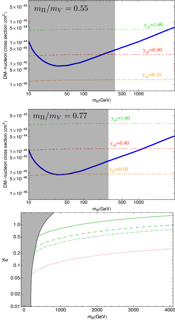
FIG. 2. Constraints on the stealth dark matter model in the Linear Case of the model. The top and middle figures show the predicted values for the smallest and largest fermion mass explored in our simulations (corresponding to the pseudoscalar to vector mass ratio m_{\Pi}/m_V = 0.55, 0.77 ) as well as LUX bounds. Various y_{\text{eff}} values are plotted on the figure, where y_{\text{eff}} \approx ym_B/M_1 in this case. The dark grey region is excluded by the LEP constraints on charged dark mesons. The bottom figure displays the maximum y_{\text{eff}} allowed for a given dark matter mass. Each of the green curves represents a different fermion mass in the lattice calculation, m_{\Pi}/m_V = 0.55, 0.7, 0.77 from top to bottom, and the bottom red curve is the result in the heavy fermion limit.
