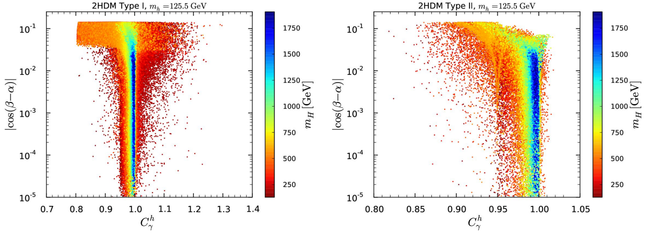
Figure 7: |\cos(\beta-\alpha)| versus C_\gamma^h in Type I (left) and Type II (right) with m_H color code. Points are ordered from low to high m_H .
