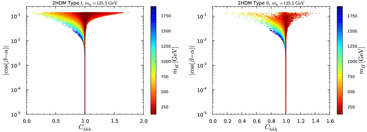
Figure 8: |\cos(\beta-\alpha)| versus the reduced triple Higgs coupling C_{hhh} in Type I (left) and Type II (right) with m_H color code. Points are ordered from high to low m_H values.
