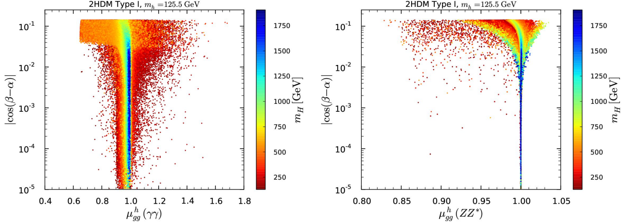
Figure 10: Signal strengths in Type I for the 125.5 GeV state, for gg \rightarrow h \rightarrow \gamma\gamma (left) and gg \rightarrow h \rightarrow ZZ^* (right) with m_H color code. Points are ordered from low to high m_H values. Points with \mu_{gg}^h(ZZ^*) < 0.92 are ones for which h \rightarrow AA decays are present, so that the total h width is increased, which suppresses this particular channel's rate.
