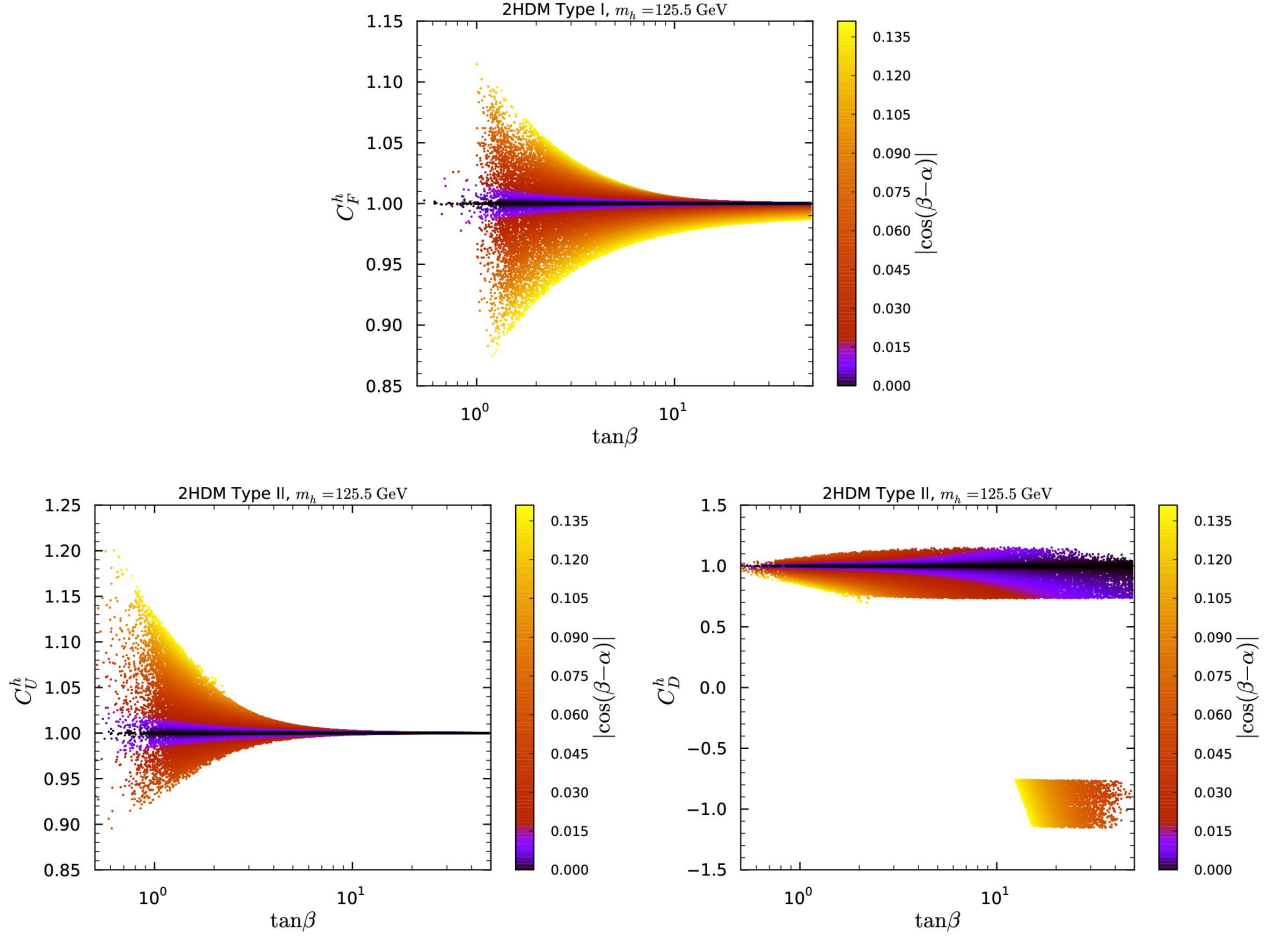
Figure 6: Fermionic couplings versus \tan\beta in Type I (upper panel) and Type II (lower panels) with |\cos(\beta-\alpha)| color code. Points are ordered from high to low |\cos(\beta-\alpha)| .
