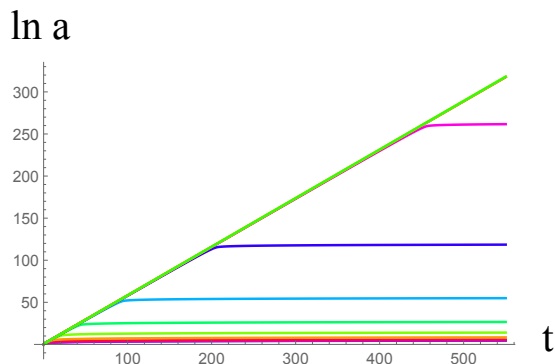
FIG. 14. The log of a scale factor is plotted, as a function of time. The models with smallest, in our examples, initial values of \varphi < 6 produce less than 50 e-foldings, however, all other cases with \varphi > 6 easily lead to more than 60.
