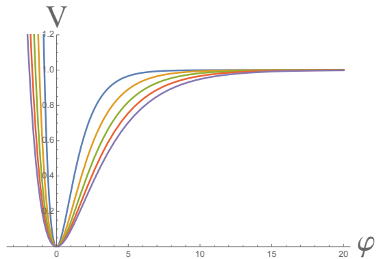
FIG. 3. Potentials of simple E-models V = \left( 1 - e^{-\sqrt{\frac{2}{3\alpha}}\varphi} \right)^2 for \alpha = 1, 2, 3, 4, 5 . It has an inflationary plateau for large positive \varphi and a wall at small negative \varphi .
