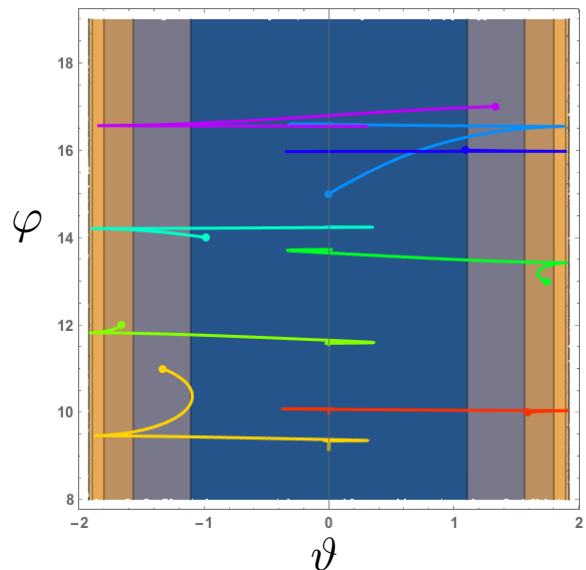
FIG. 15. Evolution of the fields \varphi and \vartheta starting at the Planck energy density. The fields start on the wall with near maximal \vartheta or anywhere between the wall and the bottom of the dS valley with velocities such that the total energy is always E_{kin}^0 + V_0 = 1 . In this process their total energy is decreasing to \sim 10^{-10} when they reach the bottom of the valley.
