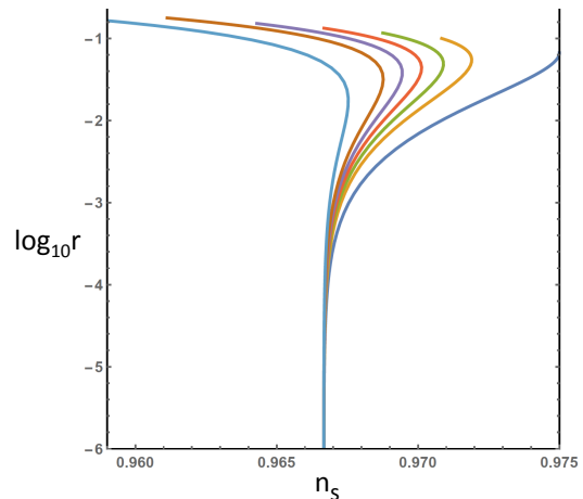
FIG. 4. Here we present the cosmological observables n_s and r for E-models with different monomial potentials V = \left( 1 - e^{-\sqrt{\frac{2}{3\alpha}}\varphi} \right)^{2n} with n = (1/2, 3/4, 7/8, 1, 3/2, 2, 3) starting from the right, increasing to the left, with the line for n = 1 in the middle. The scale in r is logarithmic.
