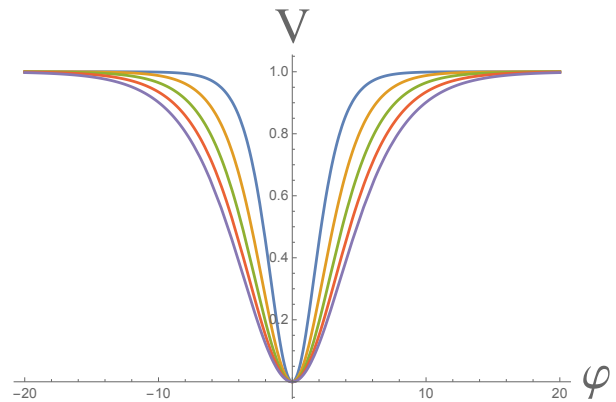
FIG. 1. T-model potential V = \alpha\mu^2 \tanh^{2n} \frac{\varphi}{\sqrt{6\alpha}} for \alpha = 1, \dots, 5 at \text{Im } Z = 0 . It is plotted in units \alpha\mu^2 = 1 . The potential has two symmetric shoulders.
