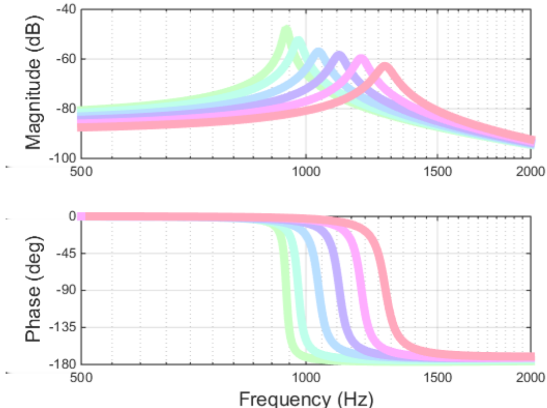
FIG. 7. Stable single-carrier optical springs (no sub-carrier) with modified coating - the first coating layer is 20.5 wavelength thick. See text for details. The six traces otherwise have the same parameters as the best-fit optical springs in figure 4. The magnitude is given in dB meter/Newton.
