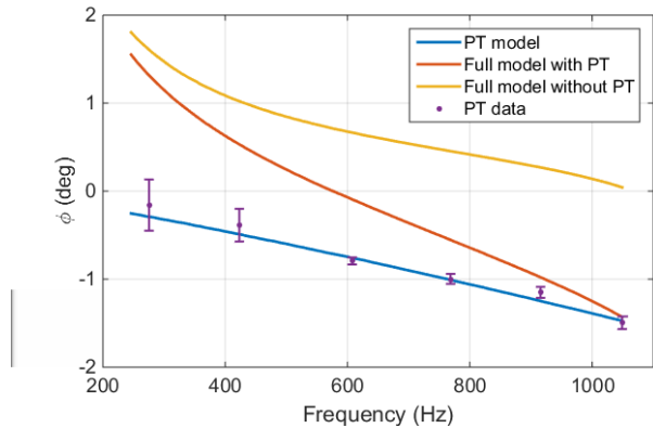
FIG. 6. Feedback phase at the optical spring resonance frequency due to the optical spring and photo-thermal (PT) effect. The measured extra phase is consistent with 2.60 ppm of absorption. The error bars are as small as \pm 0.04^\circ , a remarkable precision for an open loop transfer function phase measurement.
